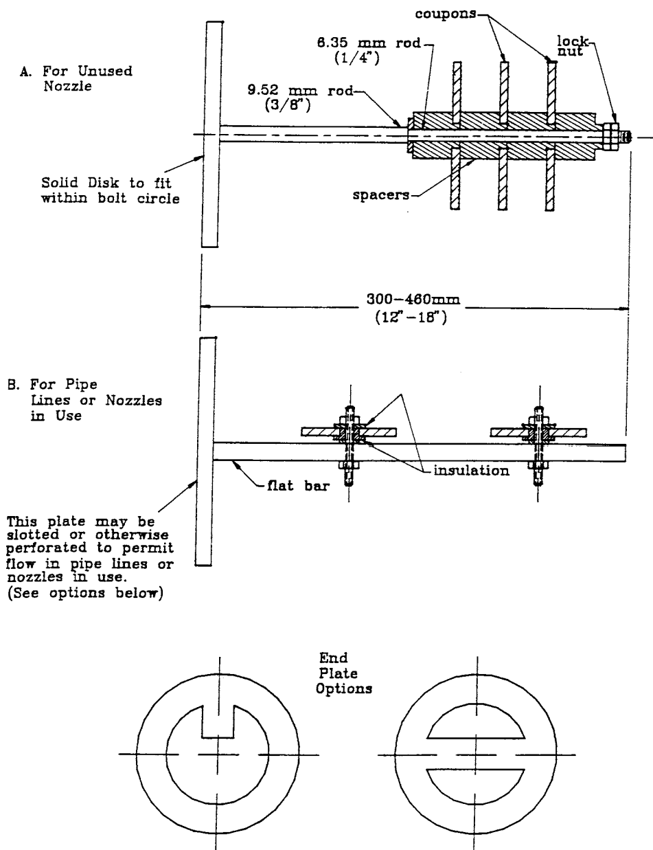
FIG. 3 Pipe Insertion Rack
