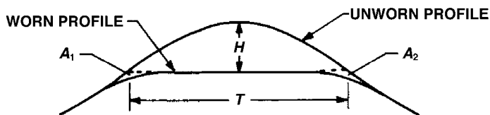
FIG. X1.1 Wear Determination
