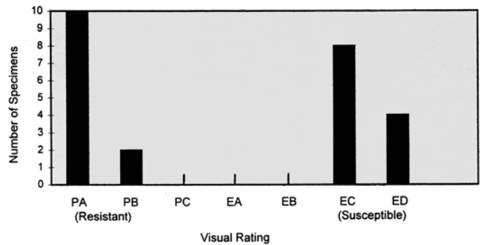
FIG. 3 Histogram of Visual Exfoliation Ratings by Six Laboratories for Two Tempers of 5086 Plate Tested by ASSET (Data in Table 1)
