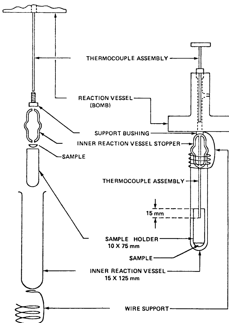
FIG. 2 Sample Holding Assembly
