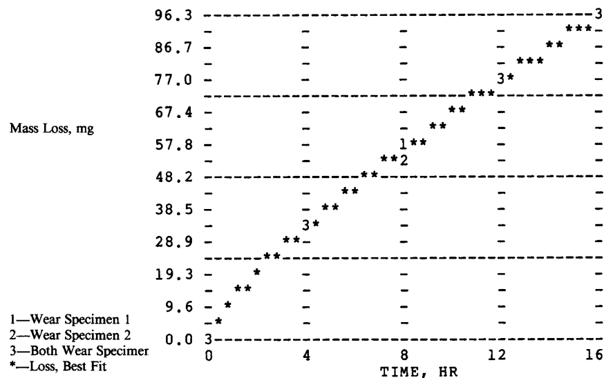
FIG. X1.7 Slurry Abrasion Response (SAR Number) Determination by Miller Number System—Test RS-1
