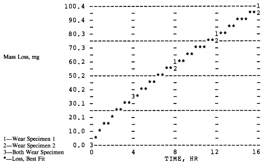
FIG. X1.4 Slurry Abrasivity Determination by Miller Number System—Test RM-1 (Test Method G 75)
