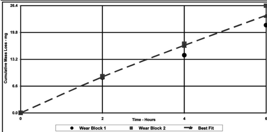
FIG. X1.1 Slurry Abrasivity Determination by Miller Number System (Test Method G 75)
