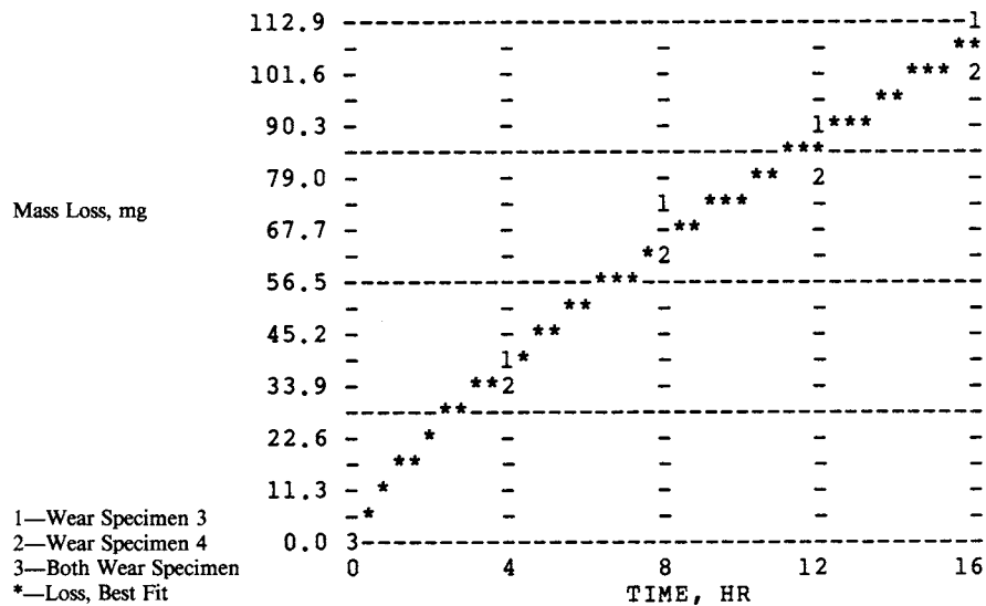
FIG. X1.5 Slurry Abrasivity Determination by Miller Number System—Test RM-2 (Test Method G 75)
