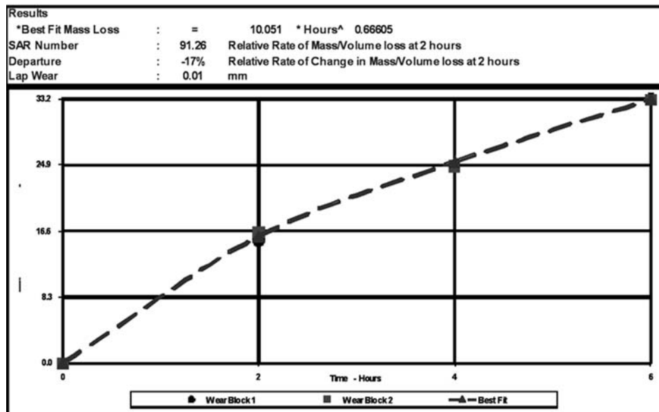
FIG. X1.2 Slurry Abrasion Response (SAR Number) Determination by Miller Number System
