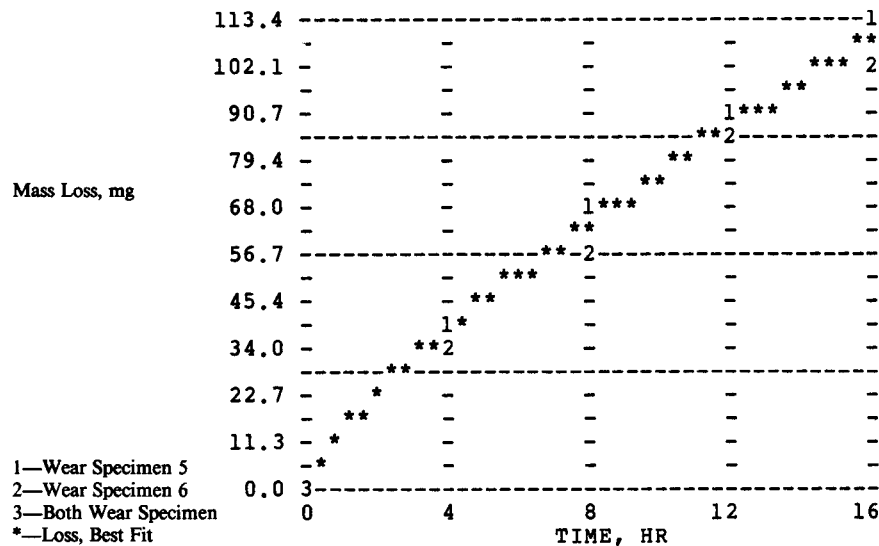
FIG. X1.6 Slurry Abrasivity Determination by Miller Number System—Test RM-3 (Test Method G 75)
