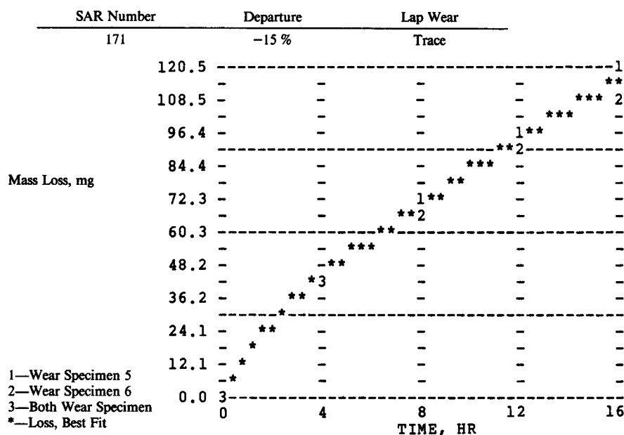
FIG. X1.9 Slurry Abrasion Response (SAR Number) Determination by Miller Number System—Test RS-3
