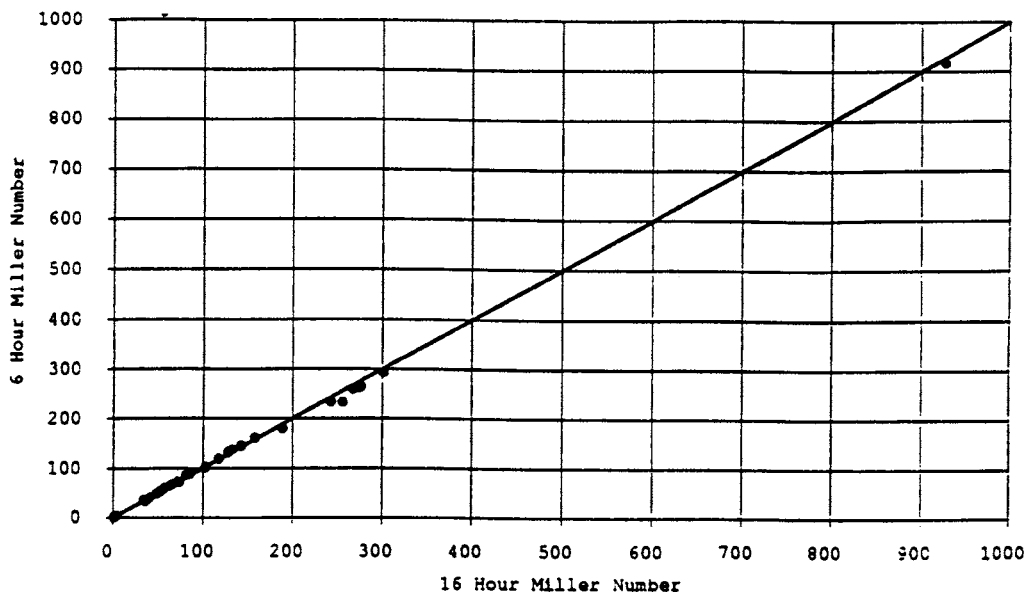
FIG. X1.3 Chart of 16-h Test Versus 6-h Test
