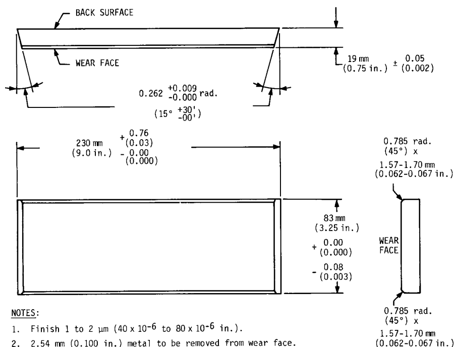
FIG. 2 Example Test Plate Dimensions for Modified Mine and Smelter 100 by 150 mm (4 by 6 in.) Jaw Crusher
