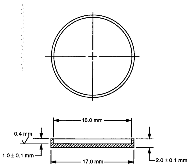
FIG. 8 One-Piece Insert Cup
