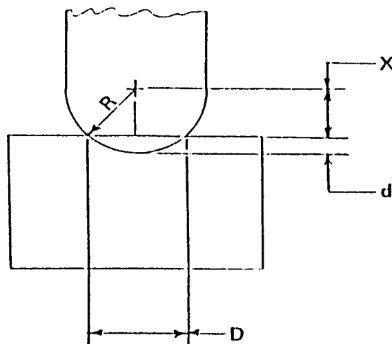
FIG. 15 Determination of the Penetration Depth from the Measured Diameter
