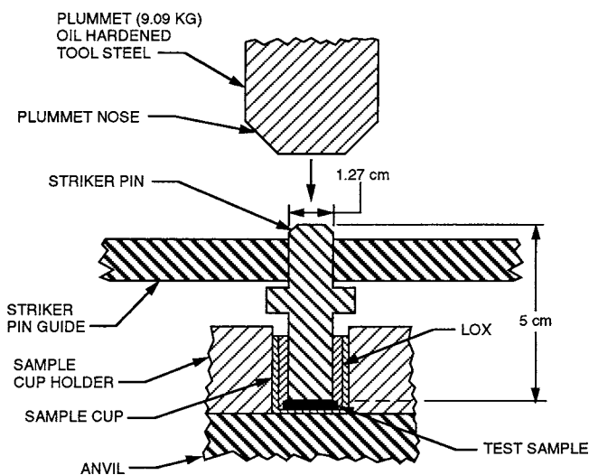
FIG. 12 LOX Impact Tester Sample Cup, Sample Cup Holder, Striker Pin, and Anvil Configuration
