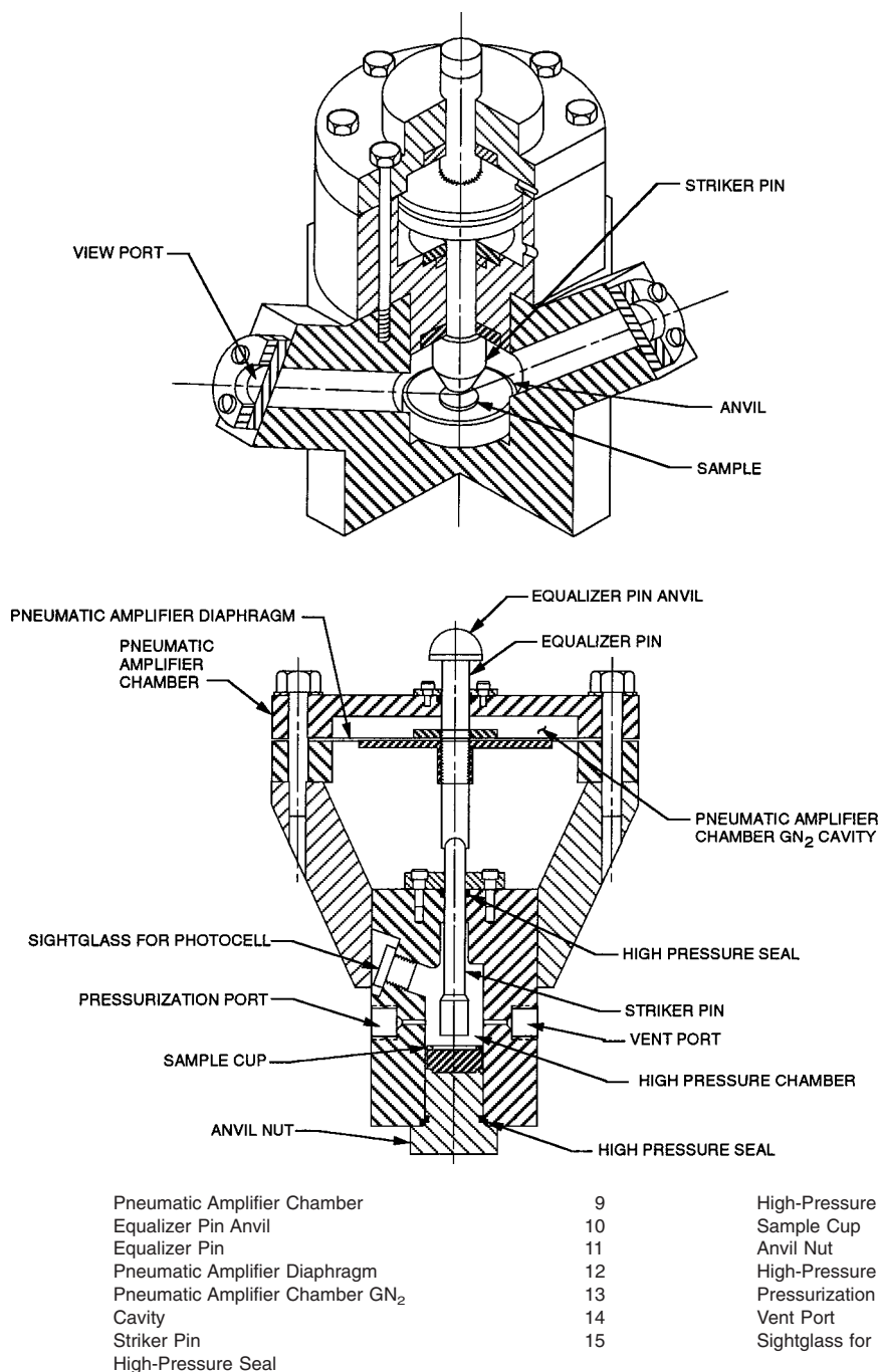
FIG. 2 Two Types of High-Pressure Test Chambers
