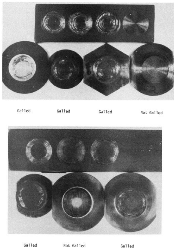
FIG. 4 Test Specimens
