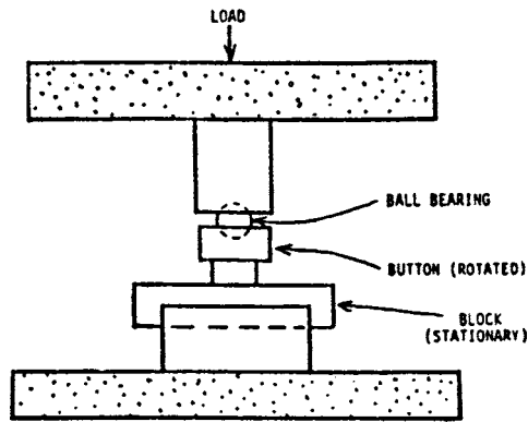
FIG. 2 Schematic Diagram of Galling Test Set-Up
