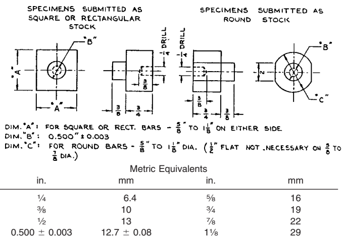
FIG. 1 Typical Button Geometries
