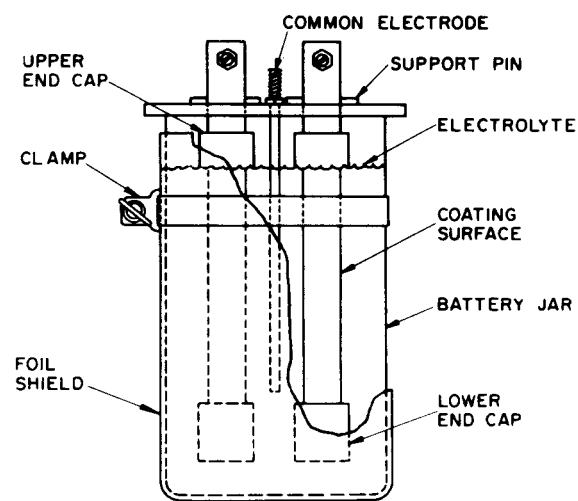
FIG. 1 Typical Test Cell
