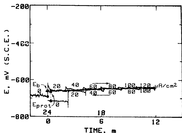
FIG. 2 Cyclic GSCP Curve of 3003 A1 in 3000 ppm NaCl (Taken from Ref 7)
