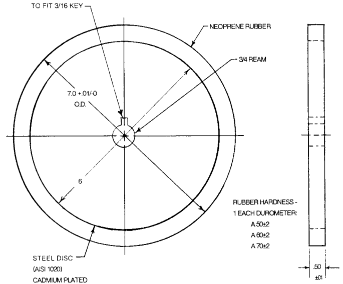
FIG. 2 Rubber Wheel
