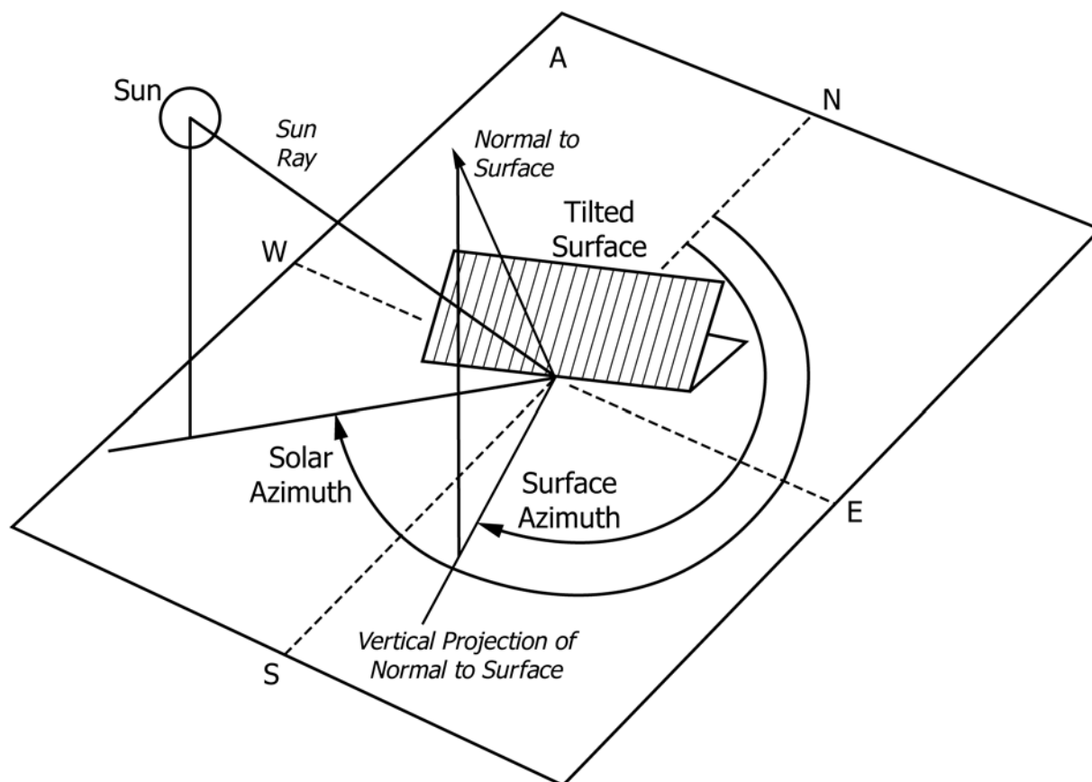
FIG. 1 Solar Azimuth Angle and Surface Azimuth Angle
