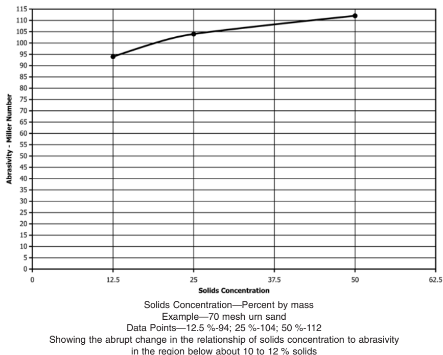
FIG. A1.1 Solids Concentration Versus Abrasivity
