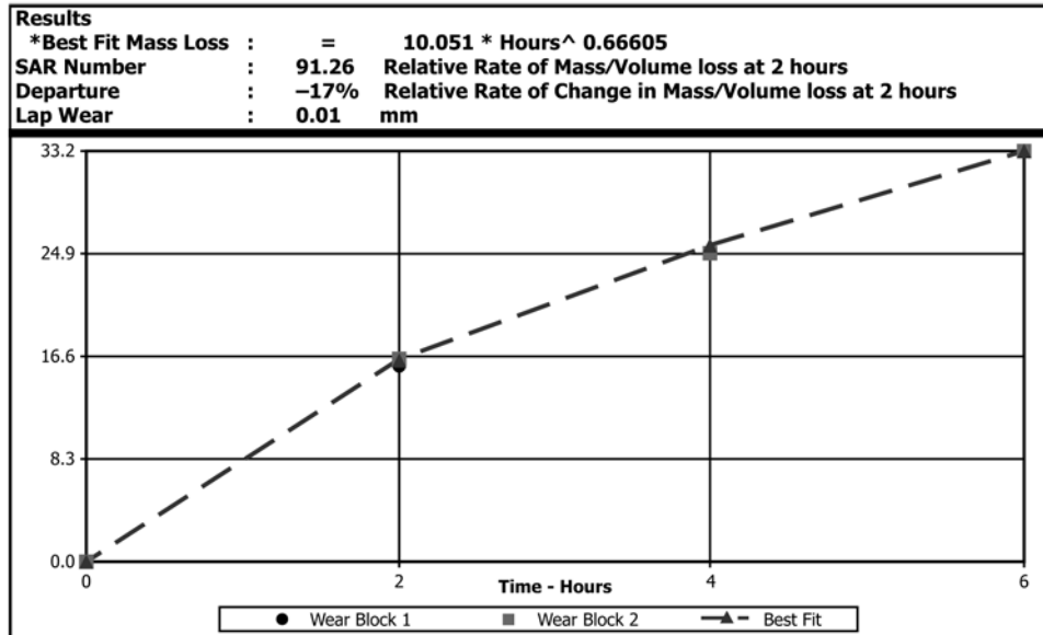
FIG. X1.2 Slurry Abrasion Response (SAR Number) Determination by Miller Number System
