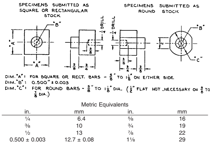
FIG. 1 Typical Button Geometries
