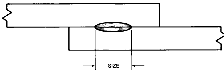
(F) SIZE OF SEAM OR SPOT WELD
