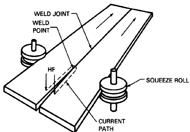
(A) BUTT JOINT MADE BY HIGH-FREQUENCY UPSET WELDING
