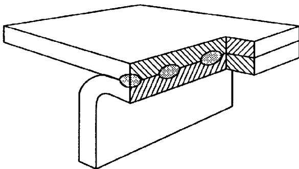
(E) RESISTANCE SPOT WELDS IN A FLANGED CORNER JOINT
