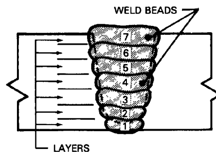
(E) CROSS-SECTIONAL SEQUENCE
