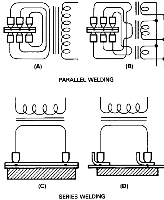
Figure 46 — Typical Arrangements for Multiple Spot Welding
