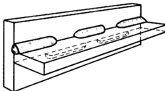
(H) STAGGERED INTERMITTENT FILLET WELD
