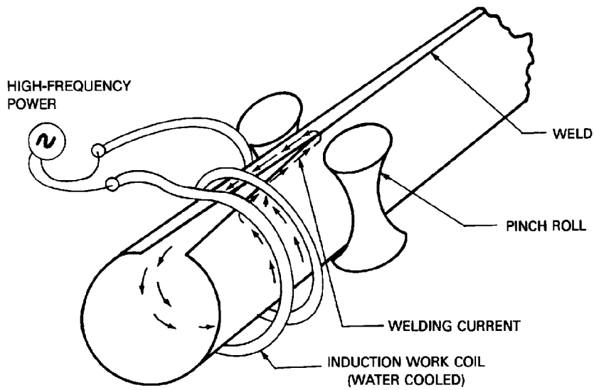
(E) INDUCTION UPSET WELDING OF TUBE
