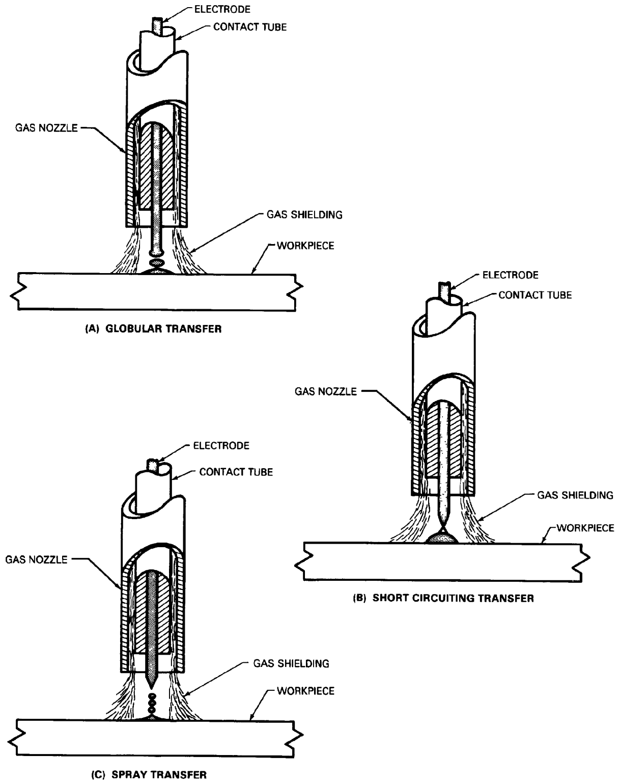
Figure 39 — Metal Transfer in Gas Metal Arc Welding
