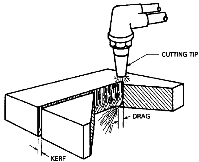
Figure 41 — Oxygen Cutting
