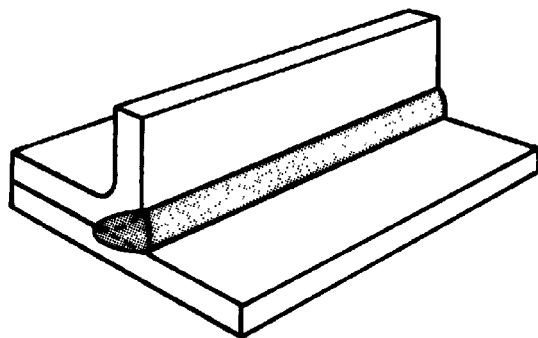
(G) SINGLE-FLARE-BEVEL GROOVE WELD
