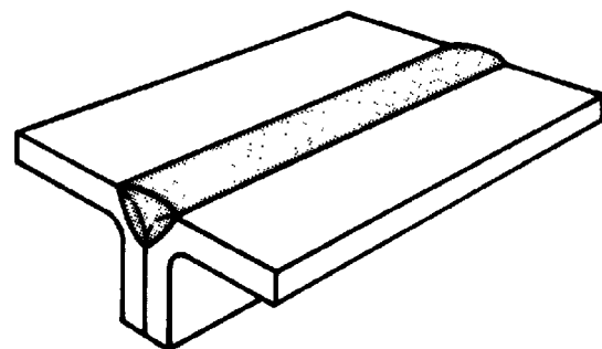
(H) SINGLE-FLARE-V-GROOVE WELD
