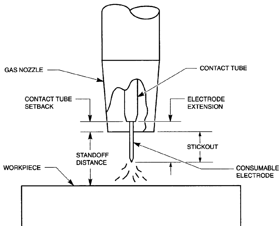
Figure 38 — Gas Metal Arc Welding Gun Nomenclature
