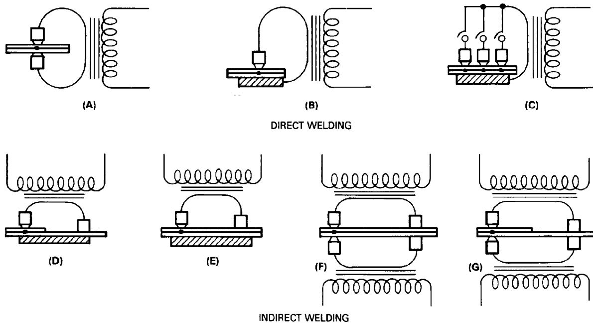
Figure 47 — Typical Arrangements for Single Spot Welds
