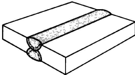
(E) DOUBLE-U-GROOVE WELD
