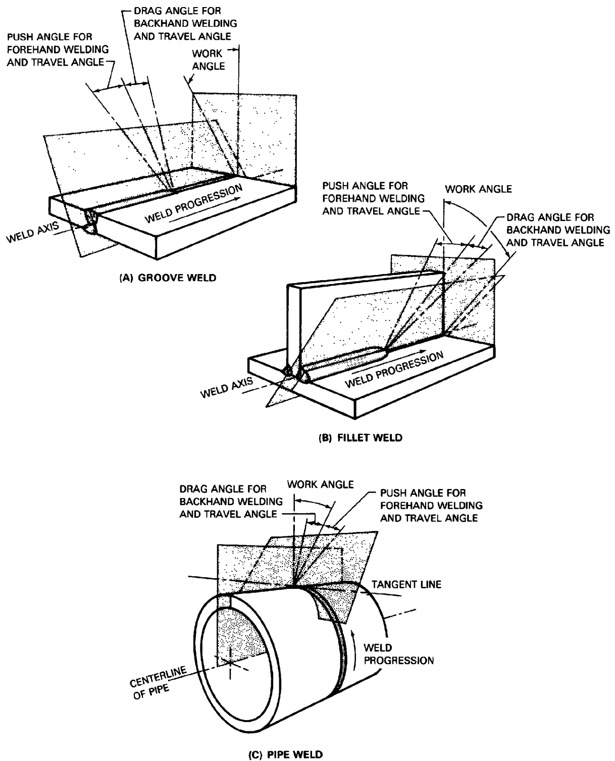
Figure 21 — Position of Electrode, Gun, Torch, Rod, or Beam
