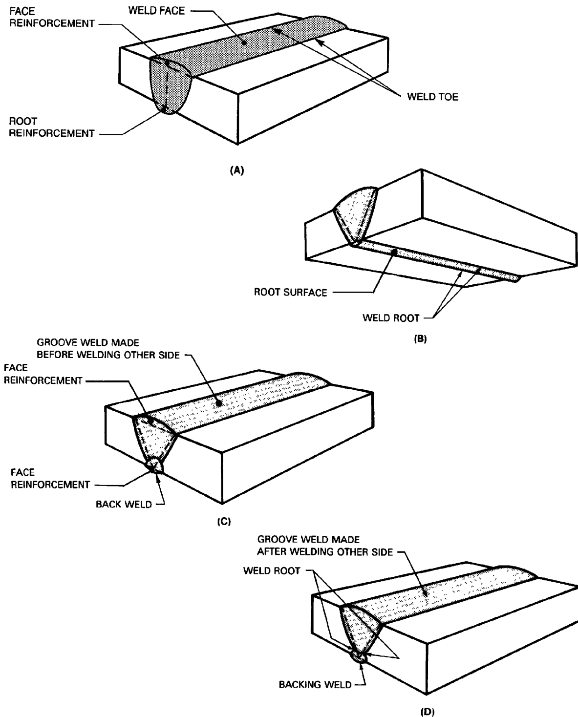
Figure 24 — Parts of a Weld
