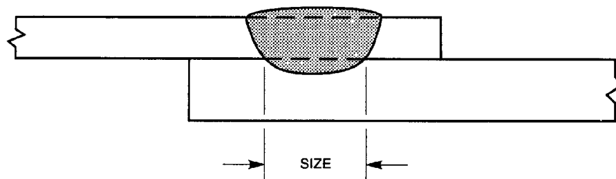
(G) ARC SEAM OR ARC SPOT WELD SIZE
