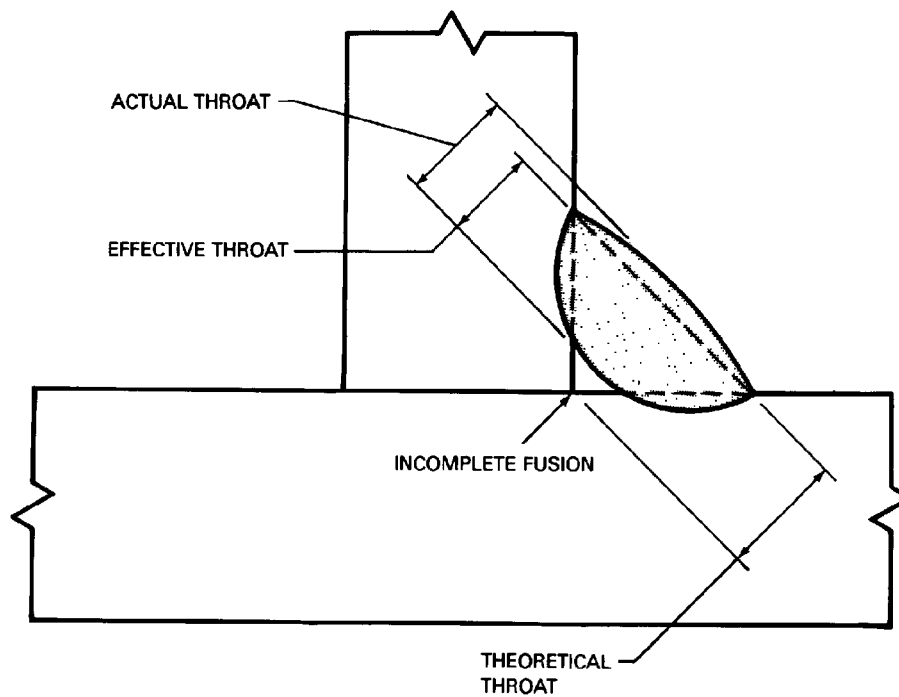
(C) FILLET WELD WITH INCOMPLETE FUSION
