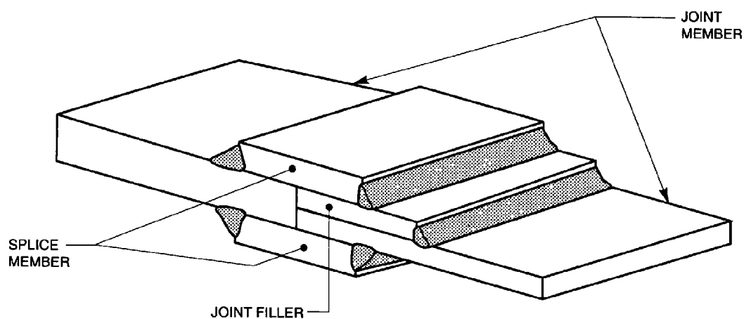
(B) DOUBLE-SPLICED EDGE JOINT WITH JOINT FILLER
