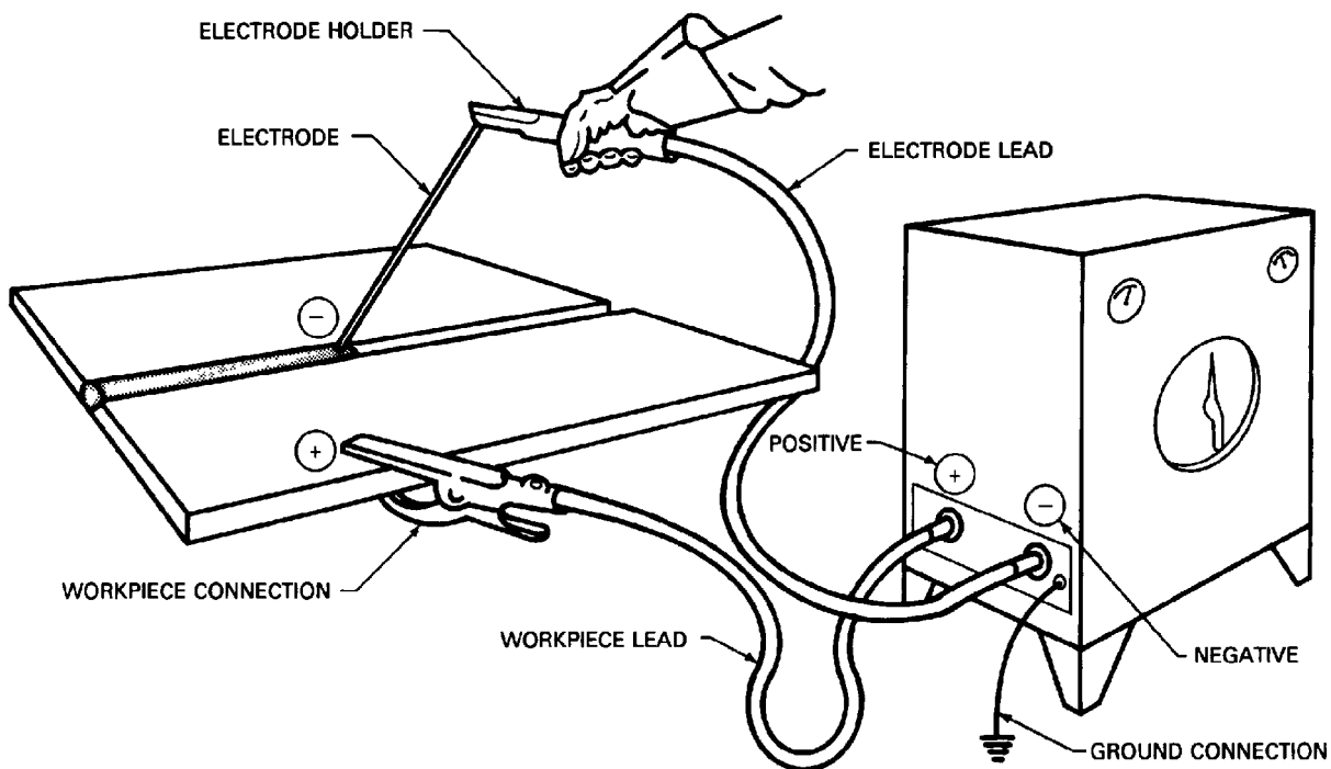
(B) DIRECT CURRENT ELECTRODE NEGATIVE
