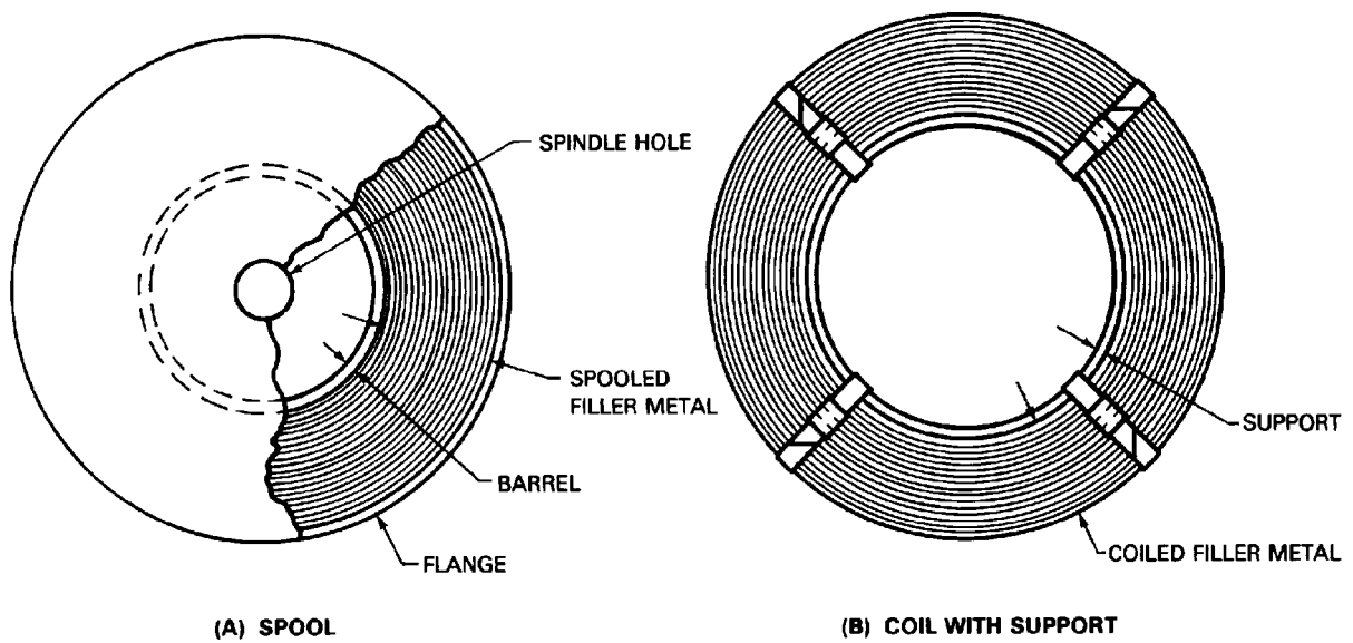
Figure 42 — Filler Metal Packaging
