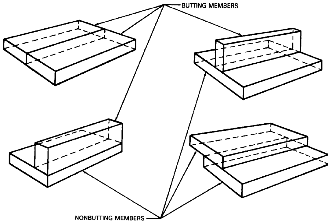
Figure 11 — Butting and Nonbutting Members
