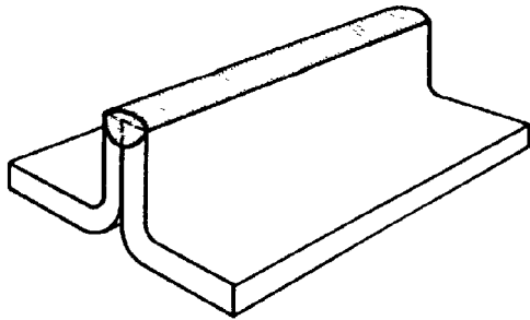
(A) EDGE WELD IN A FLANGED BUTT JOINT
