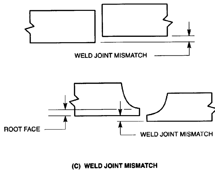
Figure 13 — Edge Weld, Scarf Groove, and Weld Joint Mismatch
