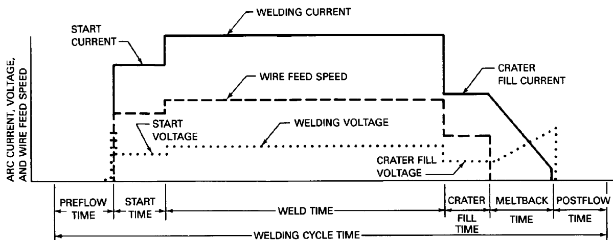
Figure 53 — Typical GMAW, FCAW, and SAW Program for Automatic Welding
