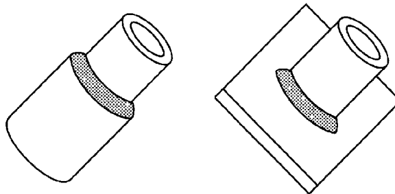
(F) MULTIPLE WELDING TEST POSITION—6F
