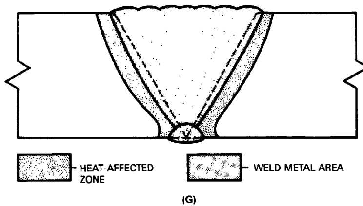
Figure 24 (Continued) — Parts of a Weld
