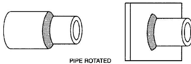
(C) HORIZONTAL WELDING TEST POSITION—2FR
