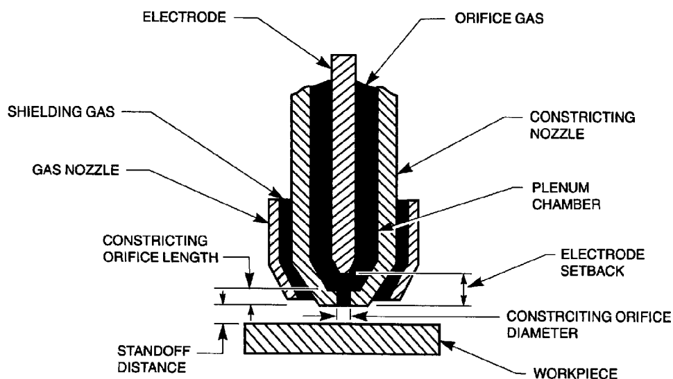
Figure 35 — Plasma Arc Torch Nomenclature
