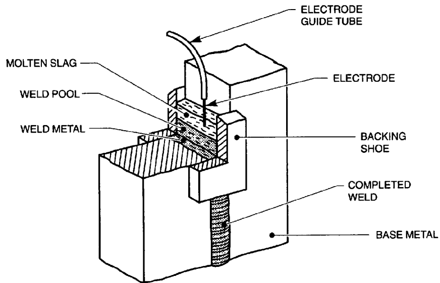
Figure 37 — Typical Arrangement for Electroslag Welding Process Nomenclature
