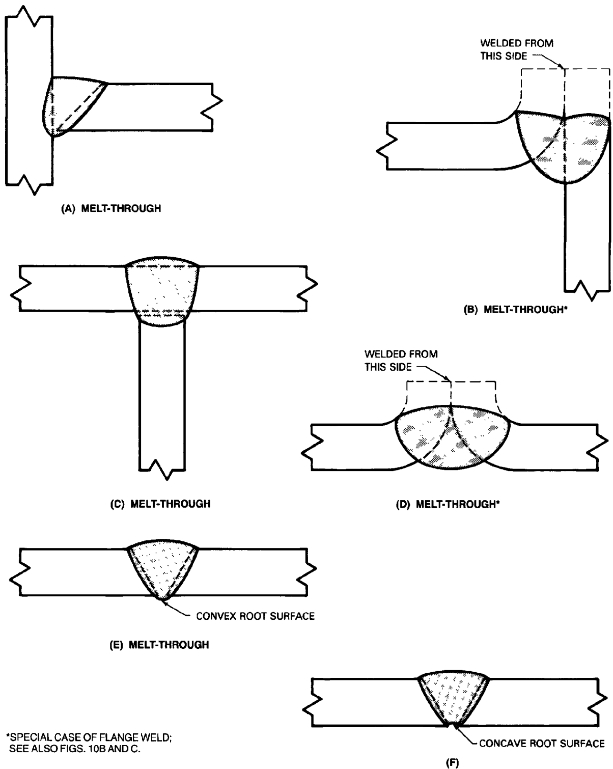
Figure 27 — Melt-Through and Root Surface Profile
