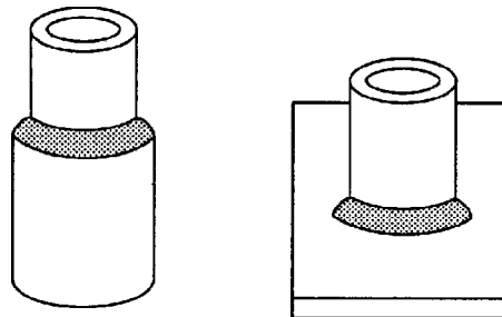
(B) HORIZONTAL WELDING TEST POSITION—2F
