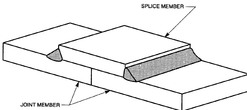
(A) SINGLE-SPLICED BUTT JOINT
