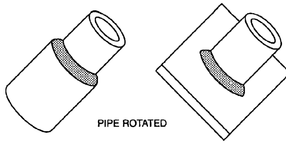
(A) FLAT WELDING TEST POSITION—1F
