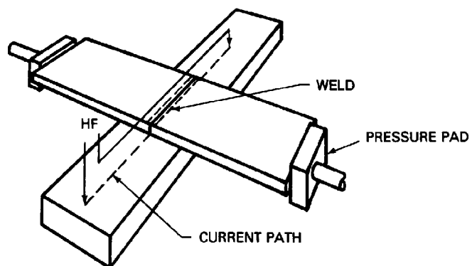
(B) BUTT JOINT MADE BY HIGH-FREQUENCY UPSET WELDING
