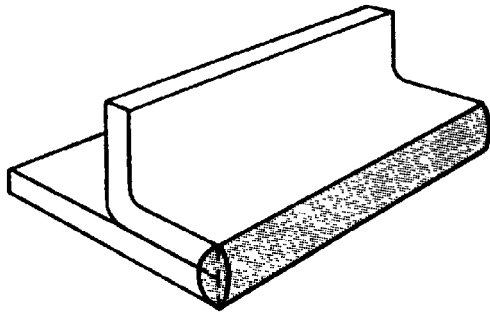
(C) EDGE WELD IN A FLANGED CORNER JOINT
