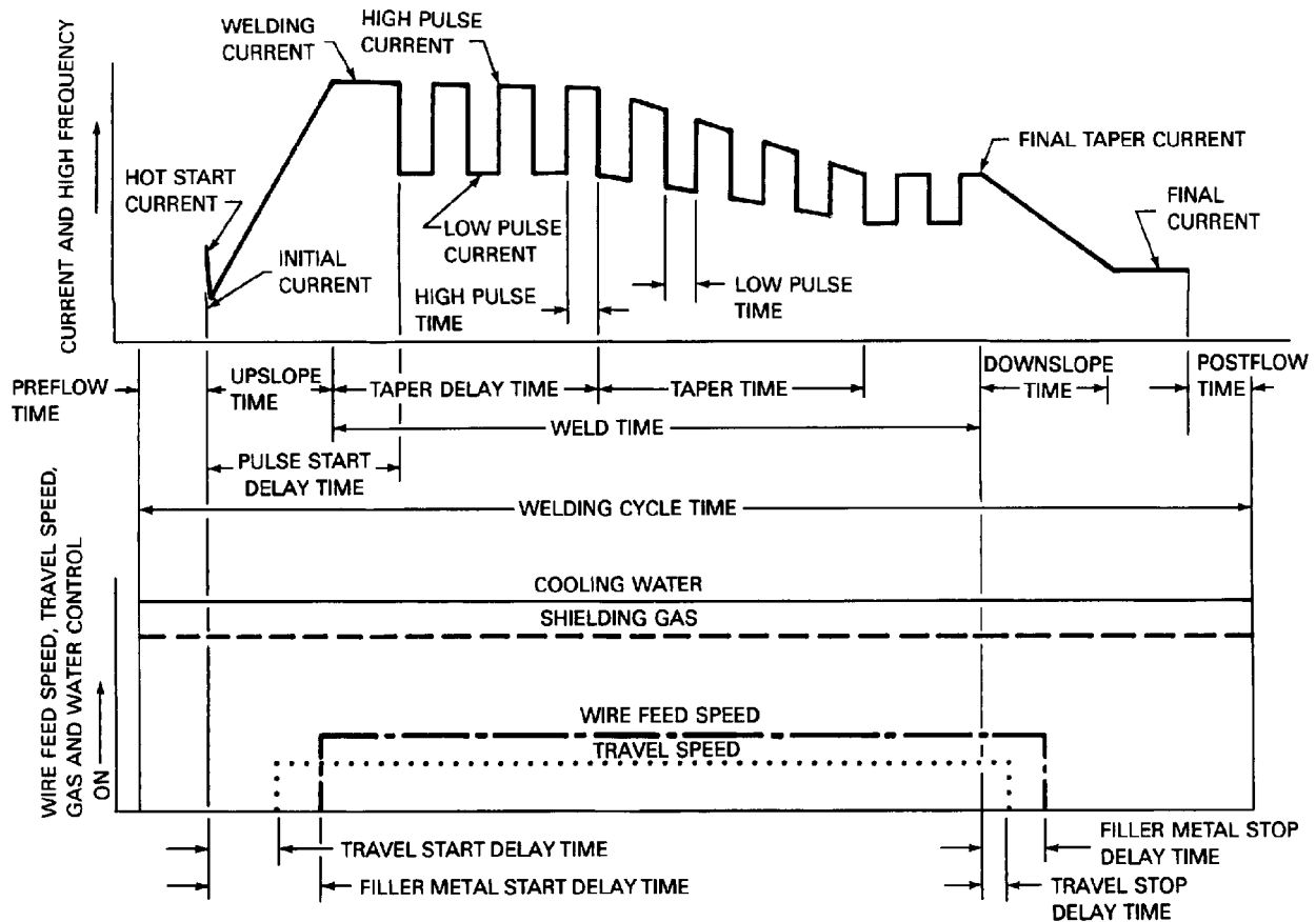
Figure 52 — Typical GTAW or PAW Program for Automatic Welding
