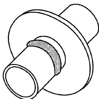
(E) MULTIPLE WELDING TEST POSITION WITH RESTRICTION RING—6GR
