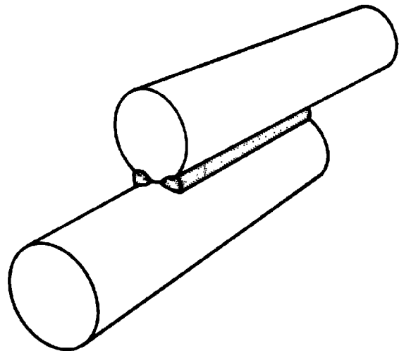
(G) DOUBLE-FLARE-V-GROOVE WELD
