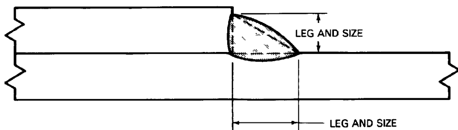
(E) UNEQUAL LEG FILLET WELD
