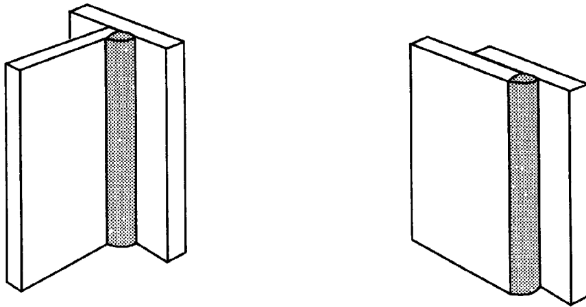
(C) VERTICAL WELDING TEST POSITION—3F
