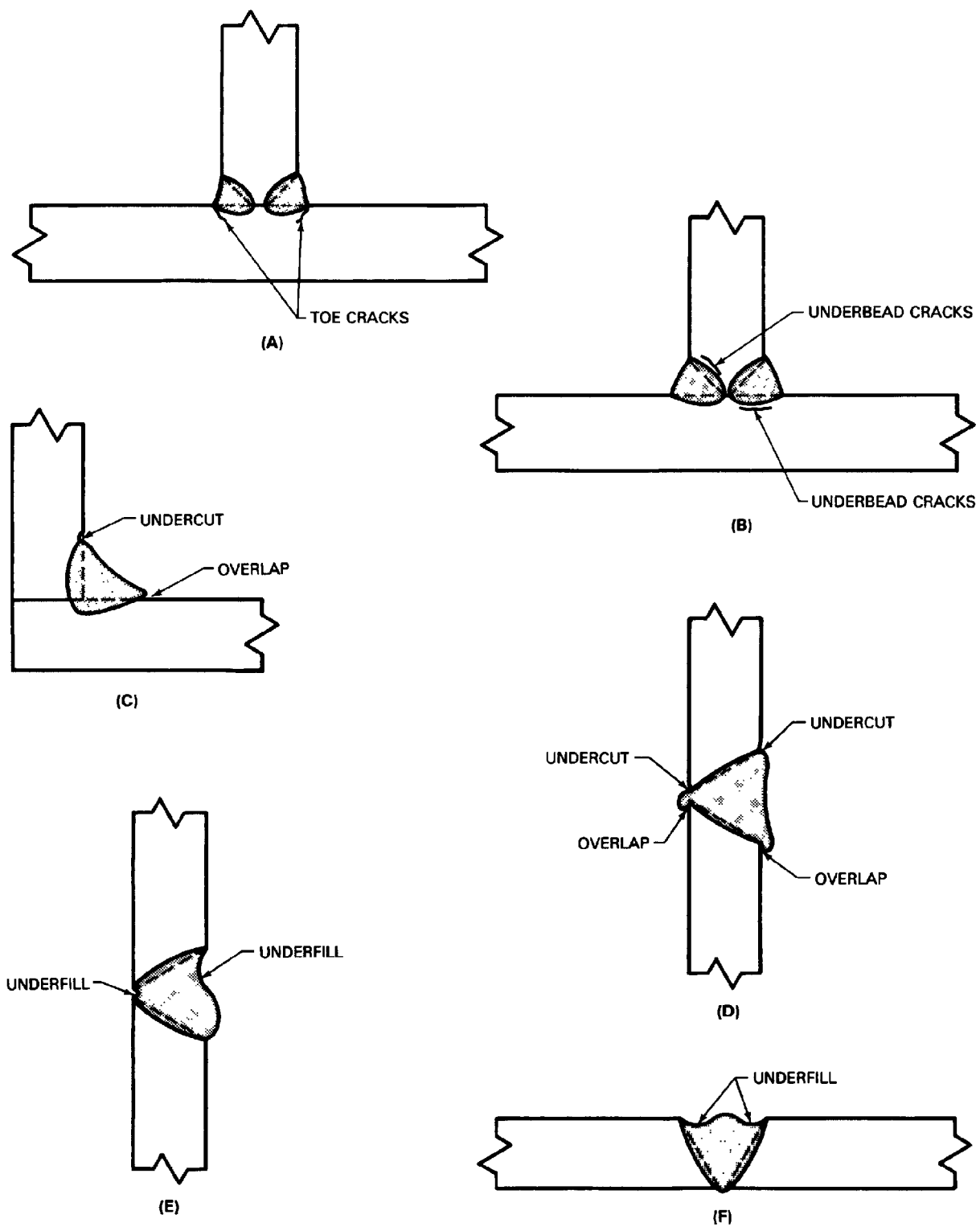
Figure 32 — Weld Discontinuities
