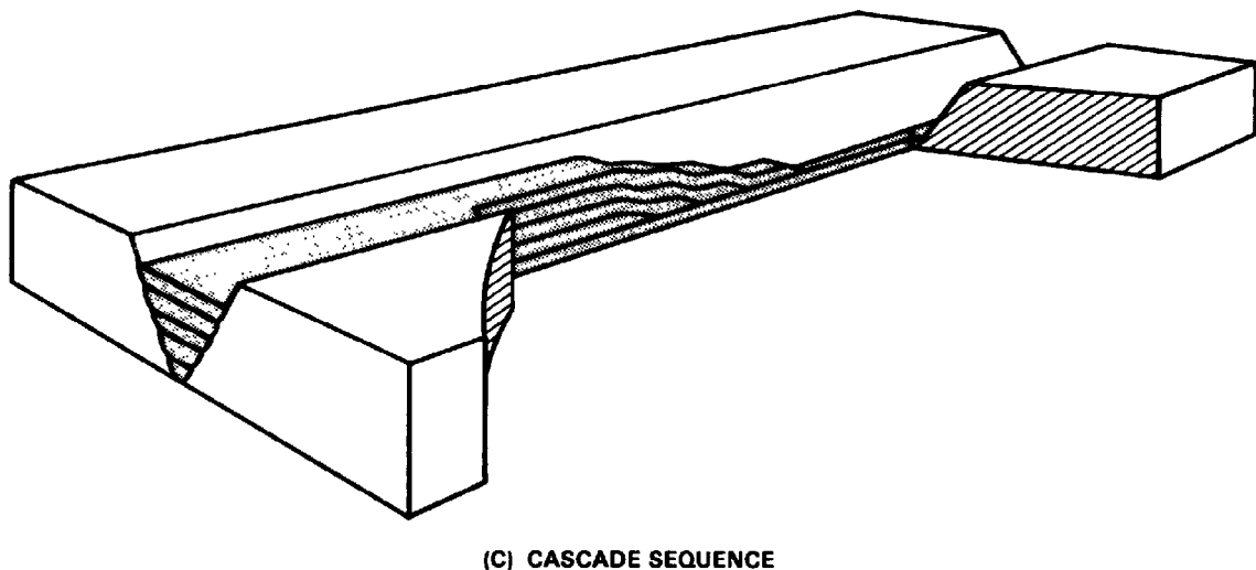
Figure 23 — Welding Sequence
