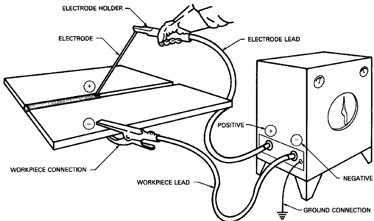
(A) DIRECT CURRENT ELECTRODE POSITIVE
