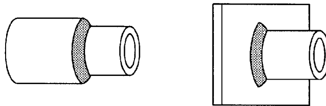
(E) MULTIPLE WELDING TEST POSITION—5F
