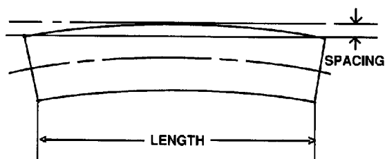
Figure 1 - Measurement Procedure for Straightness
