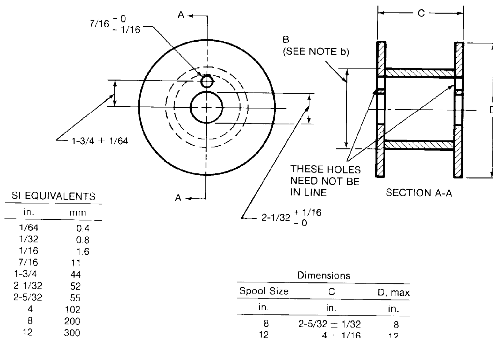
Figure 4—Dimensions of 4 in. (100 mm) Diameter Spool
