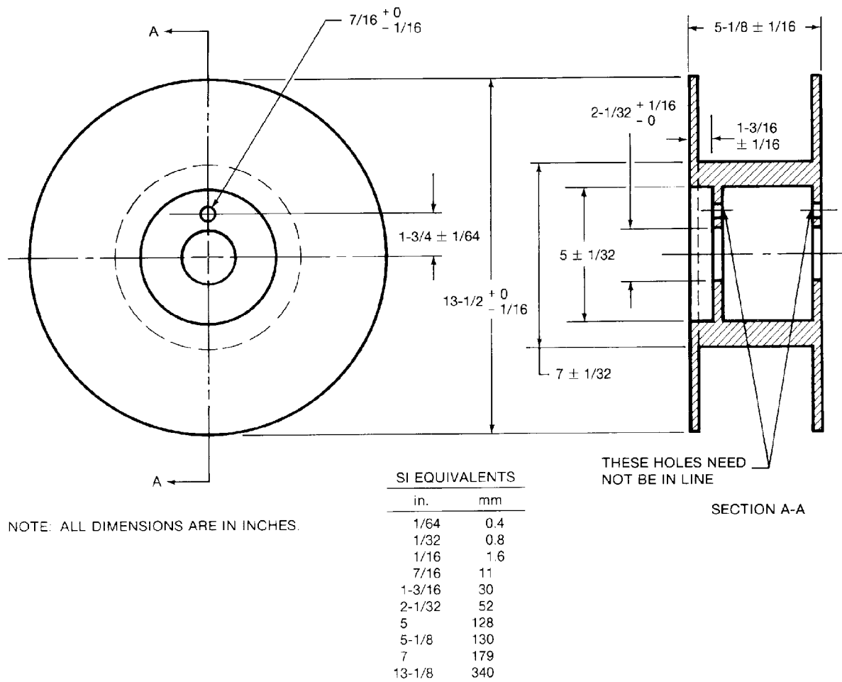
Figure 6—Dimensions of 13-1/2 in. (340 mm) Diameter Spool
