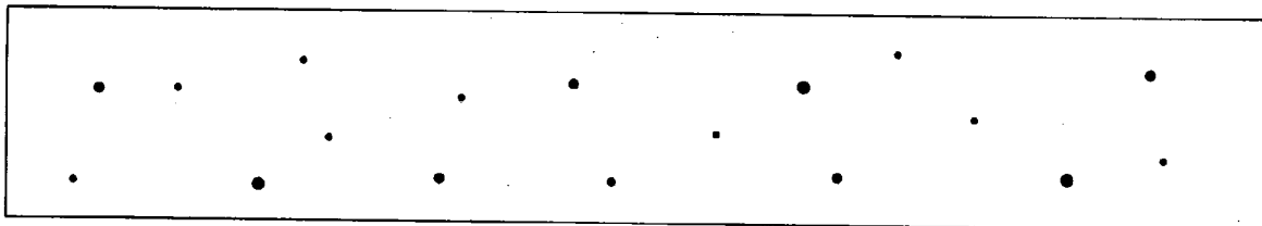
(A) ASSORTED POROSITY AND/OR INCLUSIONS
