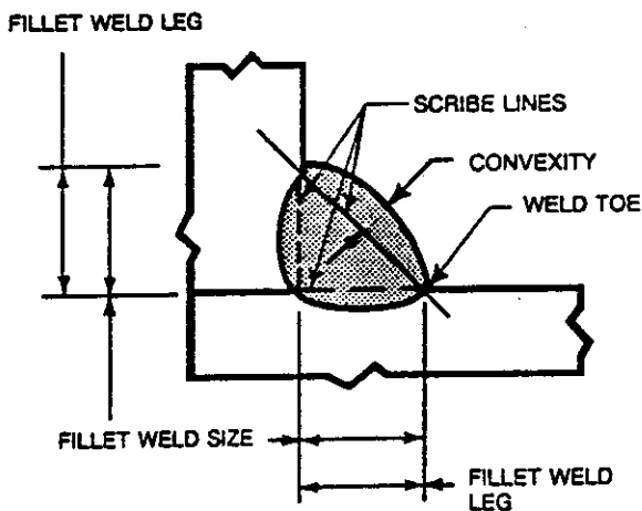
(B) CONVEX FILLET WELD
