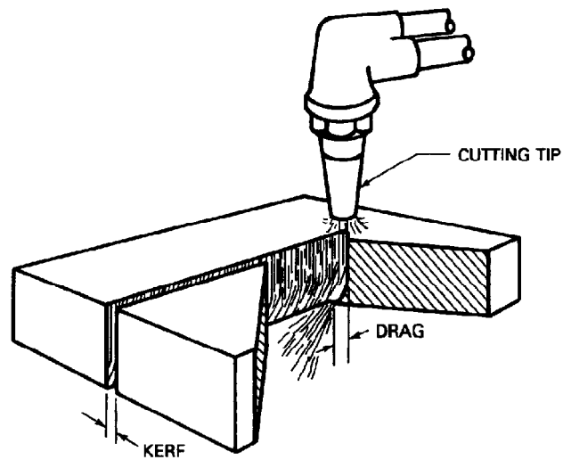
Figure 41 — Oxygen Cutting
