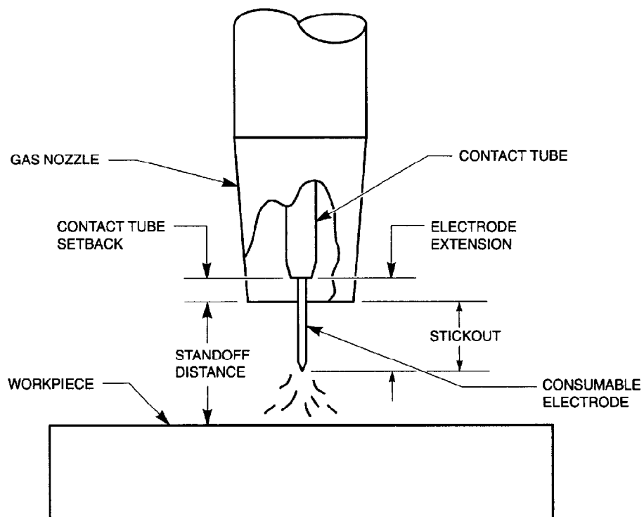
Figure 38 — Gas Metal Arc Welding Gun Nomenclature
