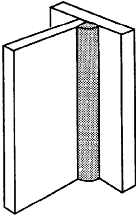
(C) VERTICAL WELDING TEST POSITION—3F
