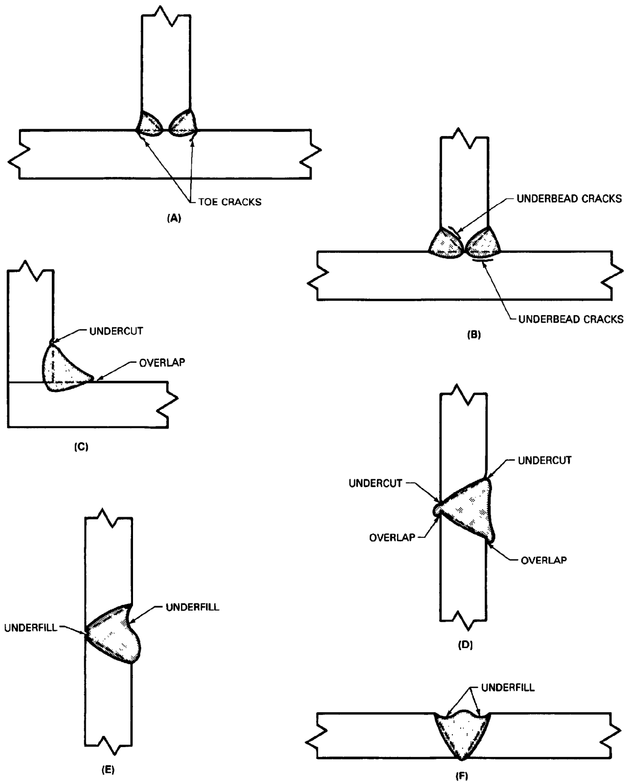
Figure 32 — Weld Discontinuities
