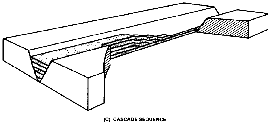
Figure 23 — Welding Sequence
