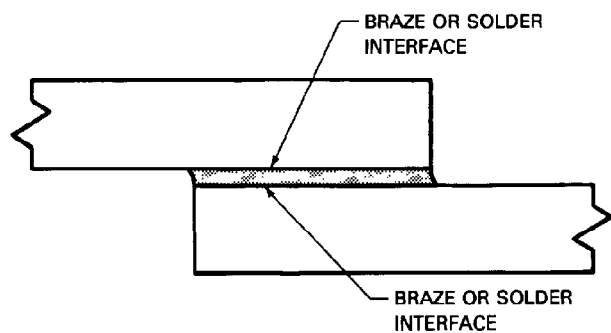
(A) BRAZED OR SOLDERED JOINT
