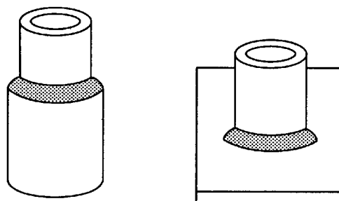
(B) HORIZONTAL WELDING TEST POSITION—2F
