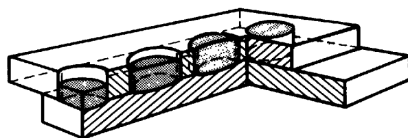
(E) PLUG WELDS
