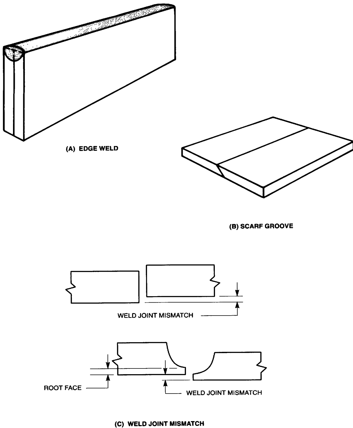
Figure 13 — Edge Weld, Scarf Groove, and Weld Joint Mismatch
