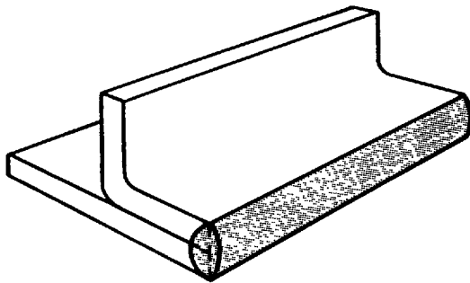
(C) EDGE WELD IN A FLANGED CORNER JOINT
