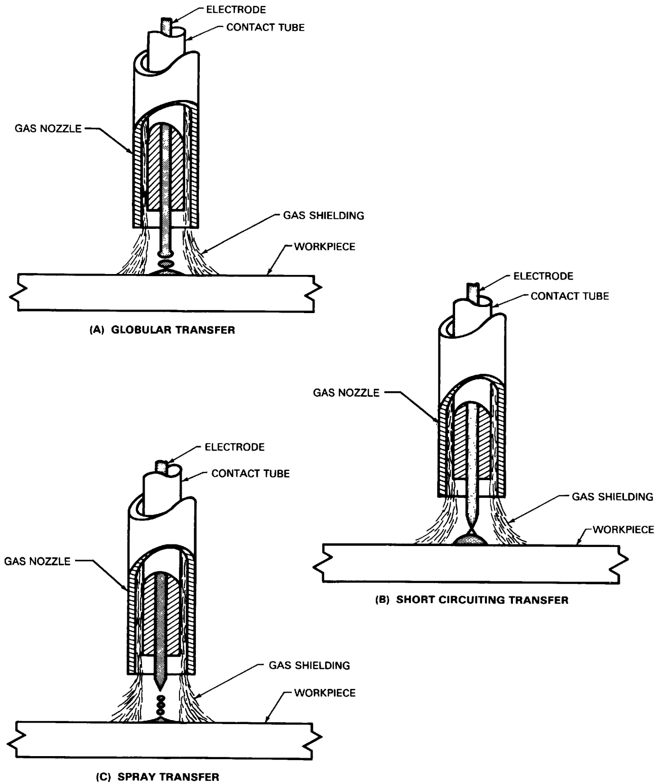
Figure 39 — Metal Transfer in Gas Metal Arc Welding
