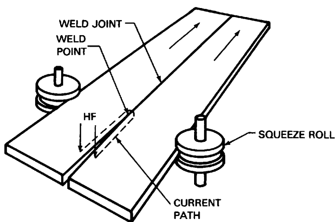
(A) BUTT JOINT MADE BY HIGH-FREQUENCY UPSET WELDING
