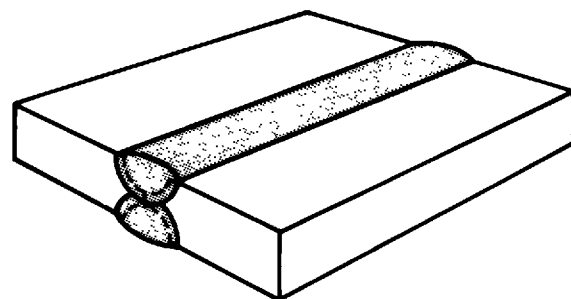
(E) DOUBLE-U-GROOVE WELD
