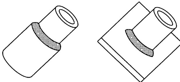
(F) MULTIPLE WELDING TEST POSITION—6F
