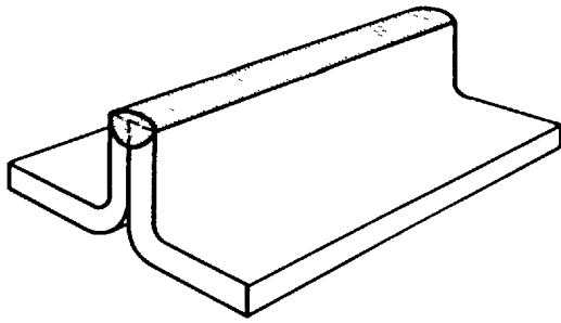
(A) EDGE WELD IN A FLANGED BUTT JOINT
