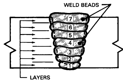
(E) CROSS-SECTIONAL SEQUENCE
