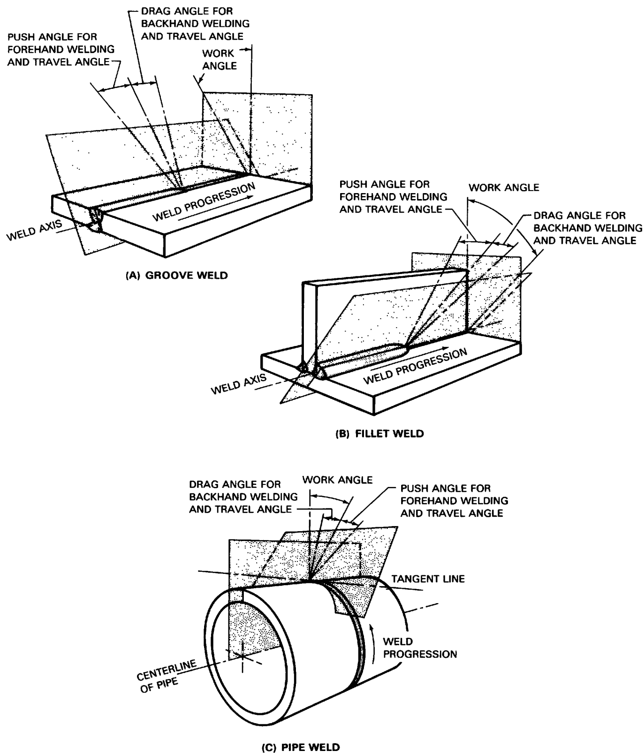
Figure 21 — Position of Electrode, Gun, Torch, Rod, or Beam
