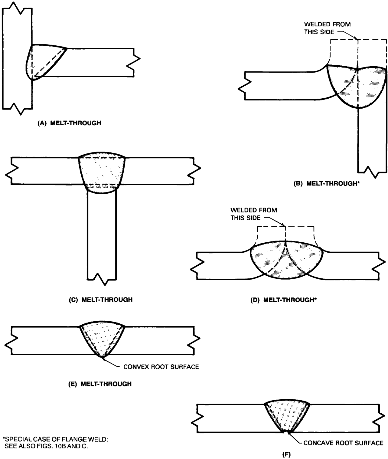
Figure 27 — Melt-Through and Root Surface Profile
