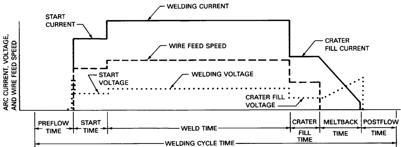
Figure 53 — Typical GMAW, FCAW, and SAW Program for Automatic Welding
