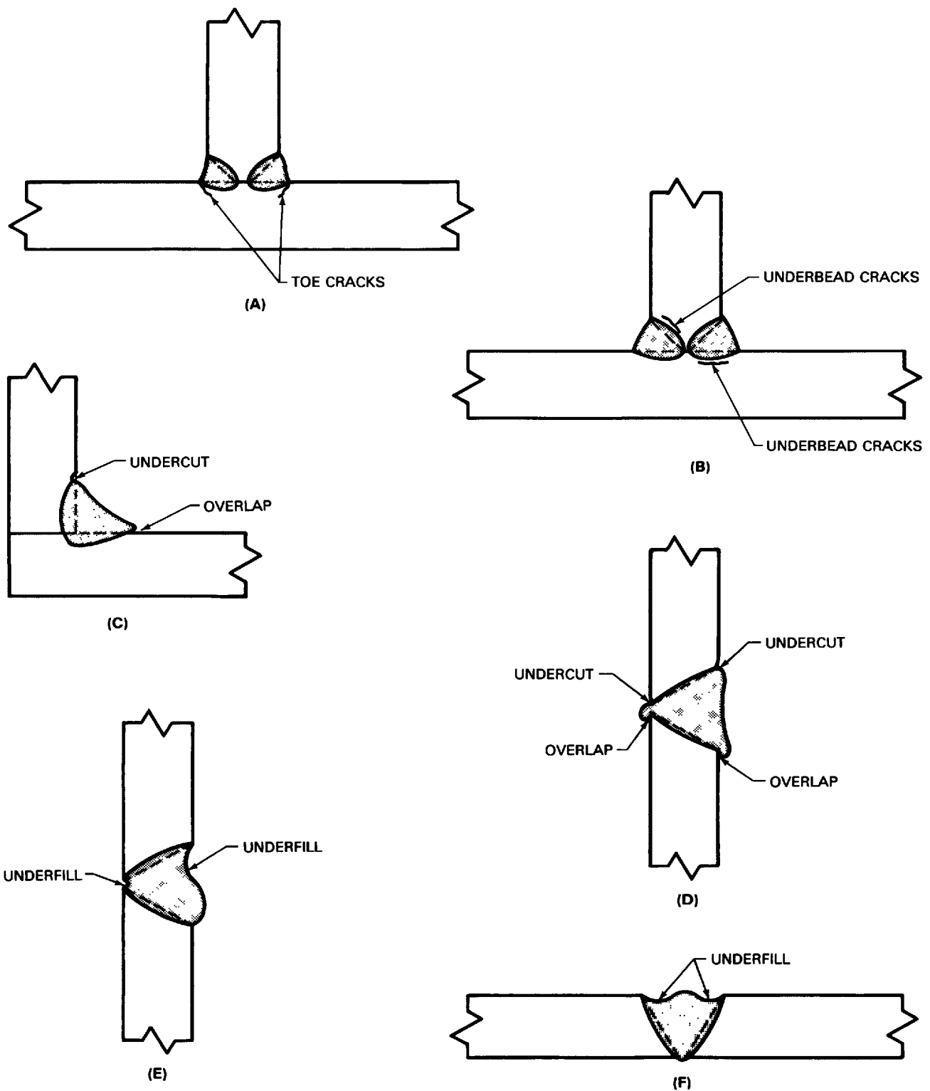
Figure 32 — Weld Discontinuities
