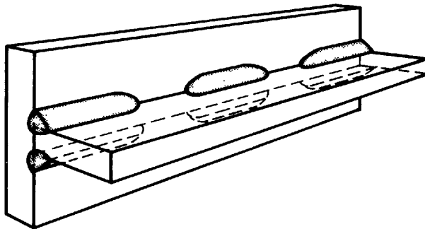
(G) CHAIN INTERMITTENT FILLET WELD
