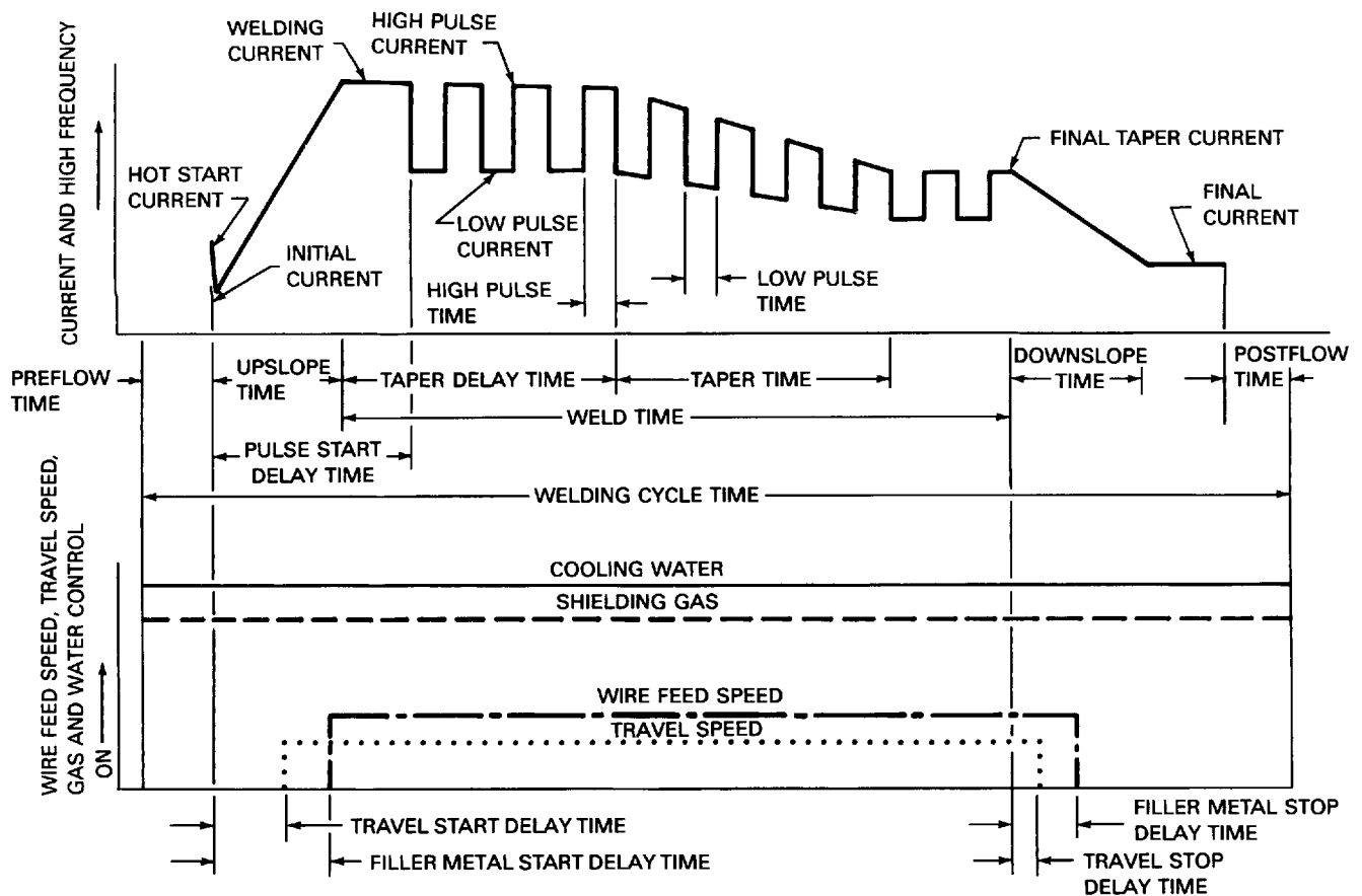
Figure 52 — Typical GTAW or PAW Program for Automatic Welding
