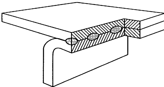
(E) RESISTANCE SPOT WELDS IN A FLANGED CORNER JOINT
