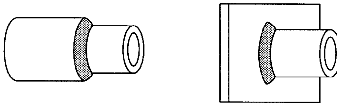
(E) MULTIPLE WELDING TEST POSITION—5F
