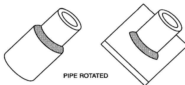
(A) FLAT WELDING TEST POSITION—1F
