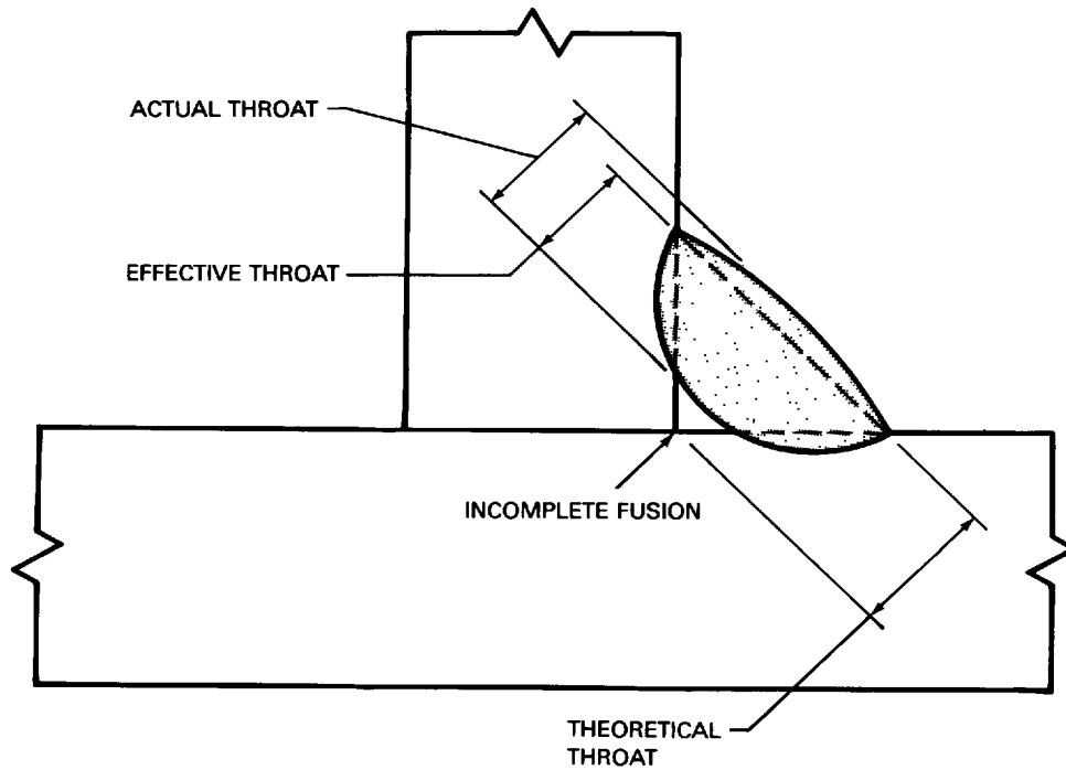
(C) FILLET WELD WITH INCOMPLETE FUSION
