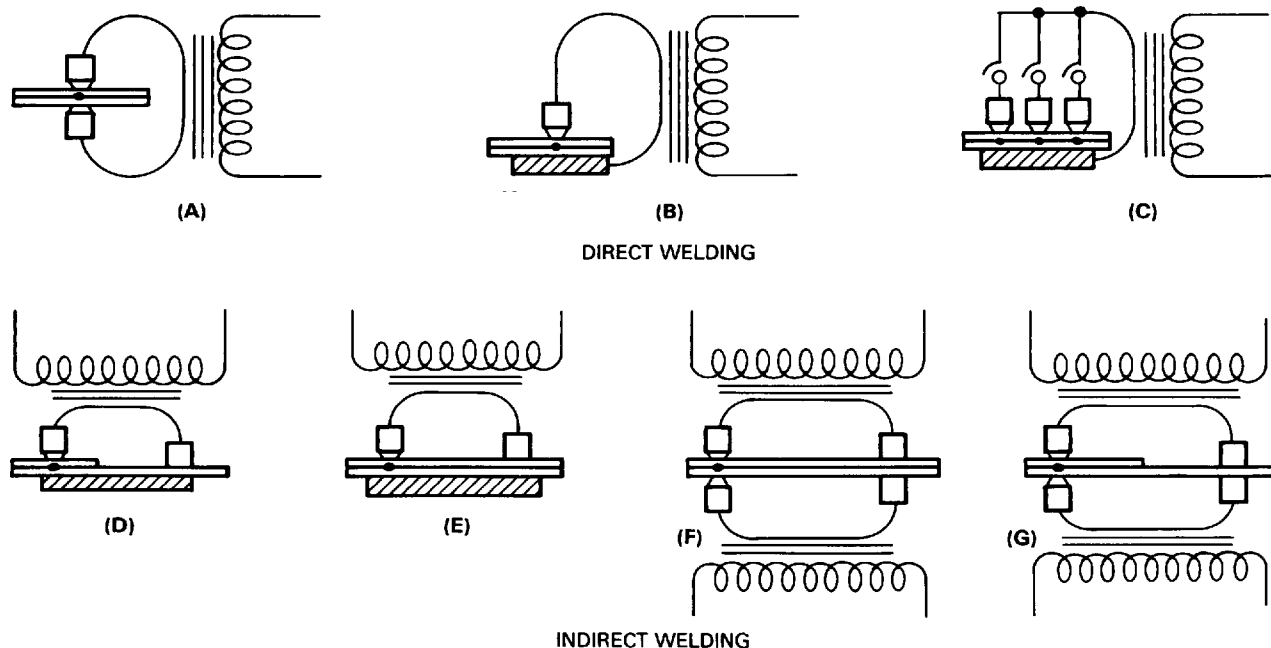
Figure 47 — Typical Arrangements for Single Spot Welds
