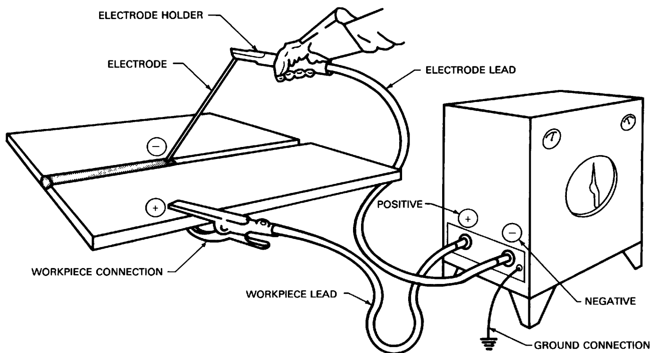
(B) DIRECT CURRENT ELECTRODE NEGATIVE
