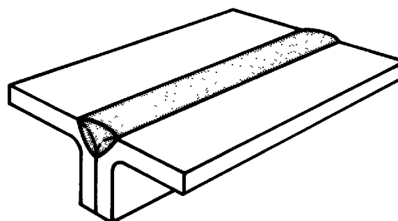
(H) SINGLE-FLARE-V-GROOVE WELD
