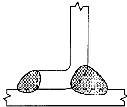
(F) FILLET WELD AND FLARE-BEVEL-GROOVE WELD IN A FLANGED T-JOINT
