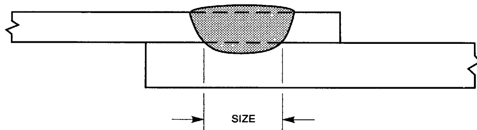
(G) ARC SEAM OR ARC SPOT WELD SIZE
