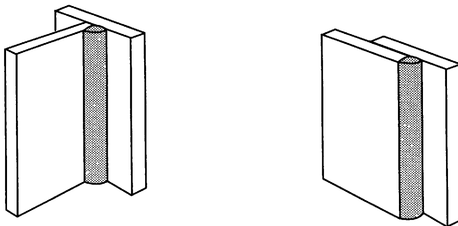
(C) VERTICAL WELDING TEST POSITION—3F
