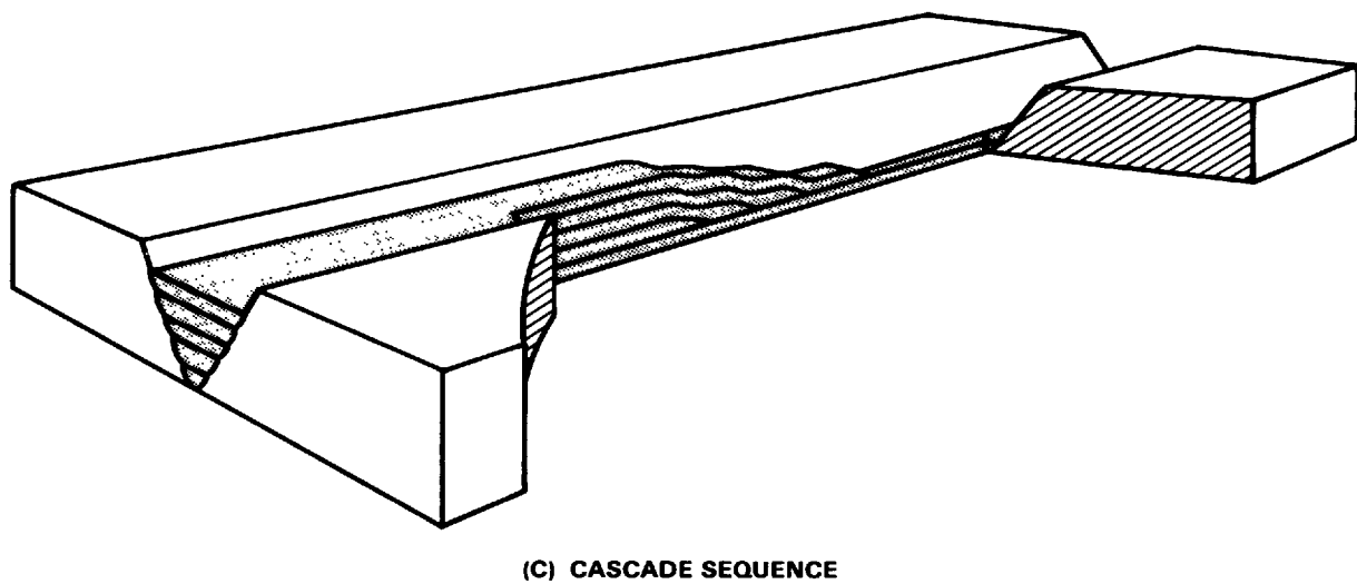
Figure 23 — Welding Sequence
