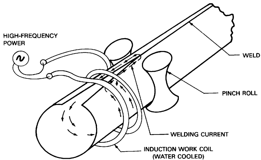
(E) INDUCTION UPSET WELDING OF TUBE
