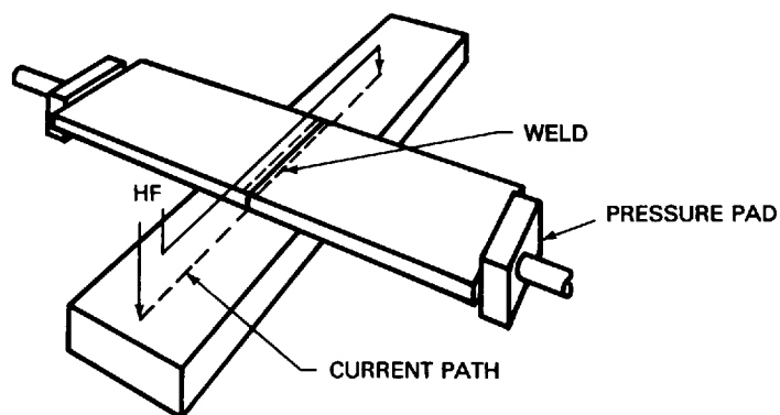
(B) BUTT JOINT MADE BY HIGH-FREQUENCY UPSET WELDING
