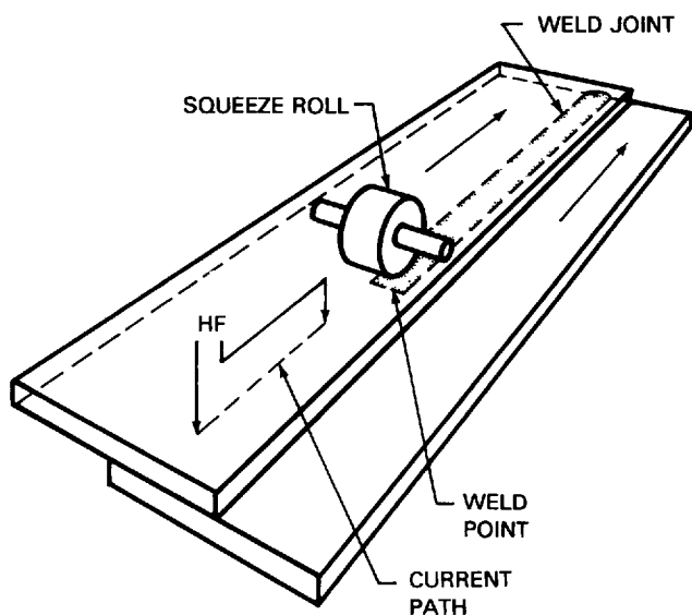
(C) LAP JOINT MADE BY HIGH-FREQUENCY SEAM WELDING
