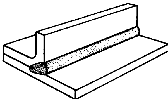
(G) SINGLE-FLARE-BEVEL GROOVE WELD
