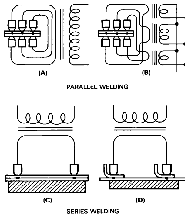
Figure 46 — Typical Arrangements for Multiple Spot Welding
