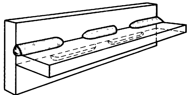
(H) STAGGERED INTERMITTENT FILLET WELD
