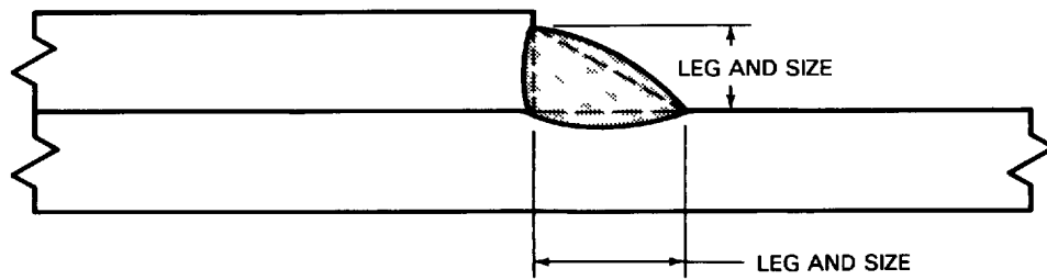
(E) UNEQUAL LEG FILLET WELD
