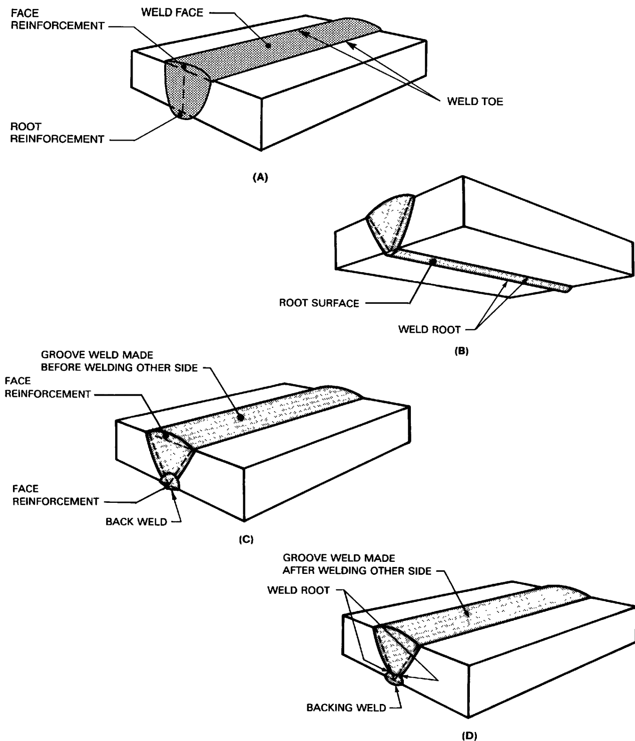
Figure 24 — Parts of a Weld
