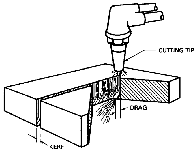
Figure 41 — Oxygen Cutting
