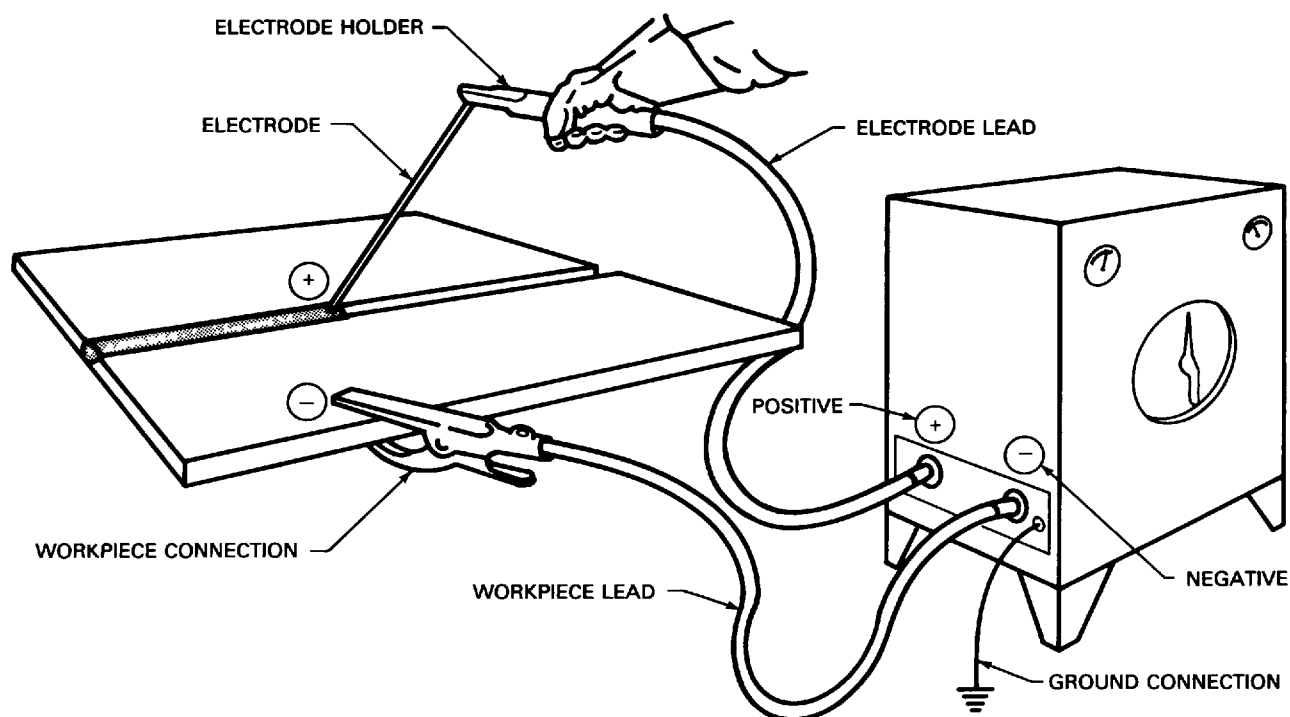
(A) DIRECT CURRENT ELECTRODE POSITIVE
