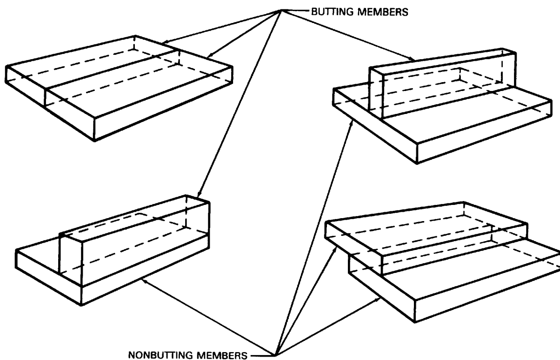
Figure 11 — Butting and Nonbutting Members
