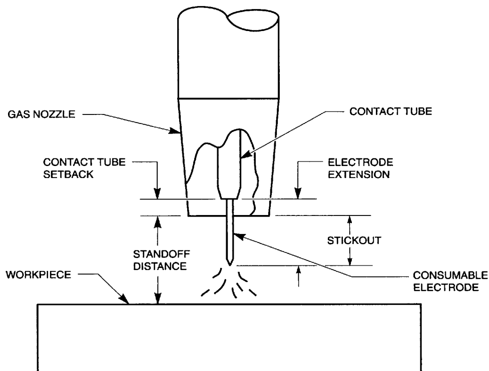
Figure 38 — Gas Metal Arc Welding Gun Nomenclature
