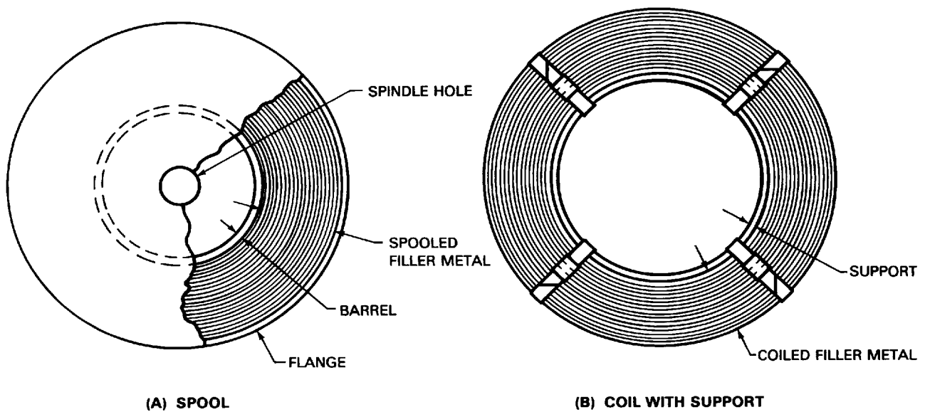
Figure 42 — Filler Metal Packaging
