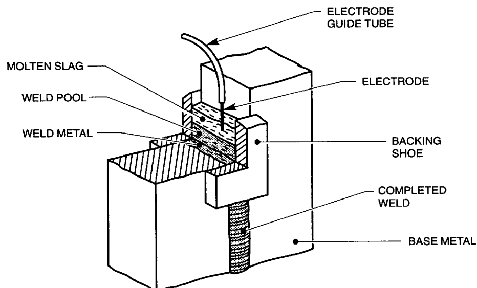
Figure 37 — Typical Arrangement for Electroslag Welding Process Nomenclature
