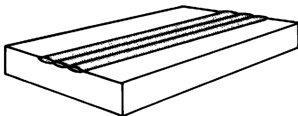
(C) SURFACING WELD
