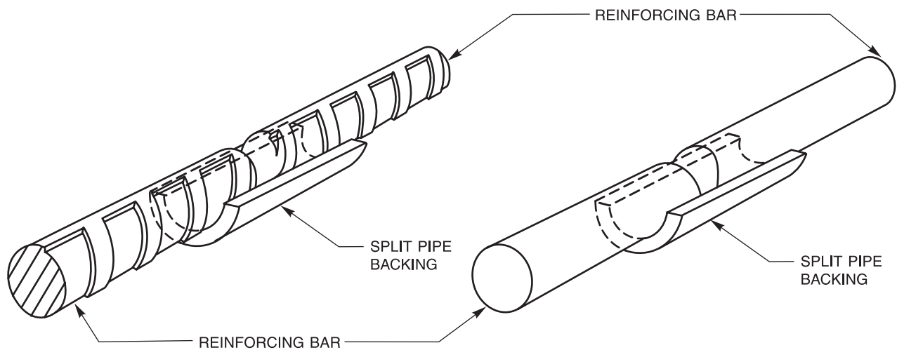
Figure B.12—Split Pipe Backing
