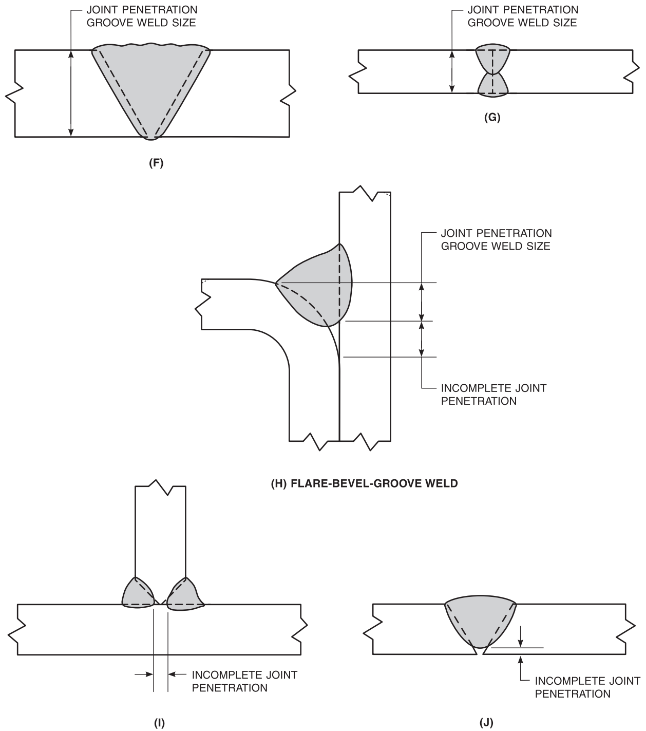
Figure B.26 (Continued)—Groove Weld Size and Joint Penetration
