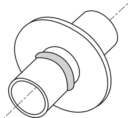
(C) MULTIPLE WELDING TEST POSITION—5G
