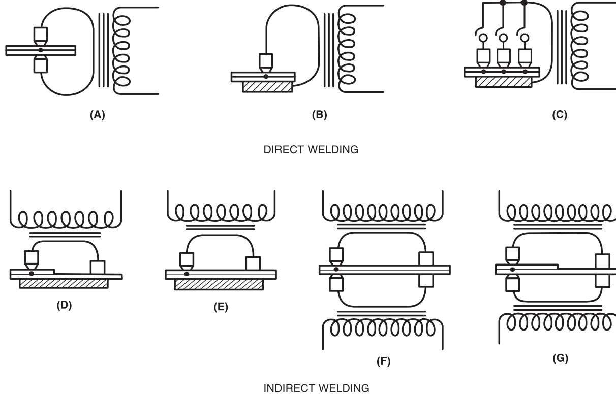
Figure B.47—Typical Arrangements for Single Spot Welds
