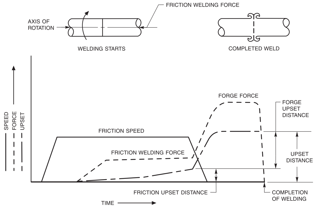
Figure B.45—Generalized Diagram of Direct Drive Friction Welding
