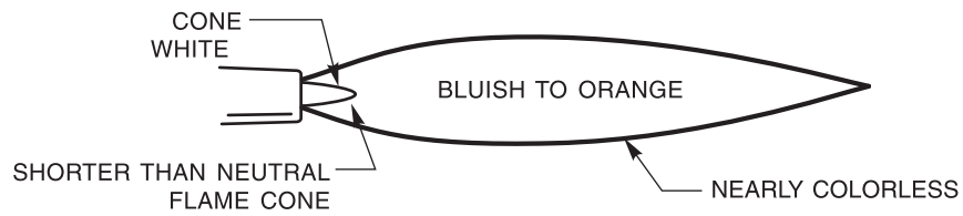
(C) OXIDIZING FLAME
