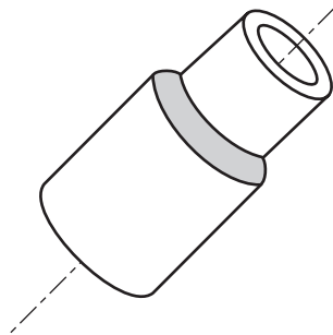
(F) MULTIPLE WELDING TEST POSITION—6F
