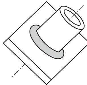
(F) MULTIPLE WELDING TEST POSITION—6F
