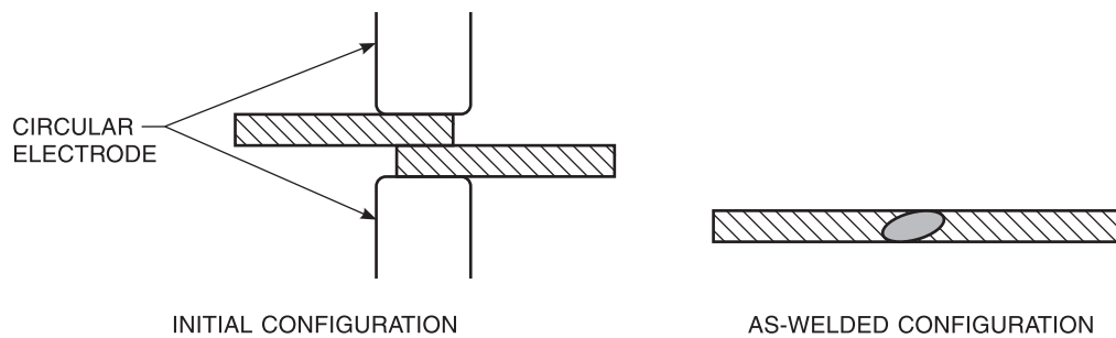
(G) EXAMPLE OF A MESH SEAM WELD
