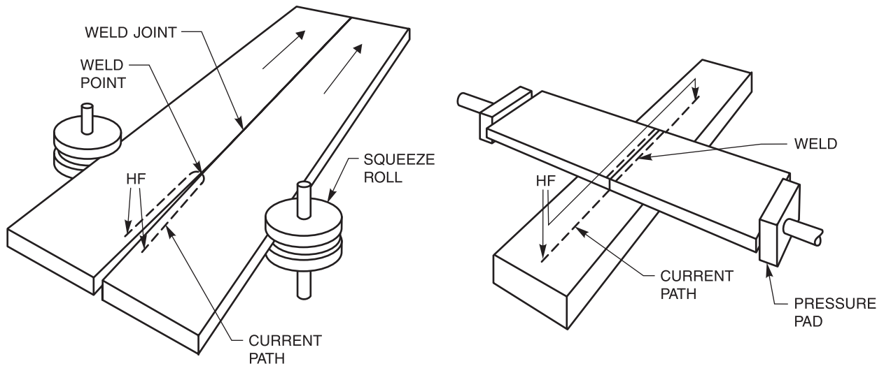
(A) BUTT JOINT MADE BY HIGH-FREQUENCY UPSET WELDING
