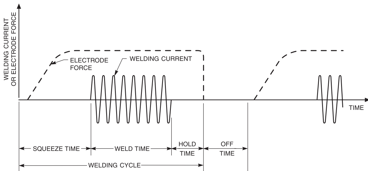
Figure B.50—Example of a Single-Impulse Resistance Spot Welding Schedule
