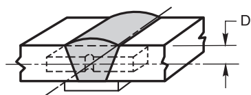
(B) LOCATION OF IMPACT TEST SPECIMENS
