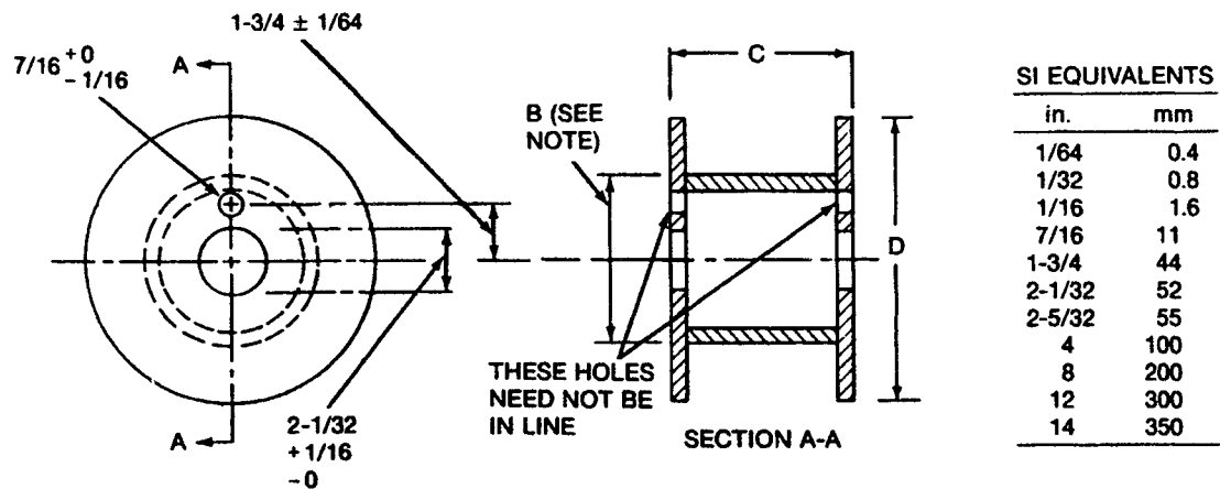
Figure 9A — Standard Spools — Dimensions of 4 in. Spools
