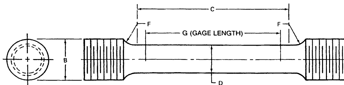
Dimensions of Specimen, in.
