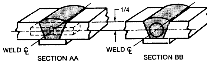
(C) LOCATION OF ALL-WELD-METAL TENSION SPECIMEN
