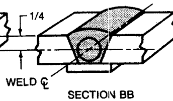
(C) LOCATION OF ALL-WELD-METAL TENSION SPECIMEN
