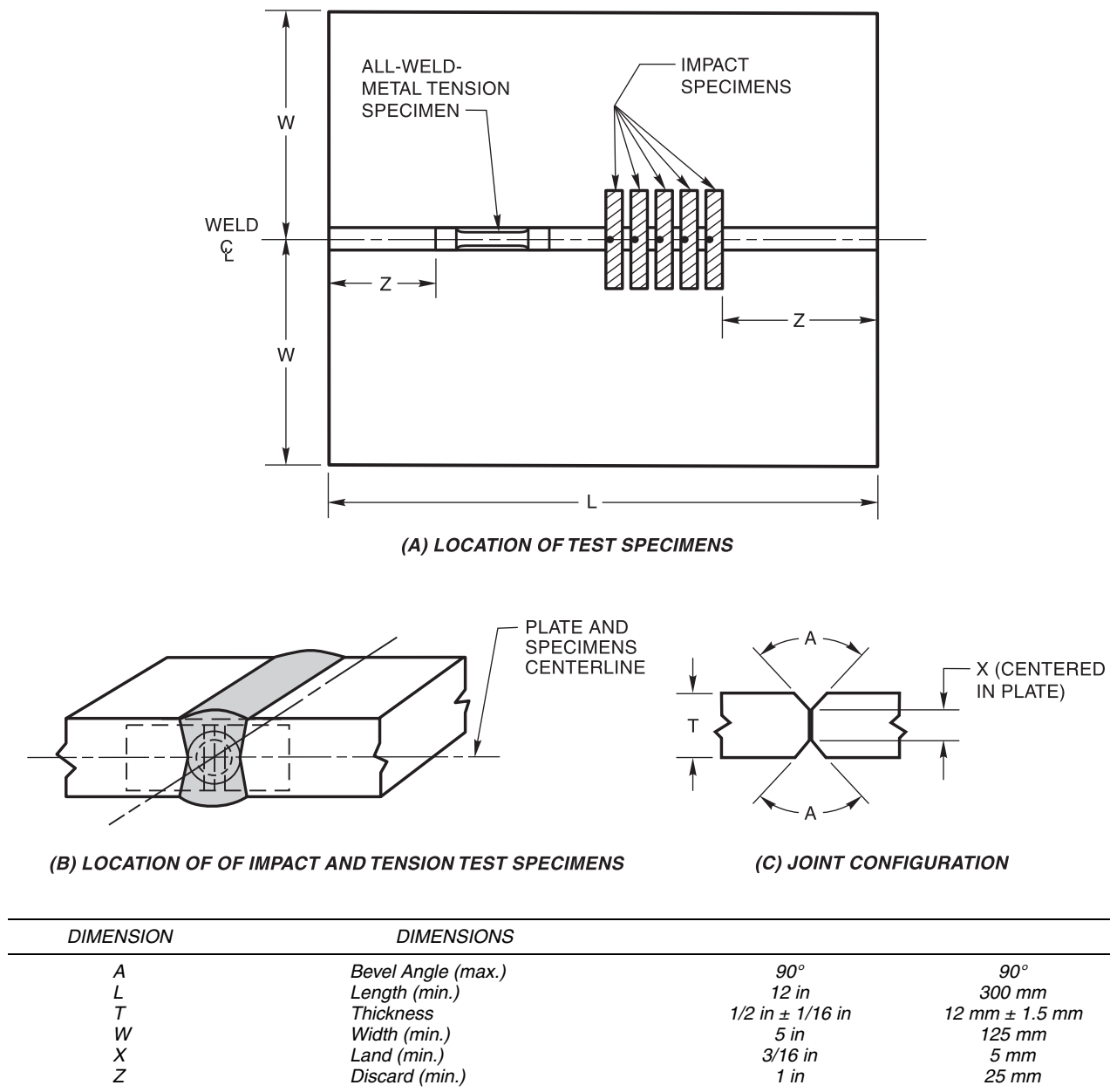
Figure 5—Two-Run Weld Test Assembly
