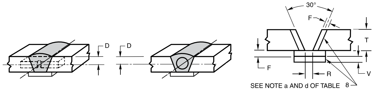
(B) LOCATION OF IMPACT TEST SPECIMENS
