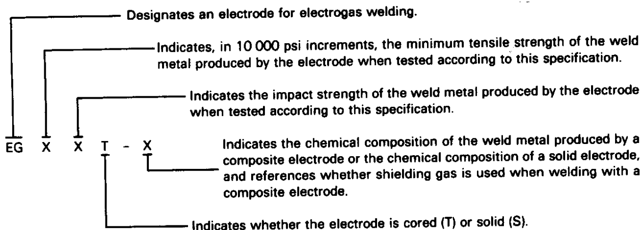
FIG. A1 CLASSIFICATION SYSTEM
