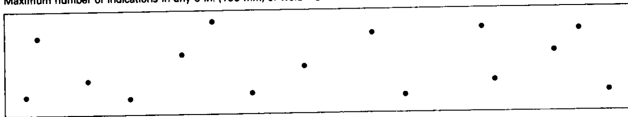
(C) MEDIUM POROSITY AND/OR INCLUSIONS
