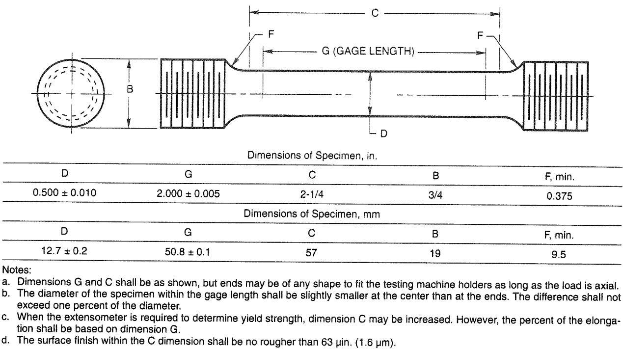
Figure 4—Tension Test Specimen
