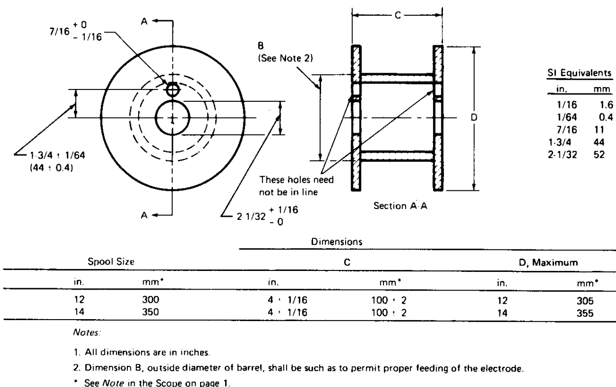
FIG. 3 DIMENSION OF 12 AND 14 in. (300 AND 350 mm)* SPOOLS
