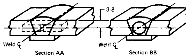
C. Orientation of impact specimen
