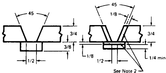
Standard test plate
