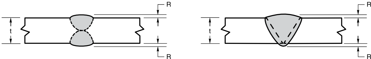
MAXIMUM REINFORCEMENT FOR GROOVE WELDS
