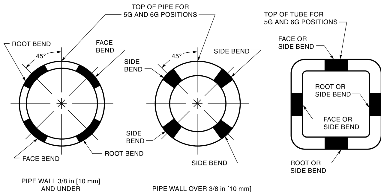
SPECIMENS FOR 5G AND 6G POSITIONS
