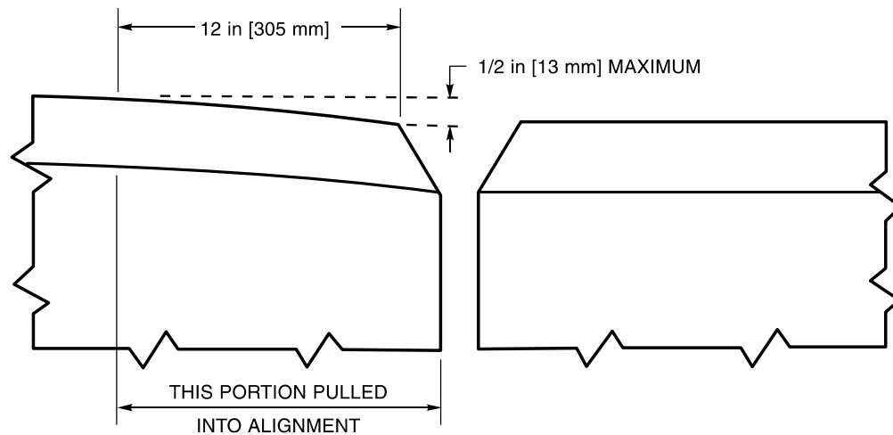
Figure C-4.3—Correction of Misaligned Members (see C-4.12.1.1)
