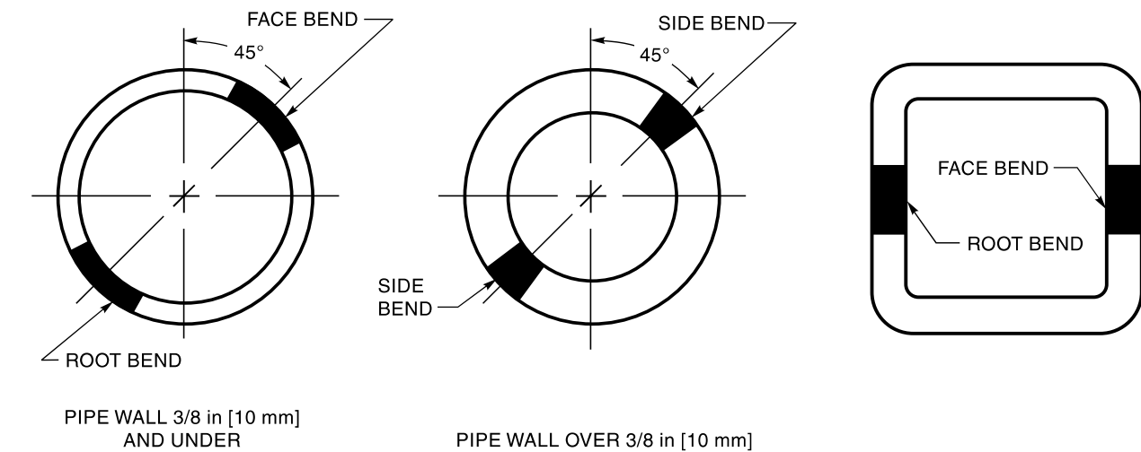
SPECIMENS FOR 1G AND 2G POSITIONS
