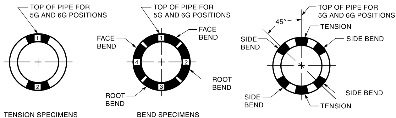
DETAIL A—3 in [75 mm] OR LESS IN DIAMETER
