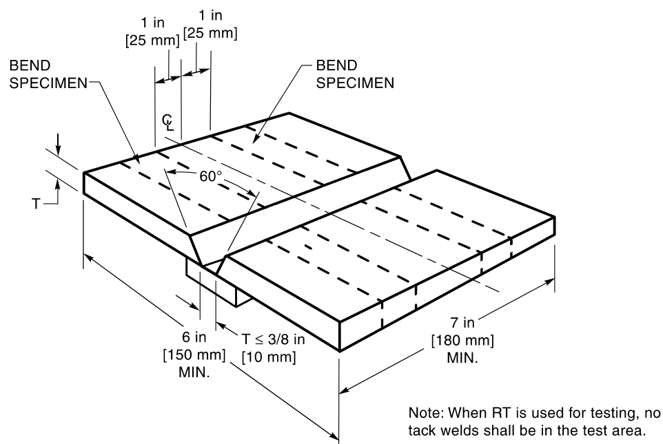
Figure 3.26—Performance Qualification in All Positions—Plate Thickness T > 1/8 in [3 mm] (see 3.19.1)
