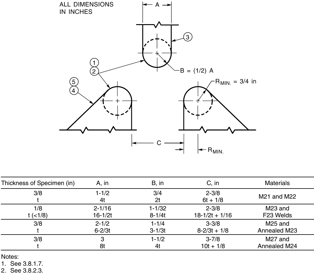
Figure 3.15—Roller-Type Guided Bend Jig (see 3.8.2.2) (Dimensions in Inches)
