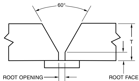
Figure 3.31—Tubular Groove Weld—Performance Qualification—With Backing (see 3.19.3(3))
