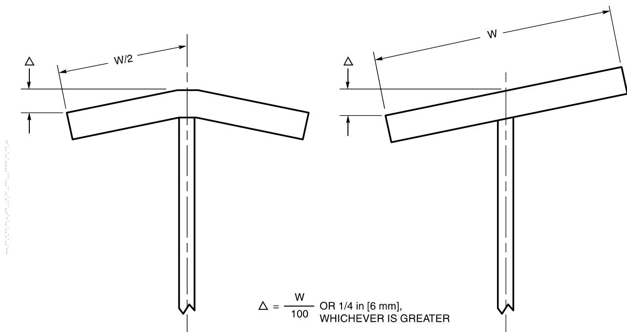
Figure C-4.4—Measurement of Flange Warpage and Tilt (see C-4.15.5)
