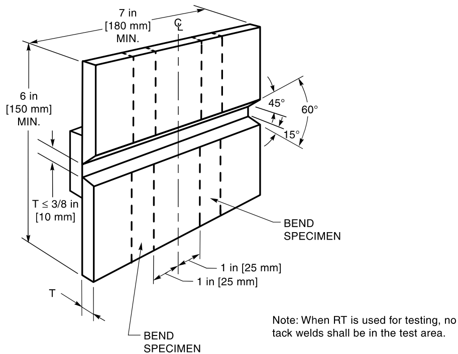
Figure 3.27—Performance Qualification in the Horizontal Position—Plate Thickness T > 1/8 in [3 mm] (see 3.19.1)
