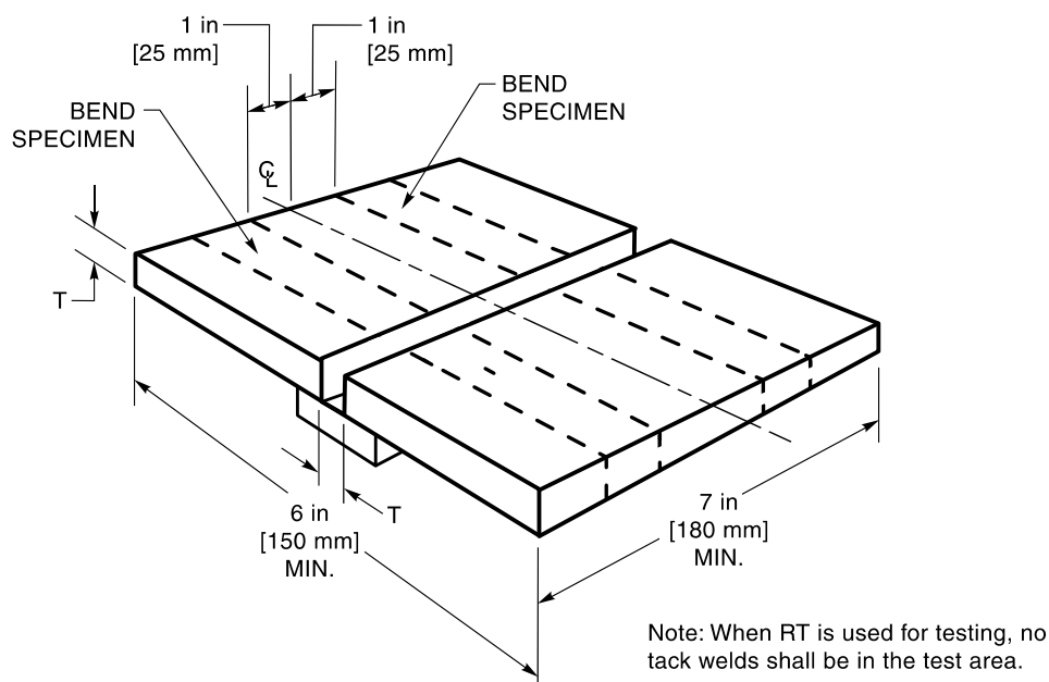
Figure 3.25—Performance Qualification in All Positions—Plate Thickness T \leq 1/8 in [3 mm] (see 3.19.1)
