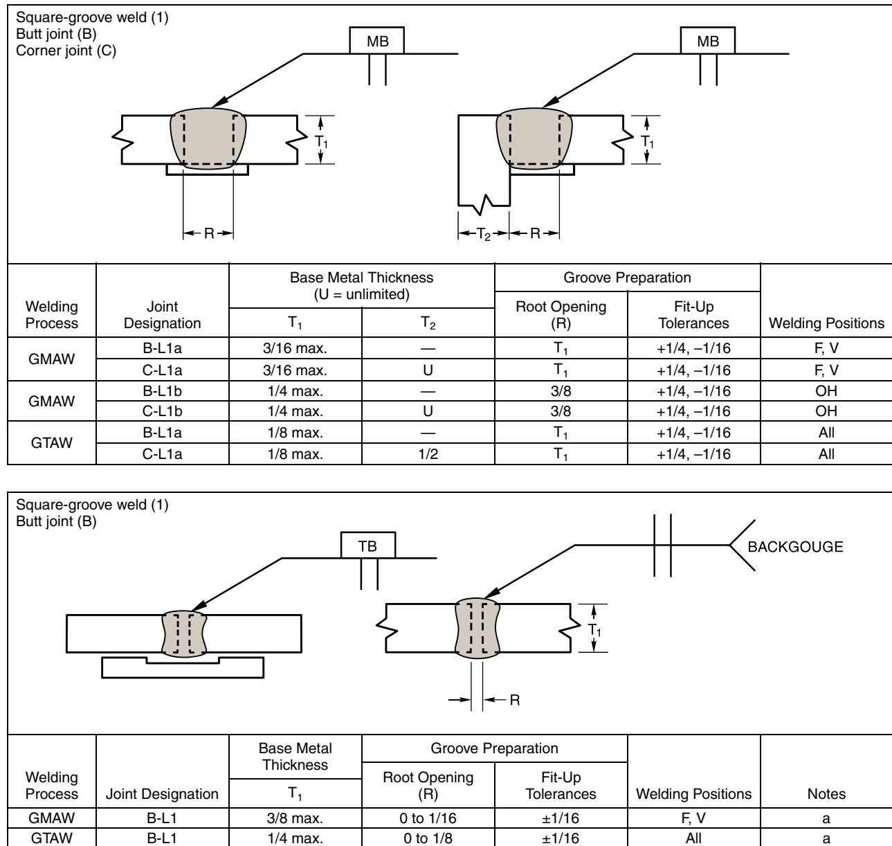
Figure B.1—Recommended CJP Groove Welded Joints (Inches)
