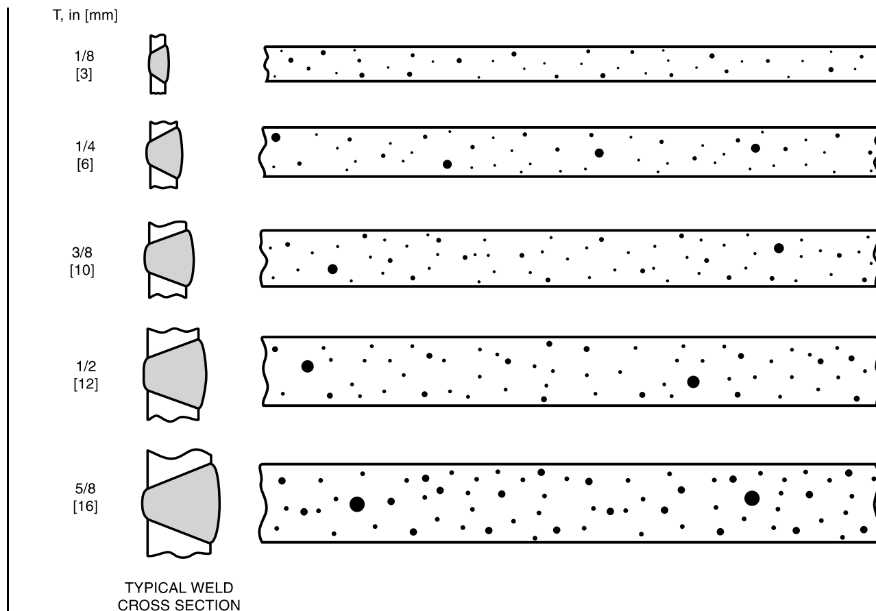
Figure 5.8—Maximum Acceptable Discontinuity RT Images (see 5.15.2.3)
