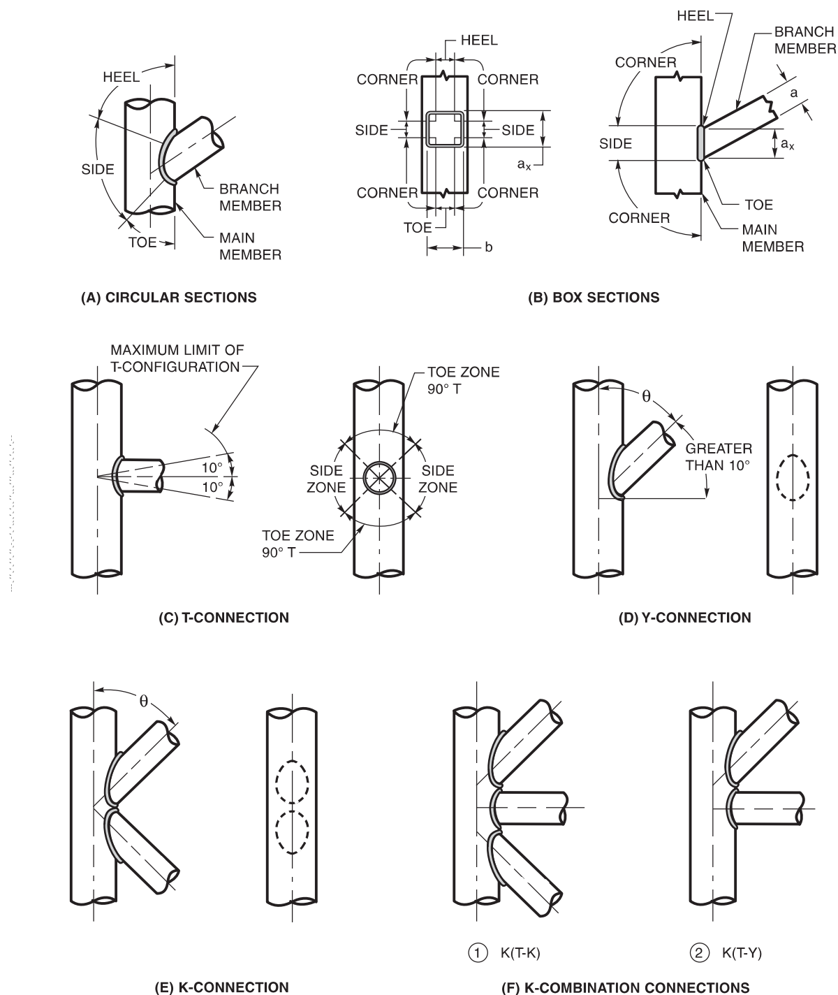
Figure D.1—Examples of Tubular Connections
