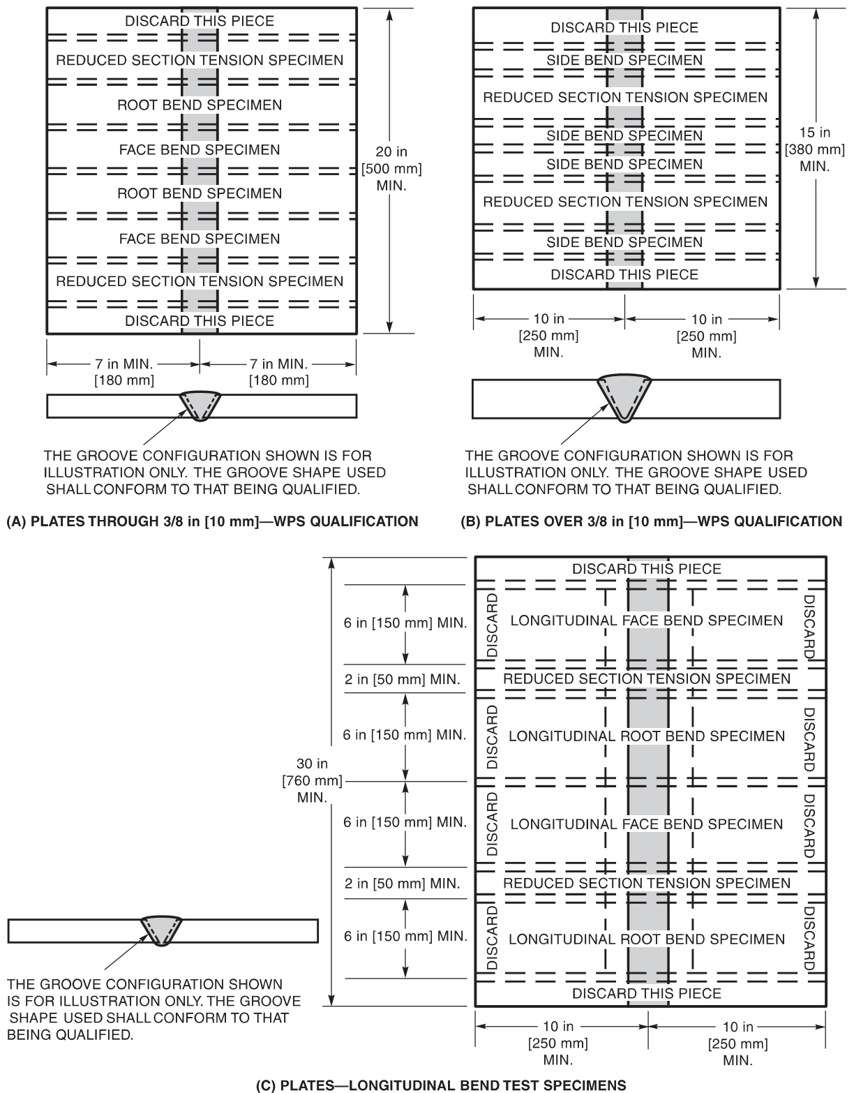
Figure 3.20—Location of Test Specimens for WPS Qualification—Plate (see 3.9.1 and 3.15.5.1)
