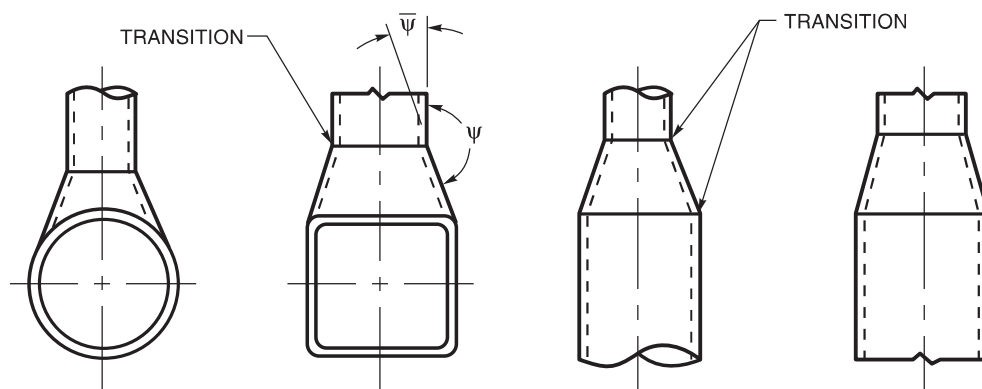
(K) FLARED CONNECTIONS AND TRANSITIONS
