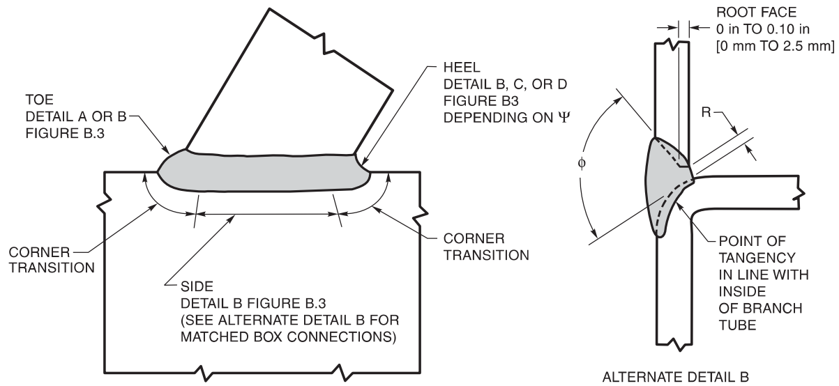
Figure B.3—PJP Box Connections
