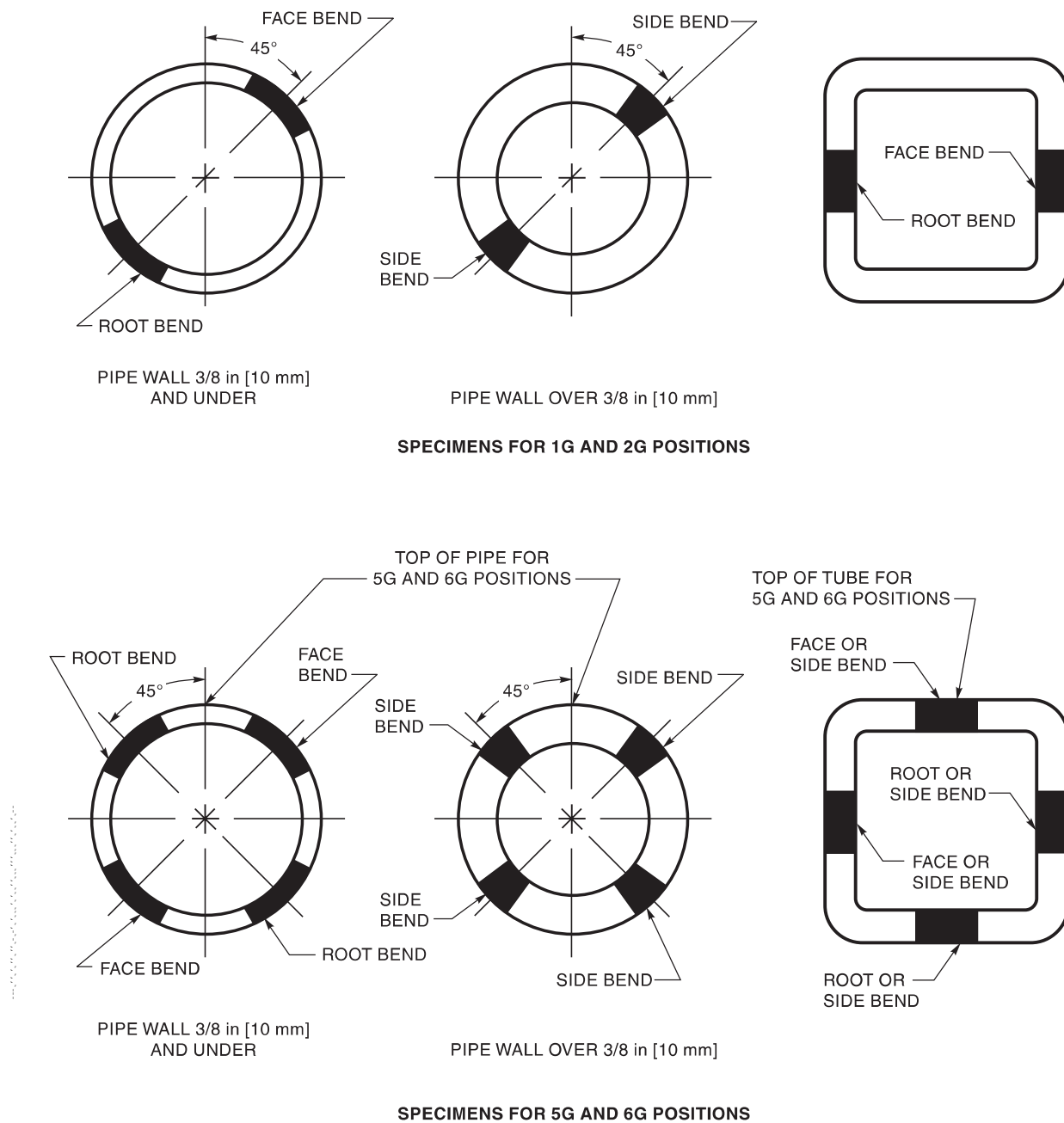
Figure 3.34—Location of Test Specimens on Welded Test Pipe and Box Tubing—Performance Qualification (see 3.21.4)
