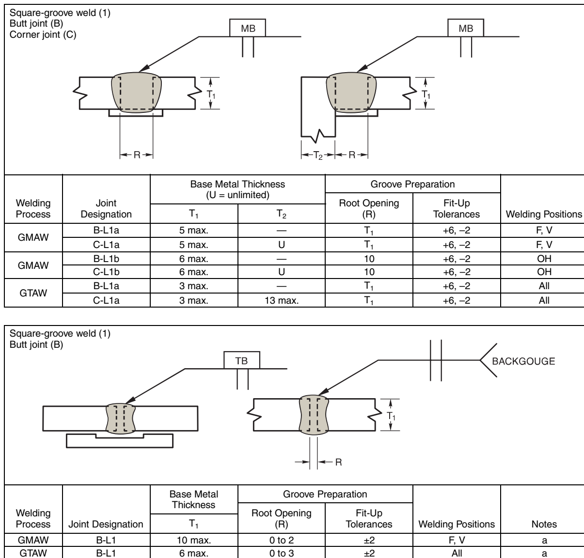
Figure B.1—Recommended CJP Groove Welded Joints (Millimeters)
