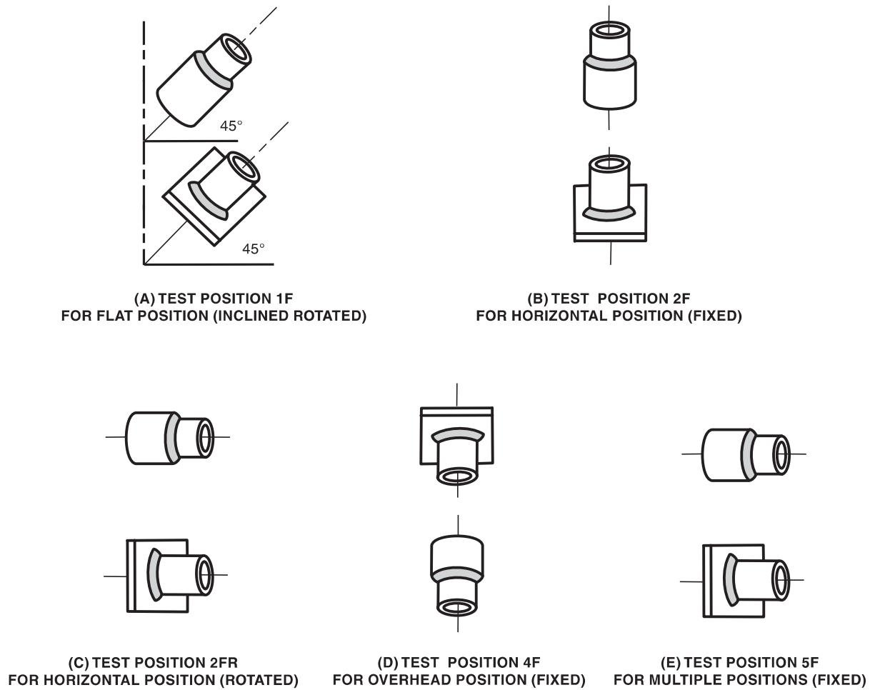
Figure 3.6—Positions of Test Pipes for Fillet Welds (see 3.4.1.4)
