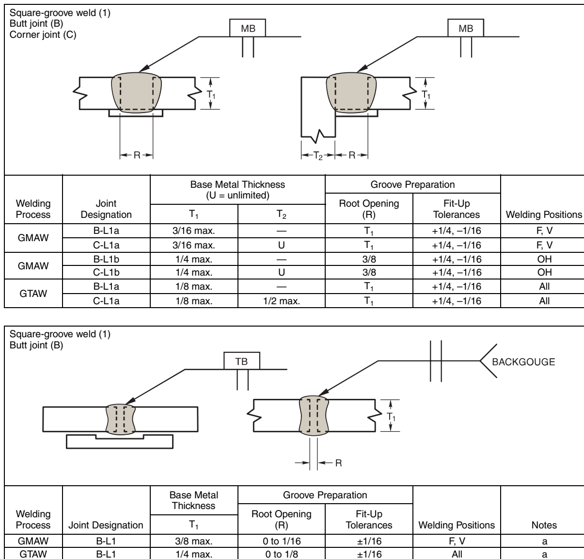
Figure B.1—Recommended CJP Groove Welded Joints (Inches)
