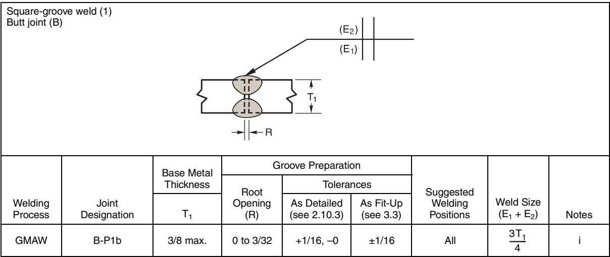
Figure B.2—Recommended PJP Groove Welded Joints (Inches)
