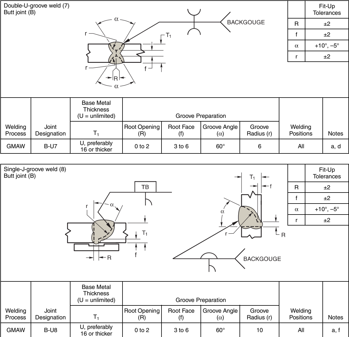
Figure B.1 (Continued)—Recommended CJP Groove Welded Joints (Millimeters)
