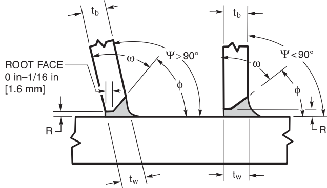
DETAIL B
