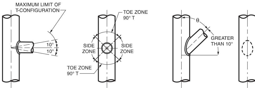
(C) T-CONNECTION
