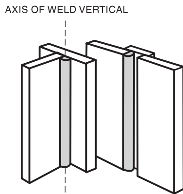
(C) TEST POSITION 3F (VERTICAL)
