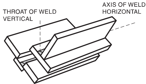
(A) TEST POSITION 1F (FLAT)
