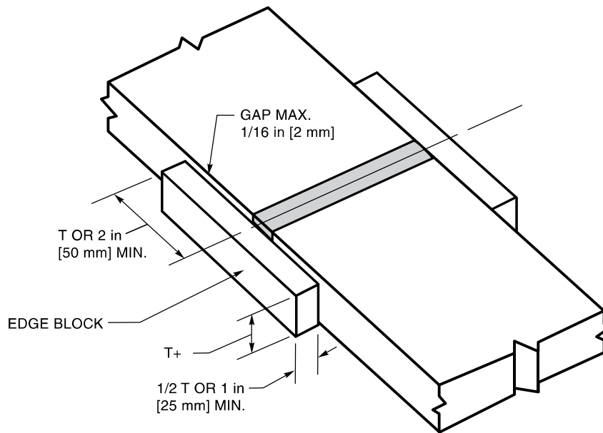
Figure 5.7—Radiographic Edge Blocks (see 5.10.13)
