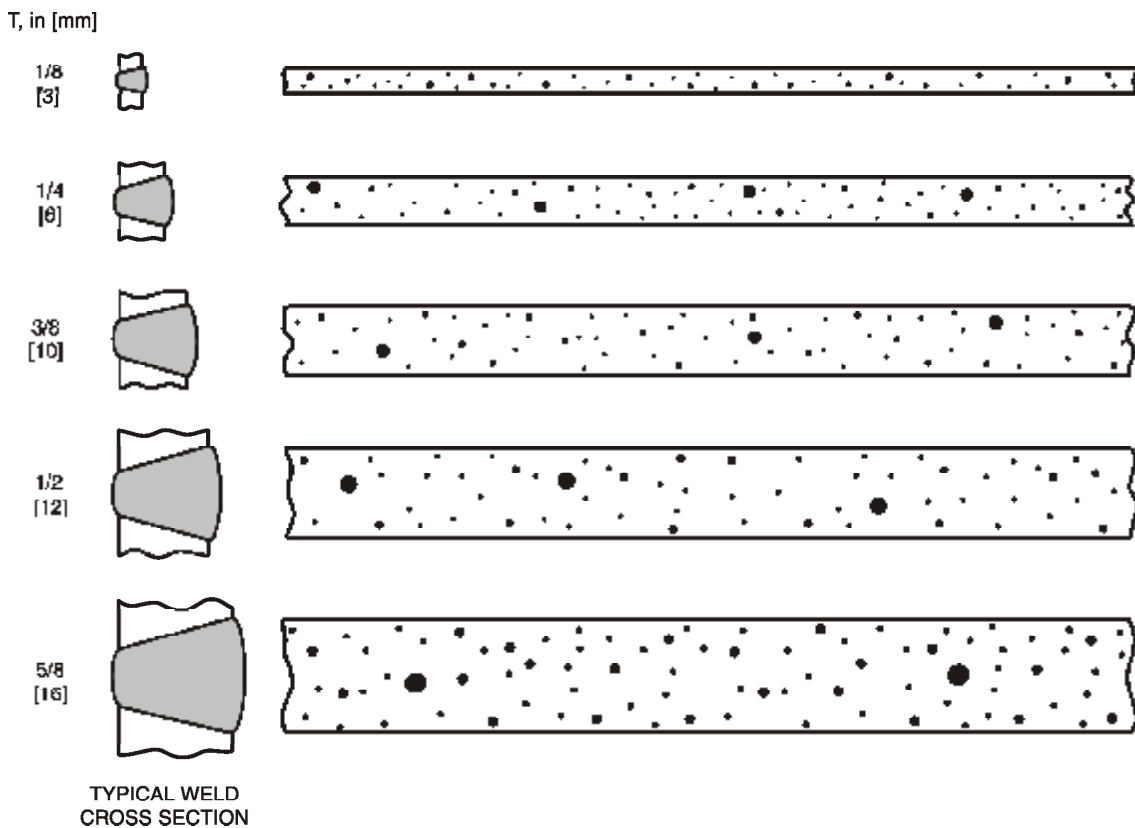
Figure 5.8—Maximum Acceptable Discontinuity RT Images (see 5.15.2.3)
