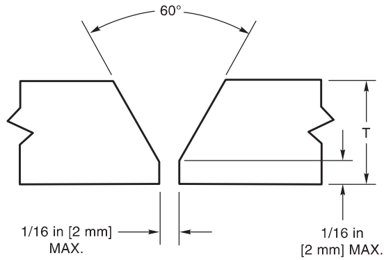
Figure 3.29—Tubular Groove Weld—Performance Qualification—Without Backing [see 3.19.3(2)]
