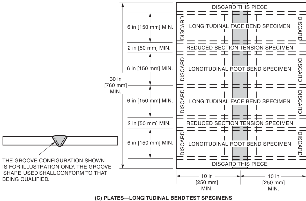
Figure 3.20—Location of Test Specimens for WPS Qualification—Plate (see 3.9.1 and 3.15.5.1)
