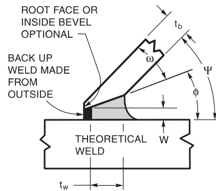
DETAIL C
