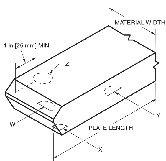
Figure 4.1—Edge Discontinuities in Cut Plate (see 4.12.7)
