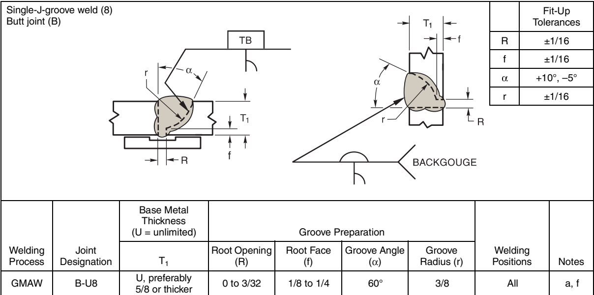
Figure B.1 (Continued)—Recommended CJP Groove Welded Joints (Inches)
