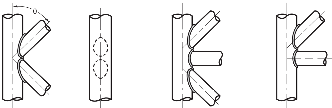
(E) K-CONNECTION
