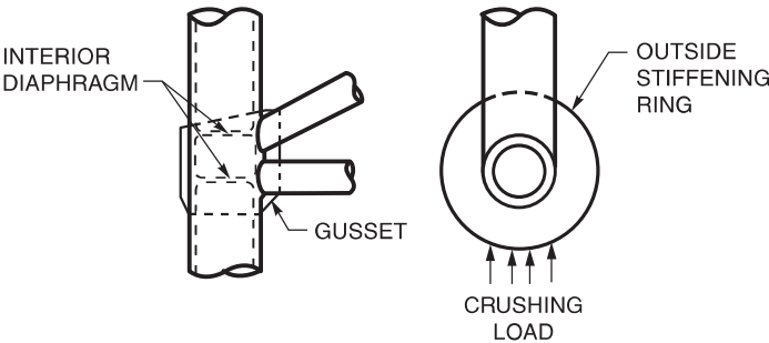
(J) EXAMPLES OF COMPLEX REINFORCED CONNECTIONS
