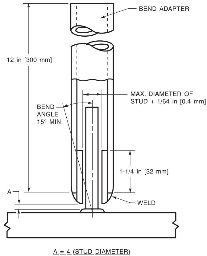
Figure 6.1—Stud Weld Bend Jig (see 6.4.6.4)
