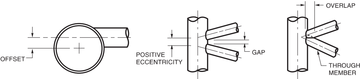
(H) DEVIATIONS FROM CONCENTRIC CONNECTIONS
