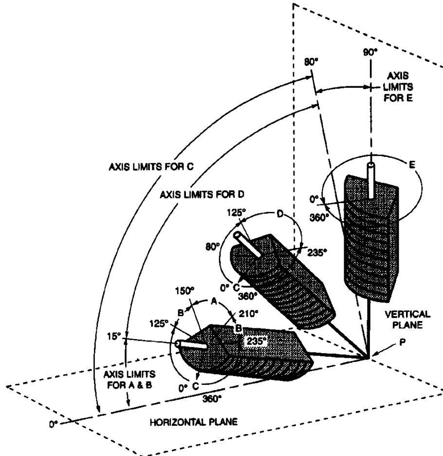
Figure 6.4—Positions of Fillet Welds (see 6.2.3)
