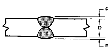
BUTT JOINT— EQUAL DIAMETER
