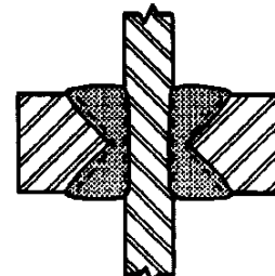
MACROETCH SPECIMEN OF WELDED JOINT
