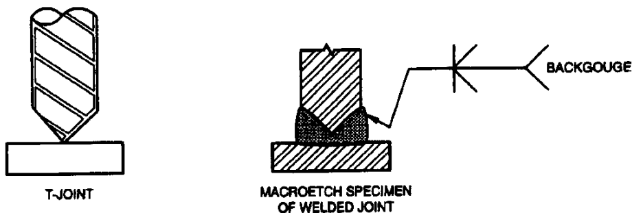
(C) COMPLETE JOINT PENETRATION GROOVE WELD—T-JOINT
