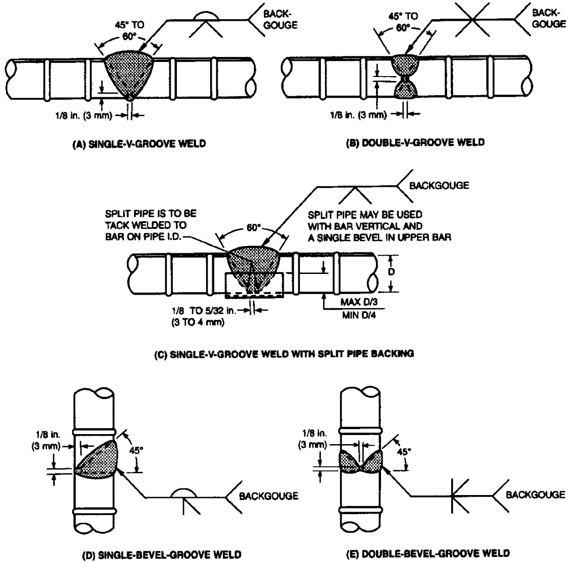
Figure 3.2—Direct Butt Joints (see Table 3.1)
