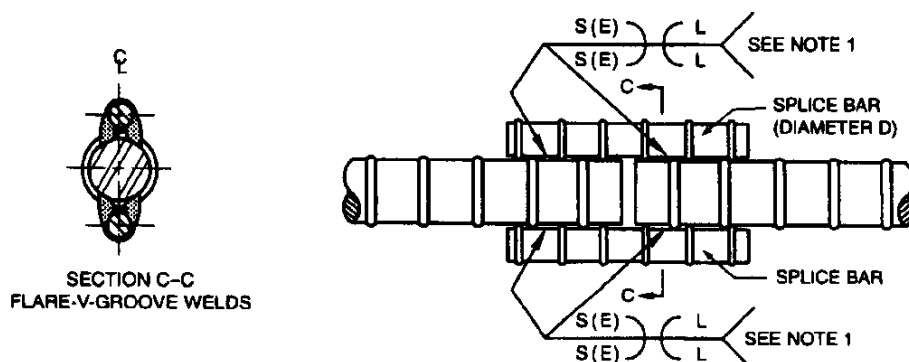
(C) INDIRECT BUTT JOINT TWO SPLICE BARS
