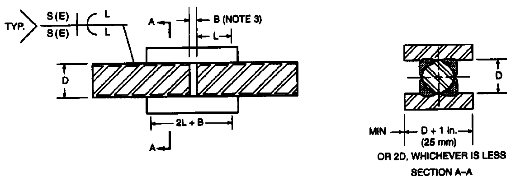
(B) FLARE-BEVEL-GROOVE—INDIRECT BUTT JOINT
