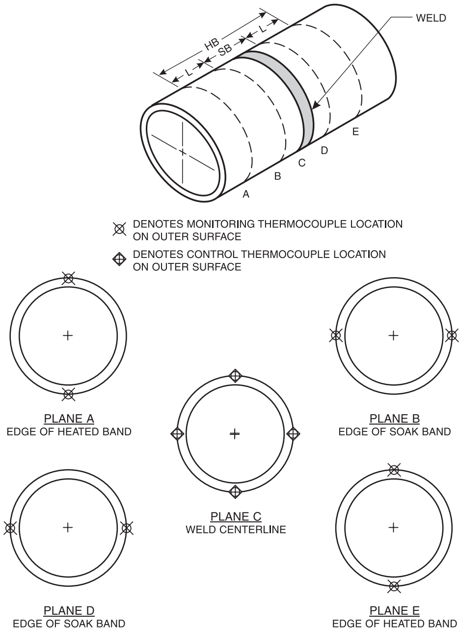
Figure 14—Minimum Number of Thermocouples (Monitoring and Control) Recommended for Local 360-Degree Band PWHT of a Butt Weld for Piping in the Horizontal Position with Pipe Sizes of 20 and up to 30 NPS (500 to 750 DN) and Four Control Zones
