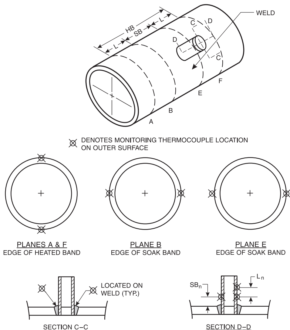
Figure 15—Minimum Number of Monitoring Thermocouples Recommended for a Branch, Nozzle, or Attachment When Heating in Accordance with Figures 6, 7, or 8
