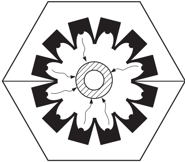
Figure 19—“Infrared Furnace” of Quartz Lamp Reflector Units Clam-Shelled or Assembled Around a Pipe
