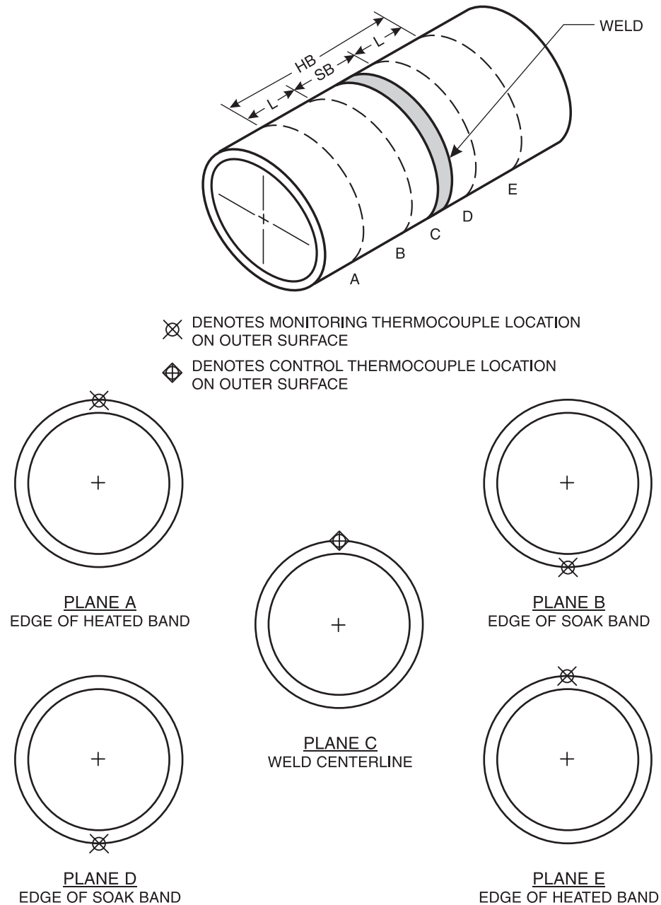
Figure 12—Minimum Number of Thermocouples (Monitoring and Control) Recommended for Local 360-Degree Band PWHT of a Butt Weld for Piping in the Horizontal Position with Pipe Size up to 6 NPS (150 DN) and One Control Zone
