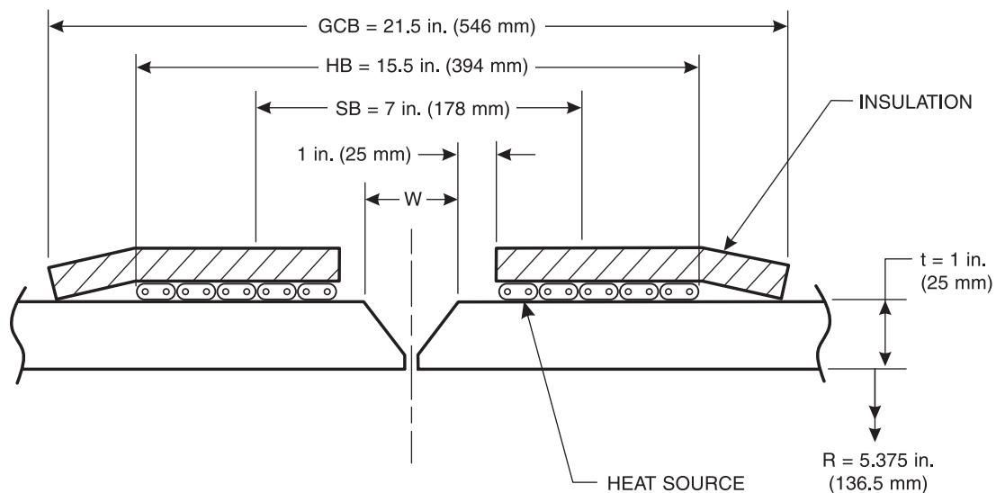
Figure 2—Example of Parameters for Local 360-Degree Band Bake-Out of a Butt Weld in a 12 NPS (300 DN), 1 in. (25 mm) Wall Thickness Pipe
