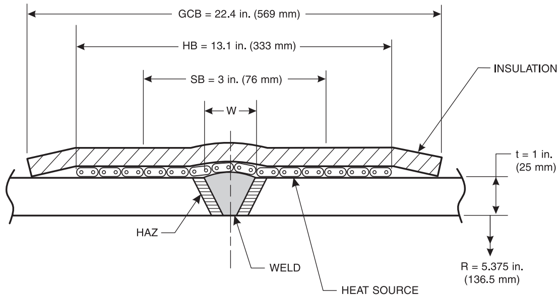
Figure 4—Example of Parameters for Local 360-Degree Band Postheating a Butt Weld in a 12 NPS (300 DN), 1 in. (25 mm) Wall Thickness Pipe
