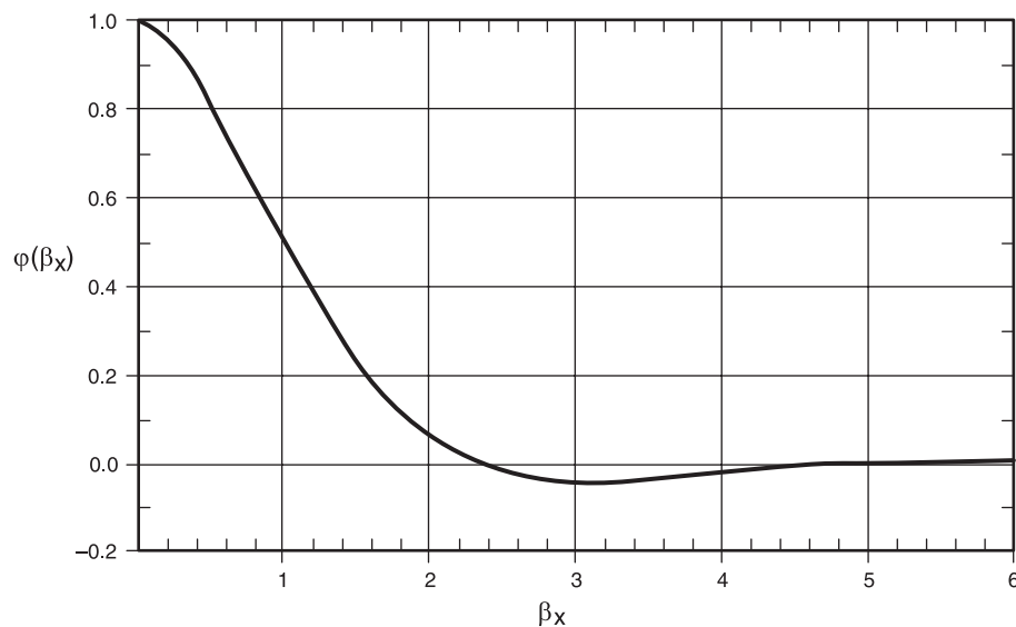
Figure B.1—Bending Stress Decay as a Function of \beta x , Where x is the Distance from the Edge of the Heater to the Centerline of the Weld
