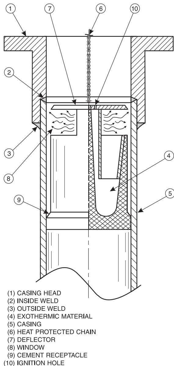
Figure 17—Schematic Depiction of Exothermic Heating of Weld Attaching a Slip-On Flange to a Well Casing
