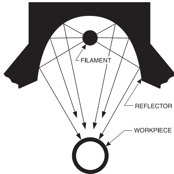
Figure 18—Relative Position of Quartz Filament, Reflector, and Workpiece
