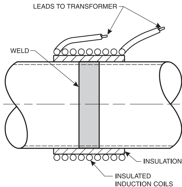
Figure 16—Schematic Depiction of Induction Coil Setup
