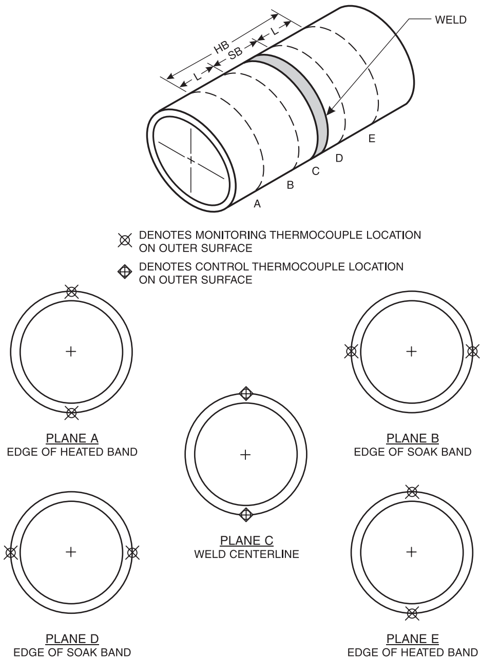
Figure 13—Minimum Number of Thermocouples (Monitoring and Control) Recommended for Local 360-Degree Band PWHT of a Butt Weld for Piping in the Horizontal Position with Pipe Sizes of 8 and up to 12 NPS (200 to 300 DN) and Two Control Zones
