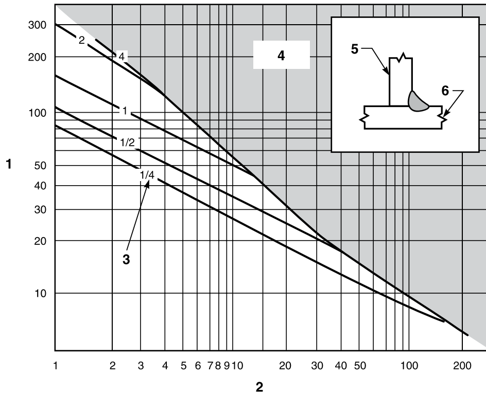
Figure 15a) — Single-pass SAW fillet welds with web and flange of same thickness
