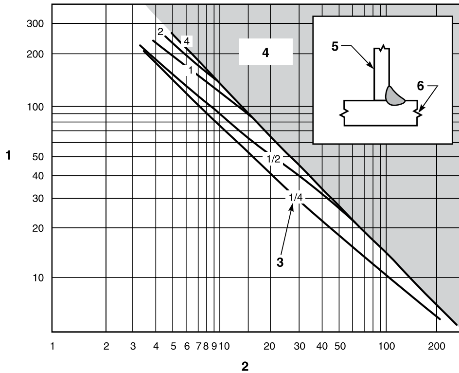
Figure 15e) — Single-pass SAW fillet welds with 2 in flanges and varying web thickness
