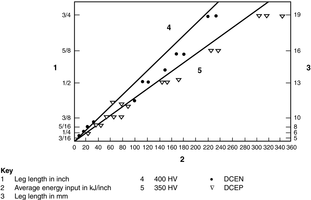
Figure 14b) — Submerged arc welding (SAW)
