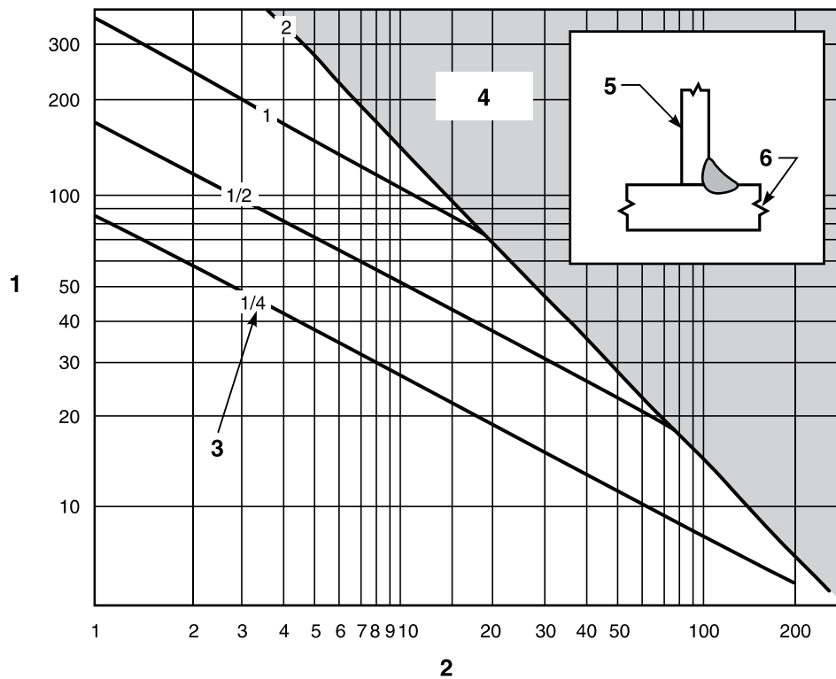
Figure 15b) — Single-pass SAW fillet welds with 1/4 in flanges and varying web thickness
