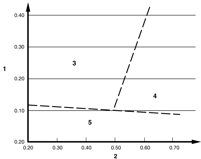
Figure 12 — Critical cooling rate for 350 HV and 400 HV
