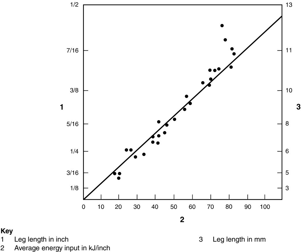
Figure 14a) — Shielded metal arc welding (SMAW)
