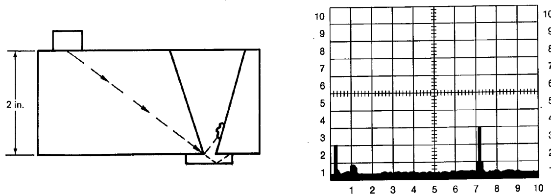
Fig. 23—Discontinuity
