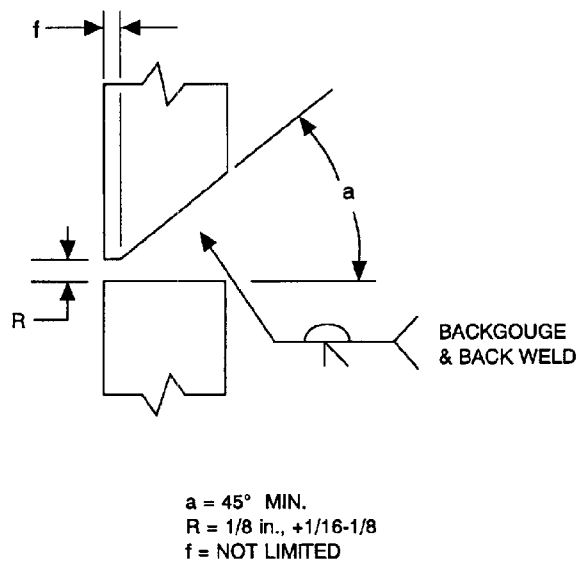
JOINT 8
