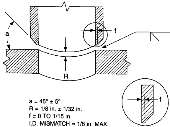
TYPICAL BRANCH CONNECTION
