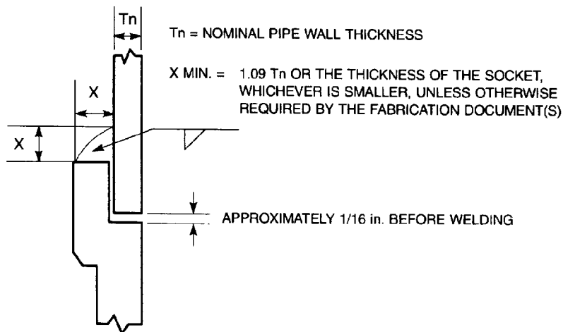
RECOMMENDED WELDING DIMENSIONS FOR SOCKET WELDING COMPONENTS OTHER THAN FLANGES
