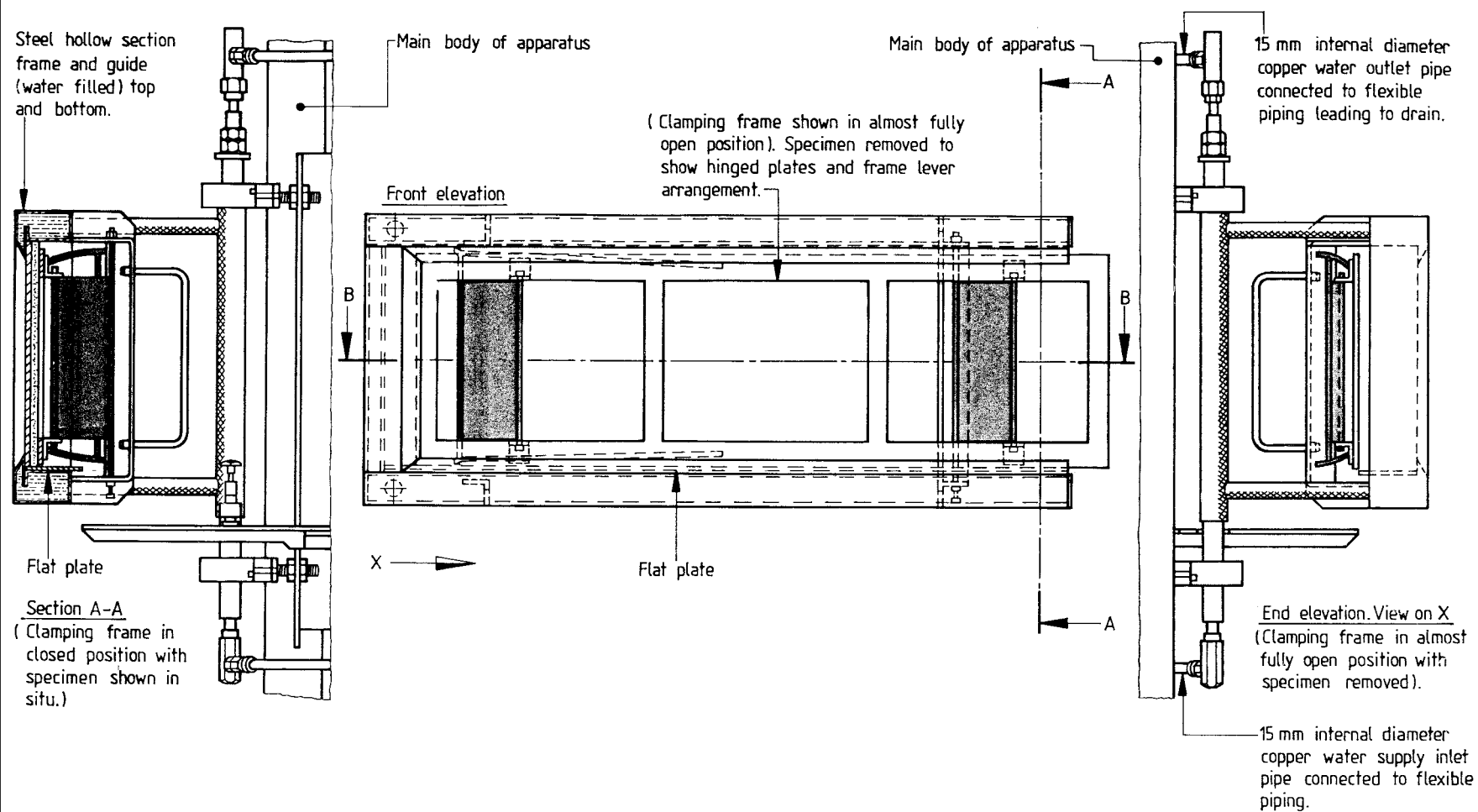
a) Elevation of specimen holder and vertical cross section
