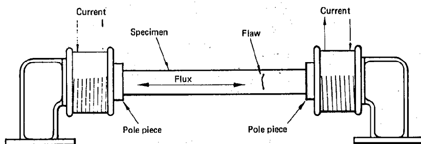
(a) Fixed bench with solenoid heads
