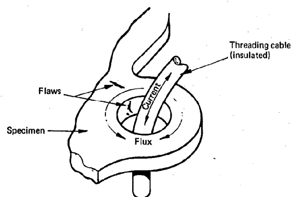
Figure 3. Flexible threading bar technique
