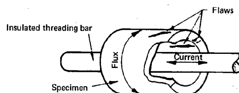
Figure 2. Threading bar or cable technique
