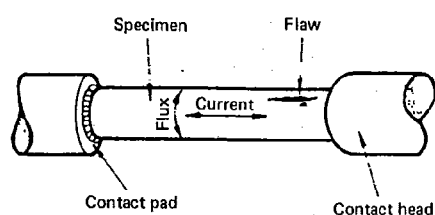
Figure 1. Current flow technique
