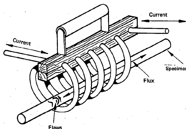
Figure 5. Coil technique
