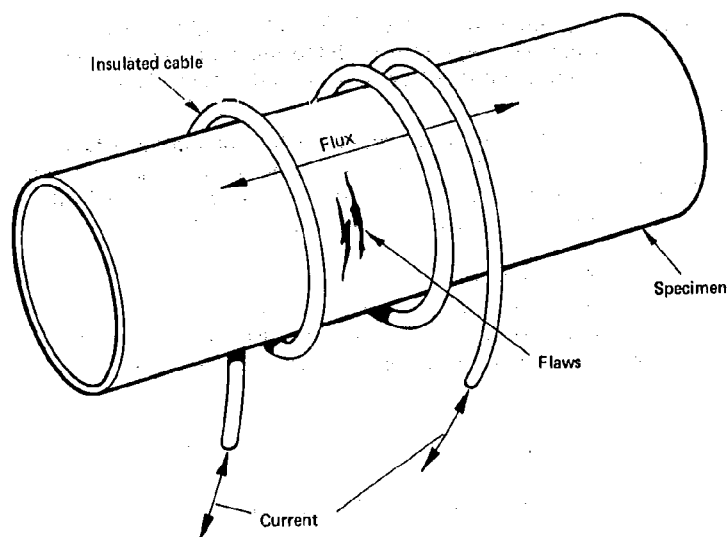
Figure 6. Flexible cable technique (using cable wound round the specimen)
