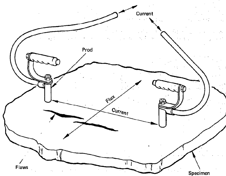
Figure 9. Current flow technique (prods)
