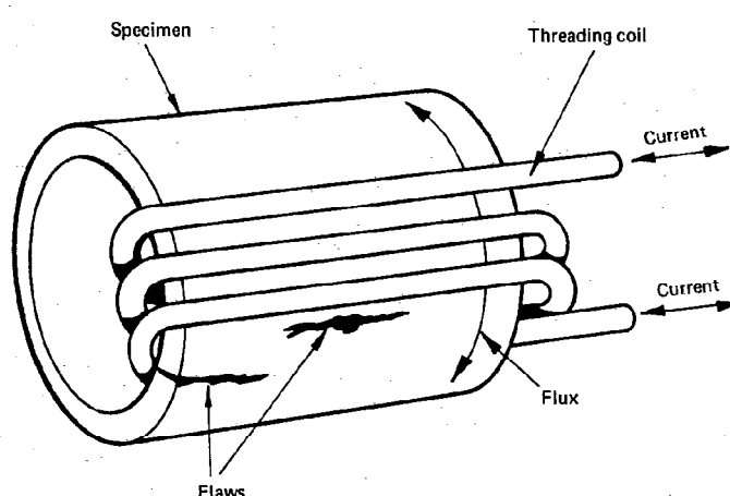
Figure 4. Flexible cable technique (using cable wound through the specimen)
