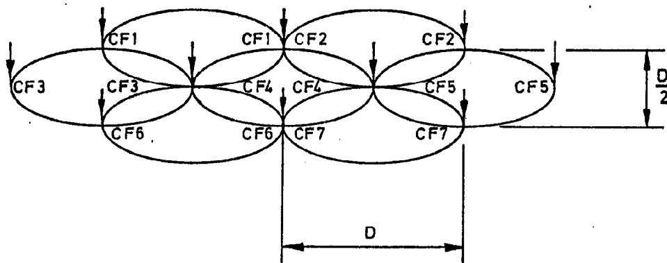
Figure 10. Search pattern which is acceptable when using current flow (prods) technique to inspect flat surfaces and those with radii of curvature greater than half the prod spacing (peak current value not less than 7500 amps per metre of prod spacing)
