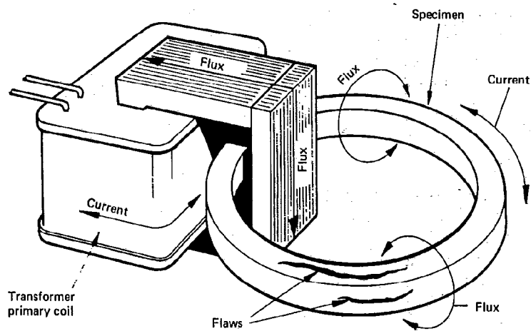
Figure 8. Induced current flow technique
