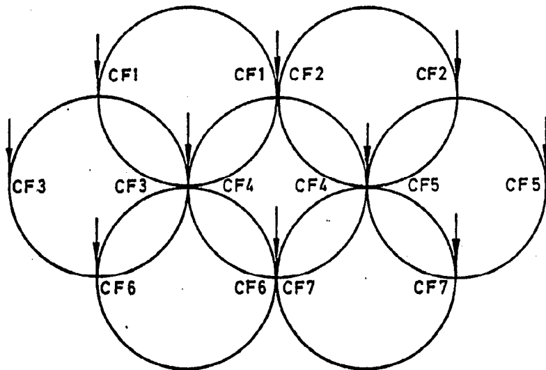
Figure 10. Search pattern which is acceptable when using current flow (prods) technique to inspect flat surfaces and those with radii of curvature greater than half the prod spacing (peak current value not less than 7500 amps per metre of prod spacing)
