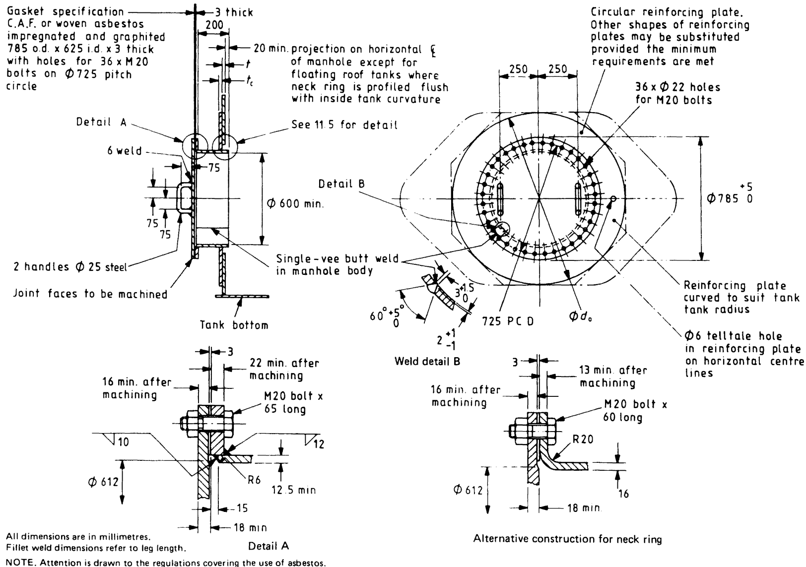
Figure 9 — Shell manholes (see 11.1)
