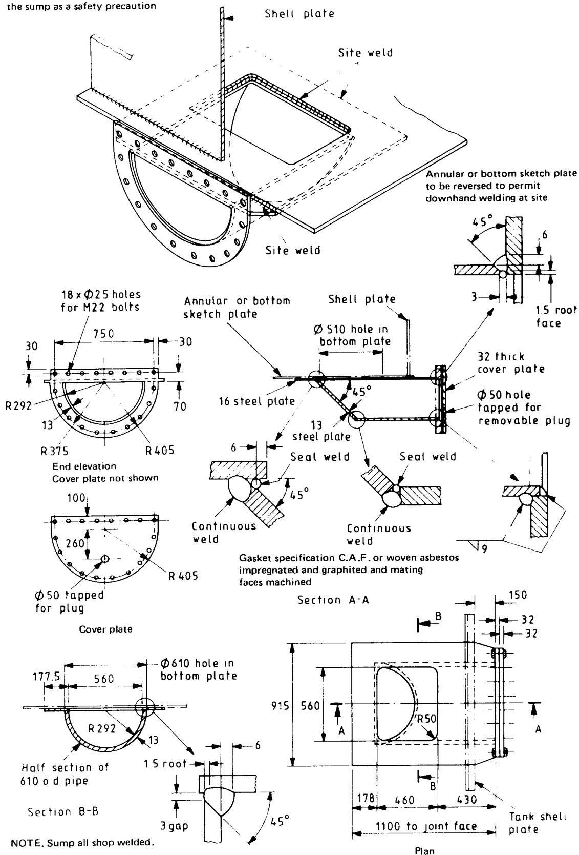
Figure 32 — Combined water draw-off and clean-out sump (see 11.14.3)
