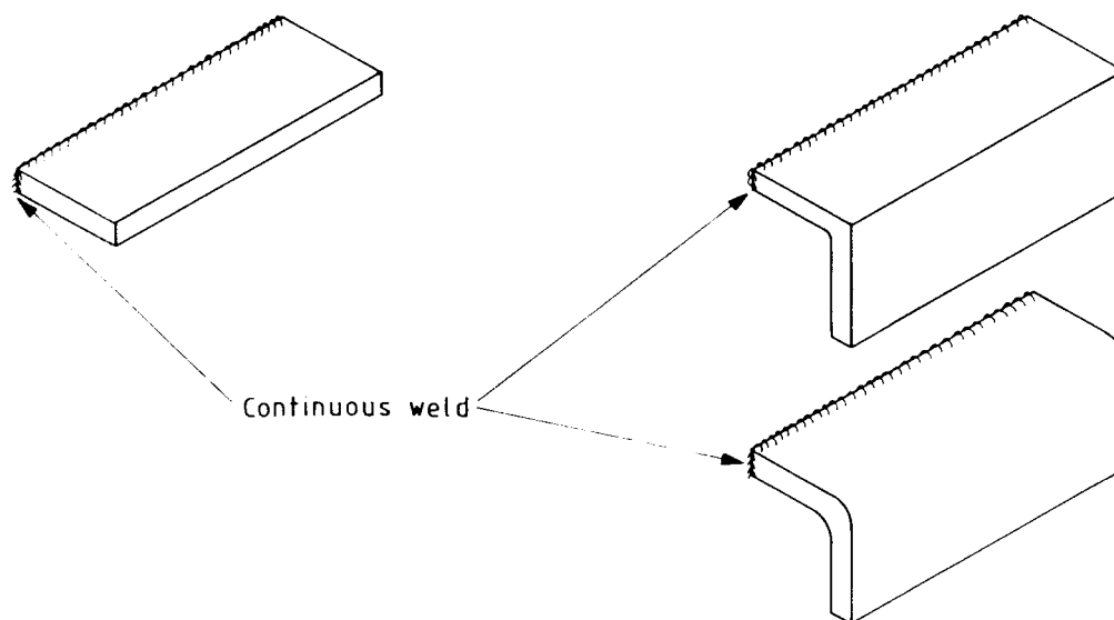
Figure 37 — Angle section and plate supports [see B.3.2 b)]
