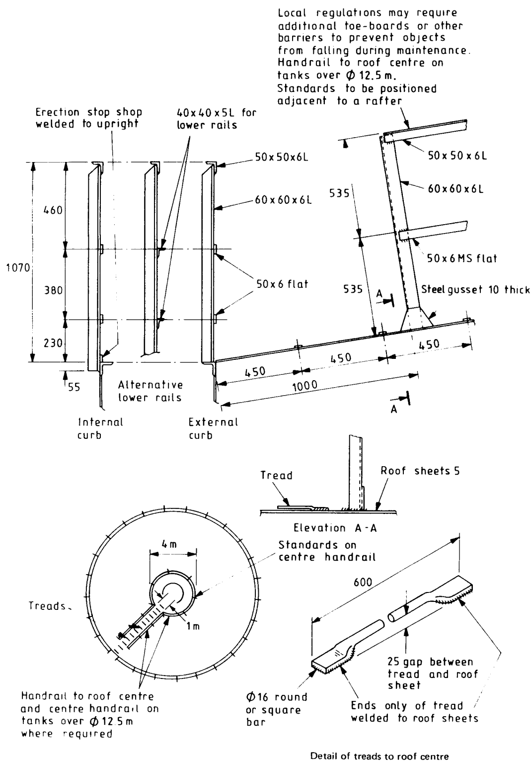
Figure 26 — Handrailing (see 11.11)
