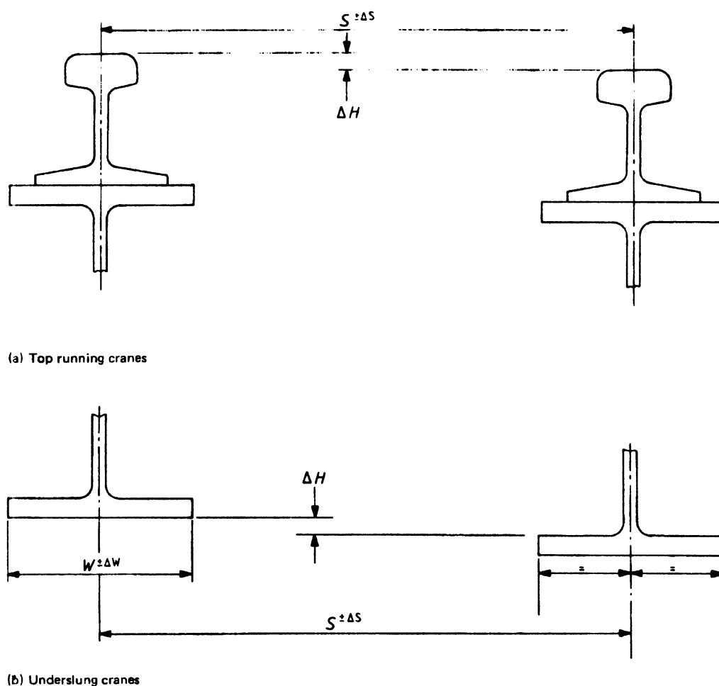
Figure 4 — Tolerances on crane tracks
