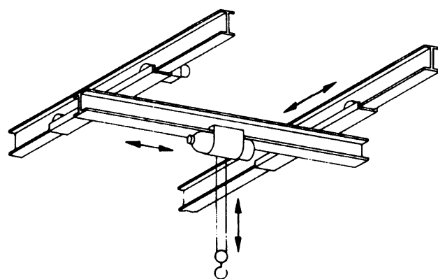
(a) Underslung crane (single girder)
