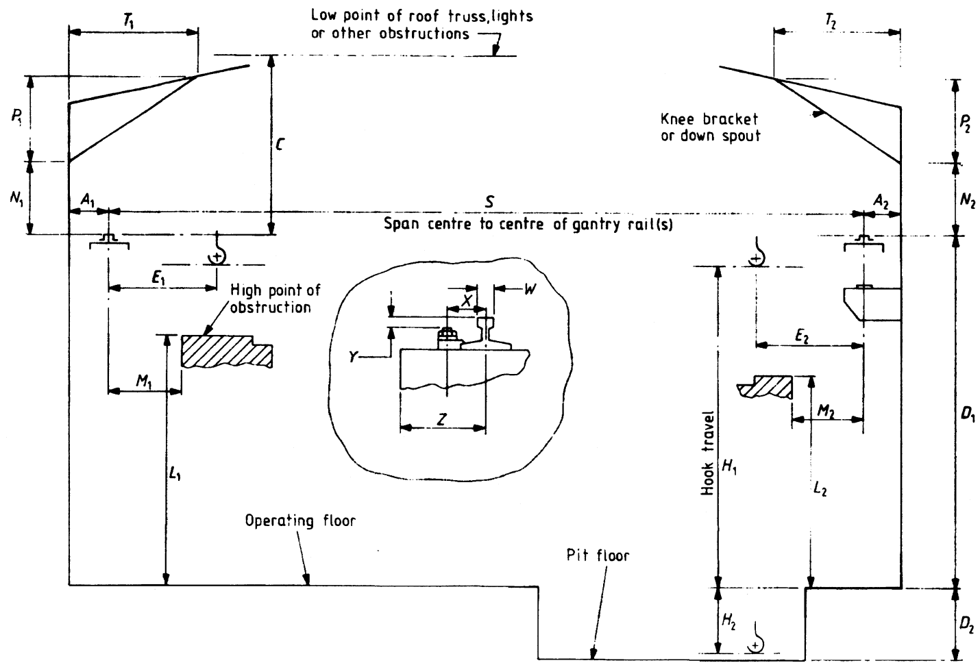
Figure 3 — Crane clearance dimensions
