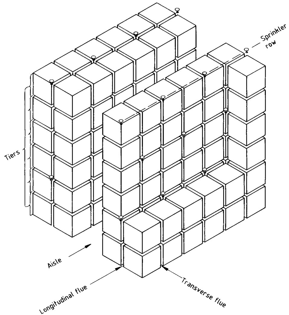
Figure 40 — Terminology for type S5 storage (beam pallet racking)
