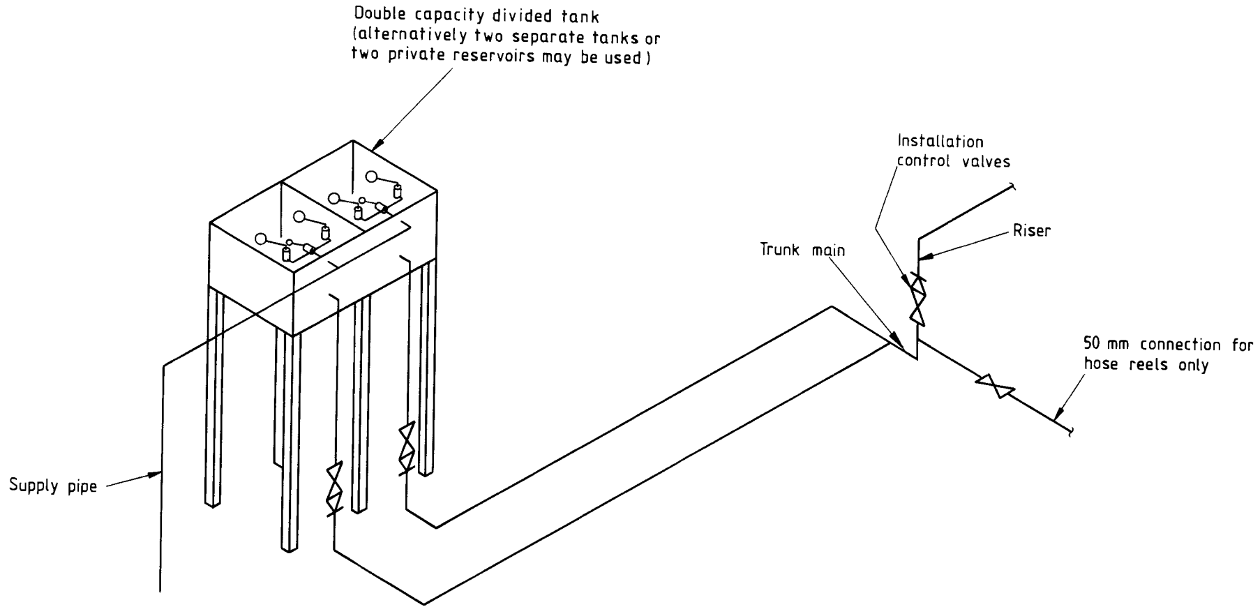
Figure 15 — Duplicate supplies using two gravity tanks
