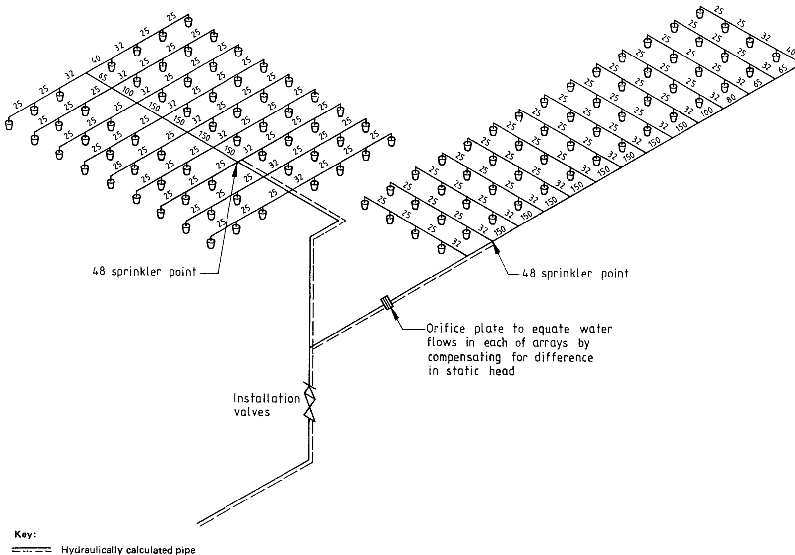
Figure 31 — Example of application of design points in a high-hazard installation with pipework sized from Table 60 and Table 63
