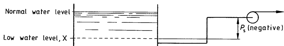
Figure 21 — Measurement of negative suction head
