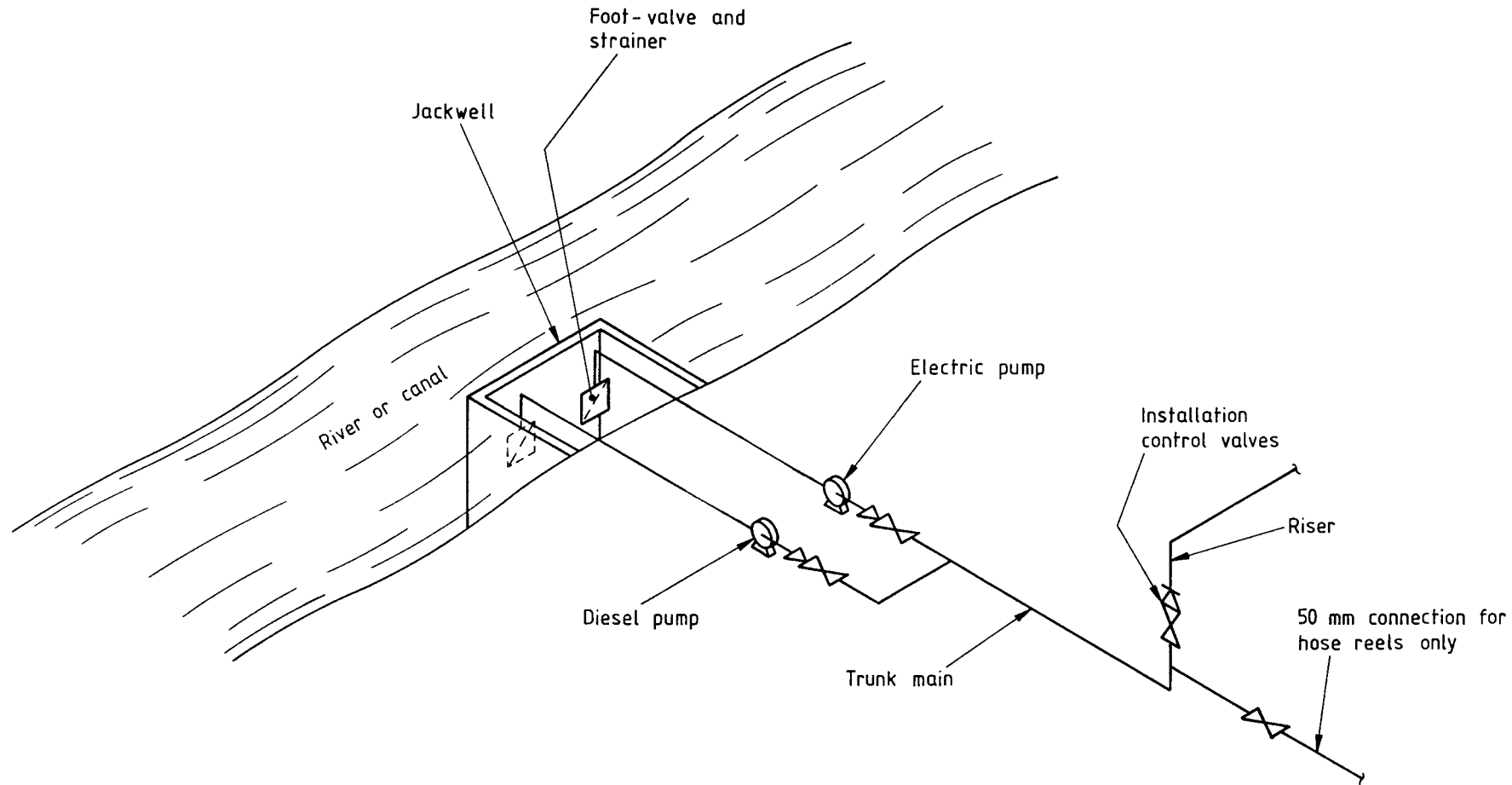
Figure 17 — Duplicate supplies using two suction pumps from river or canal (suction lift condition)
