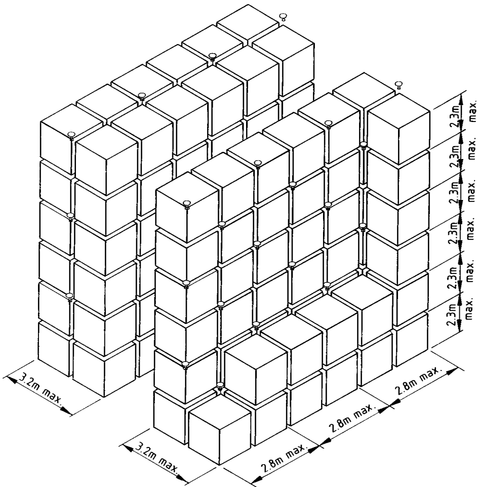
Figure 43 — Sprinkler locations for type S5 storage, category IV goods (beam pallet racking)
