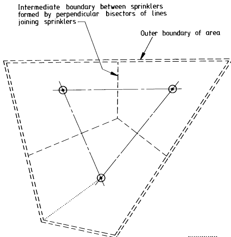
Figure 33 — Area covered by individual sprinklers where less than four sprinklers are in open communication
