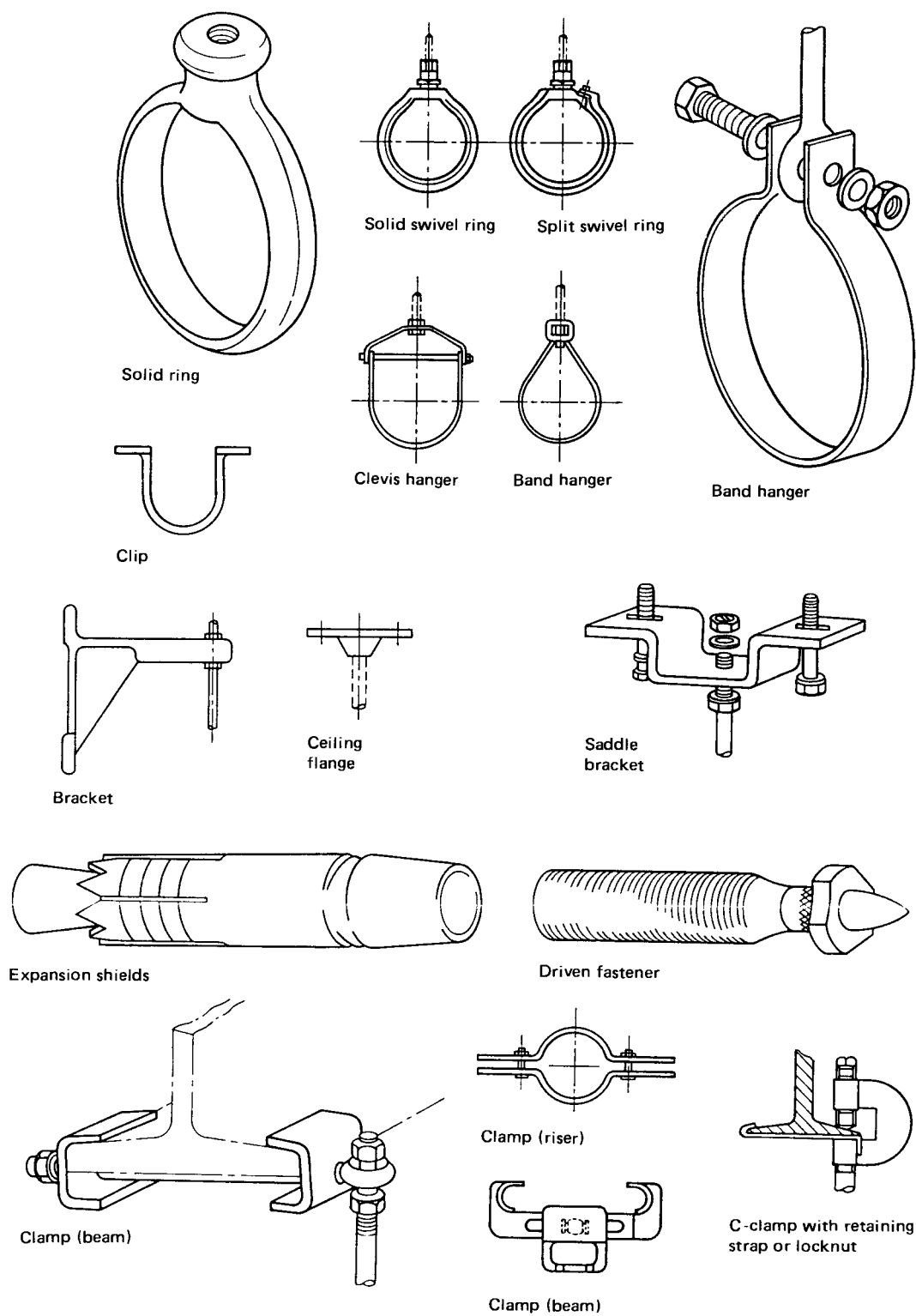
Figure 27 — Some common types of pipe hanger equipment
