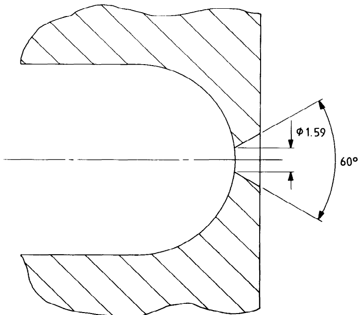
Figure 7. Type B nozzle
