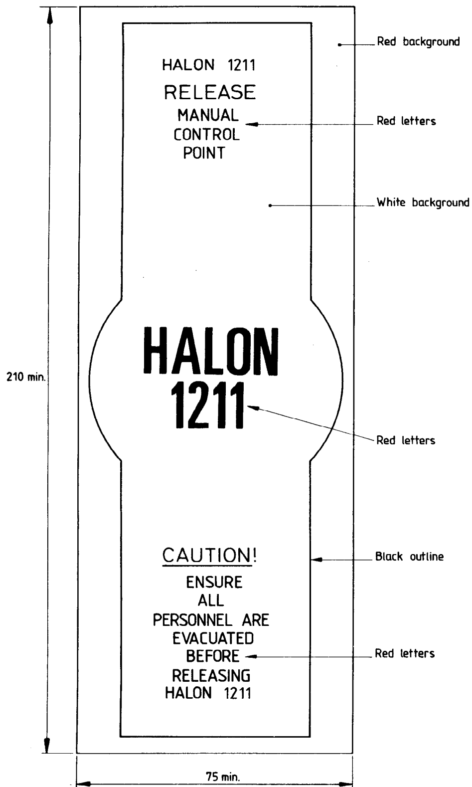
Figure 12. Label to be displayed at manual control
