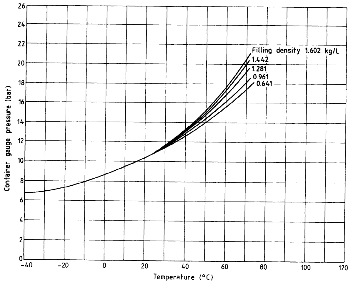
Figure 2. Isometric diagram of Halon 1211 pressurized to 10.5 bar at 21°C
