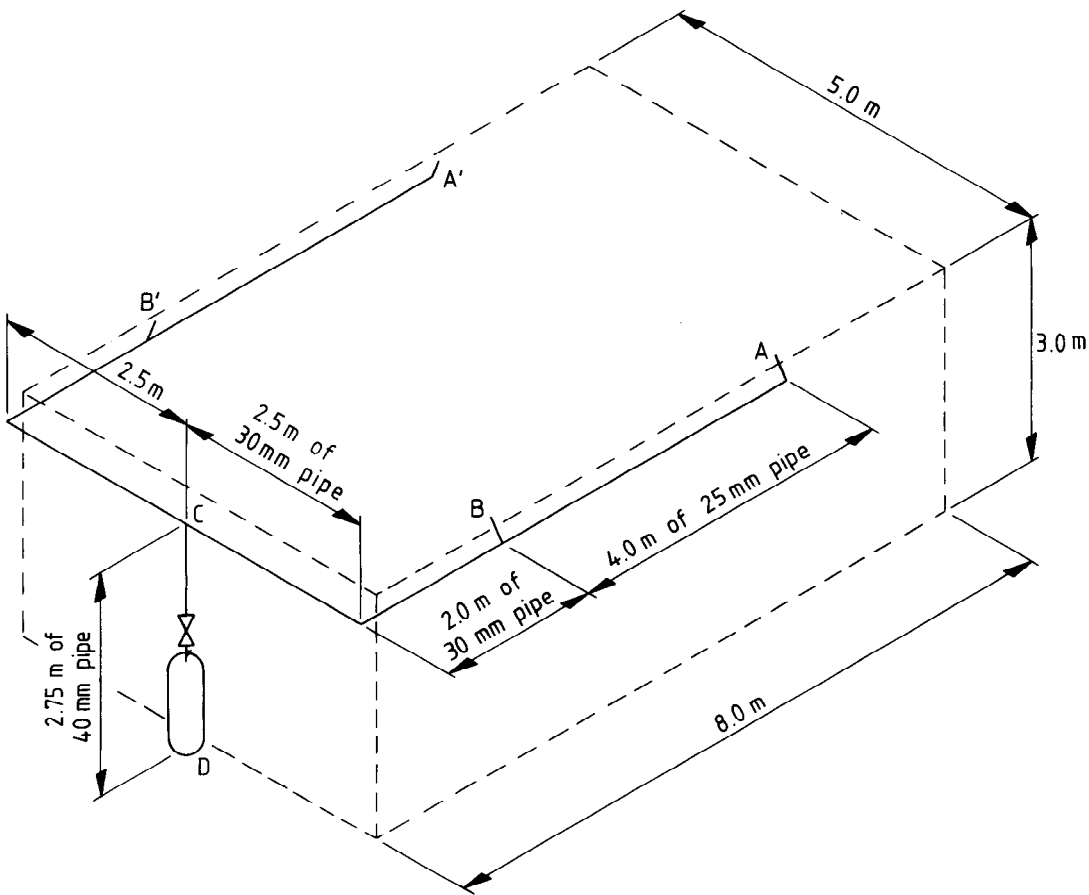
Figure 8. Example of balanced system
