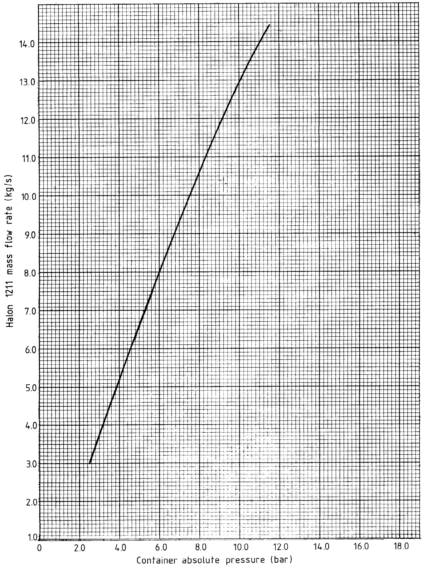
Figure 11. Example of Halon 1211 mass flow rate against container pressure for unbalanced system
