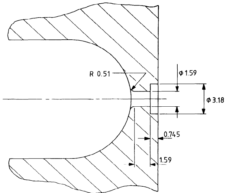
Figure 6. Type A nozzle
