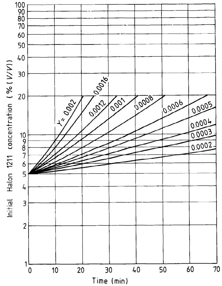
Figure 16. Initial amounts of Halon 1211 to produce a 5 % (V/V) residual concentration in enclosures equipped for mechanical mixing
