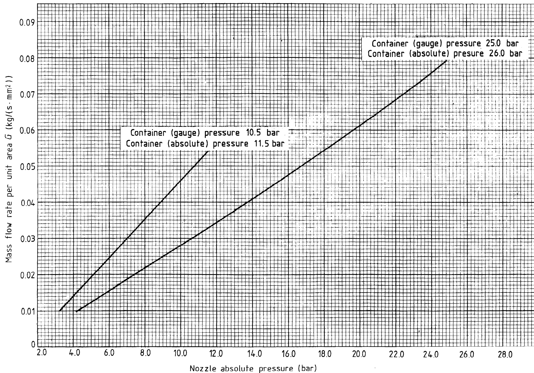
Figure 4. Mass flow rate per unit area against nozzle pressure with Halon 1211/N 2 for nozzle type A
