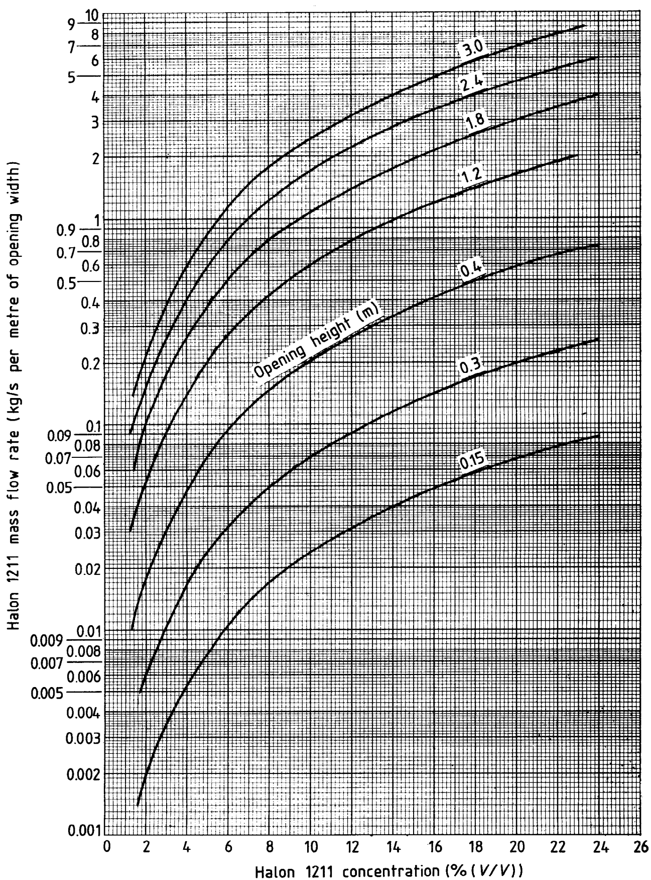
Figure 14. Extended mass flow rate of Halon 1211 to maintain constant concentration in enclosures with openings
