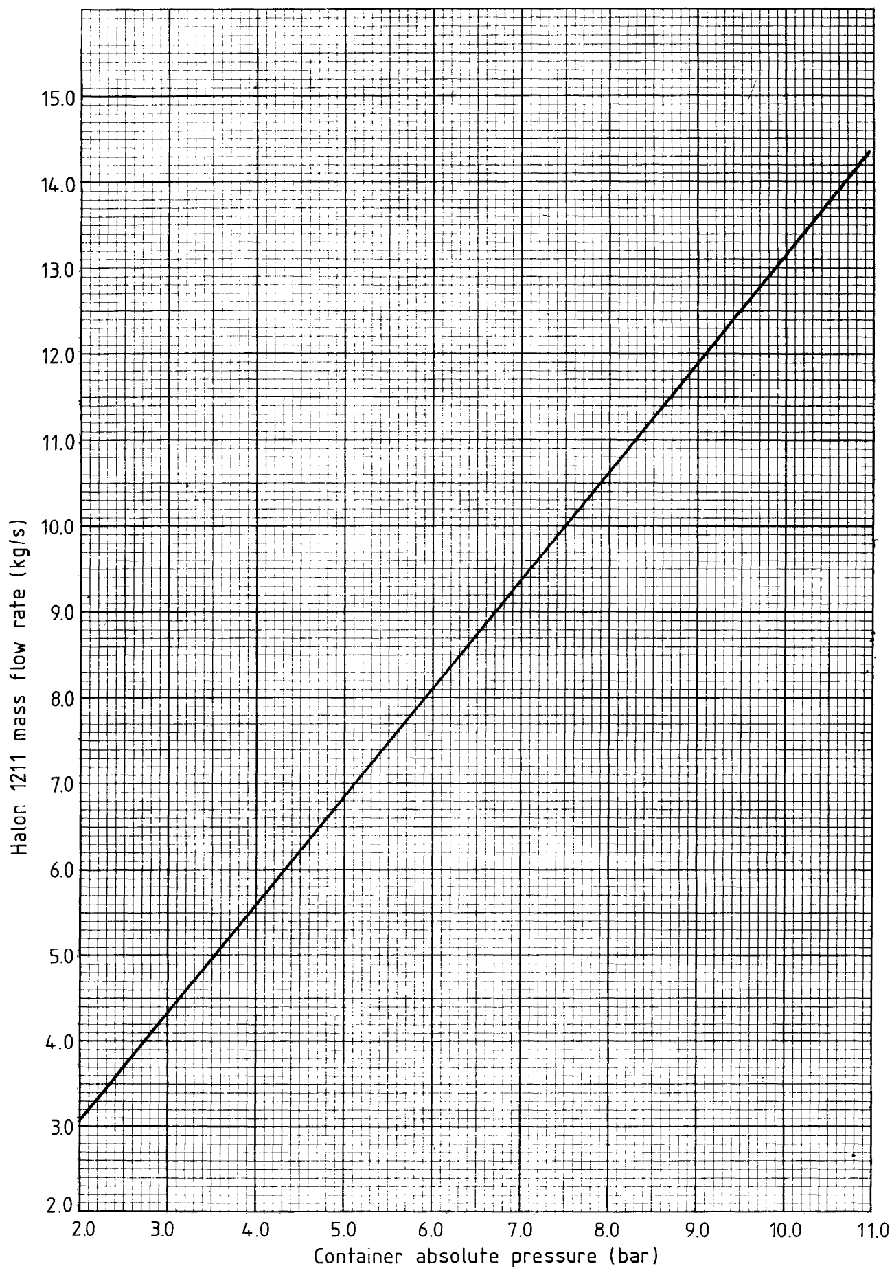
Figure 9. Example of Halon 1211 mass flow rate against container pressure for balanced system
