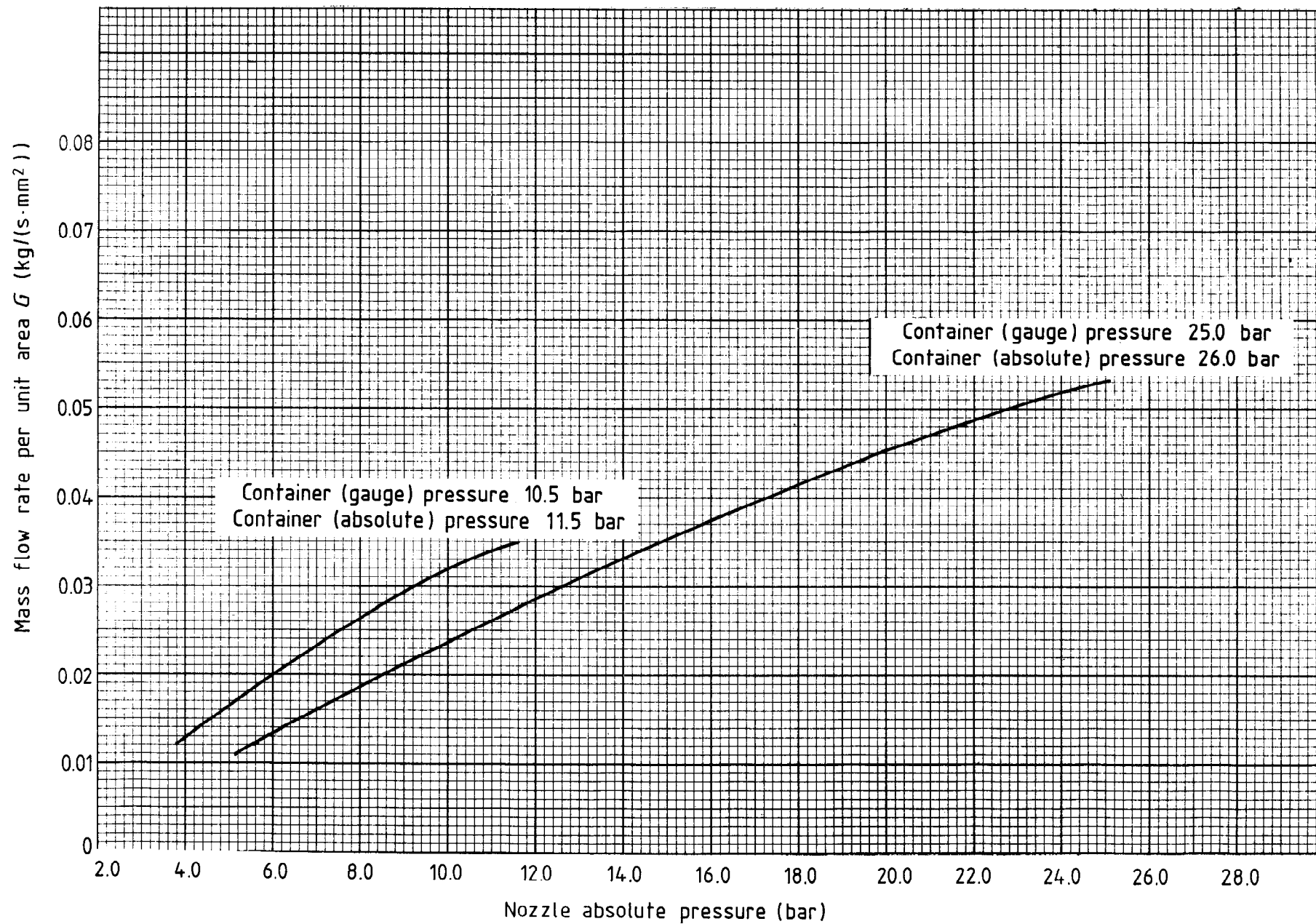
Figure 5. Mass flow rate per unit area against nozzle pressure with Halon 1211/ \text{N}_2 for nozzle type B
