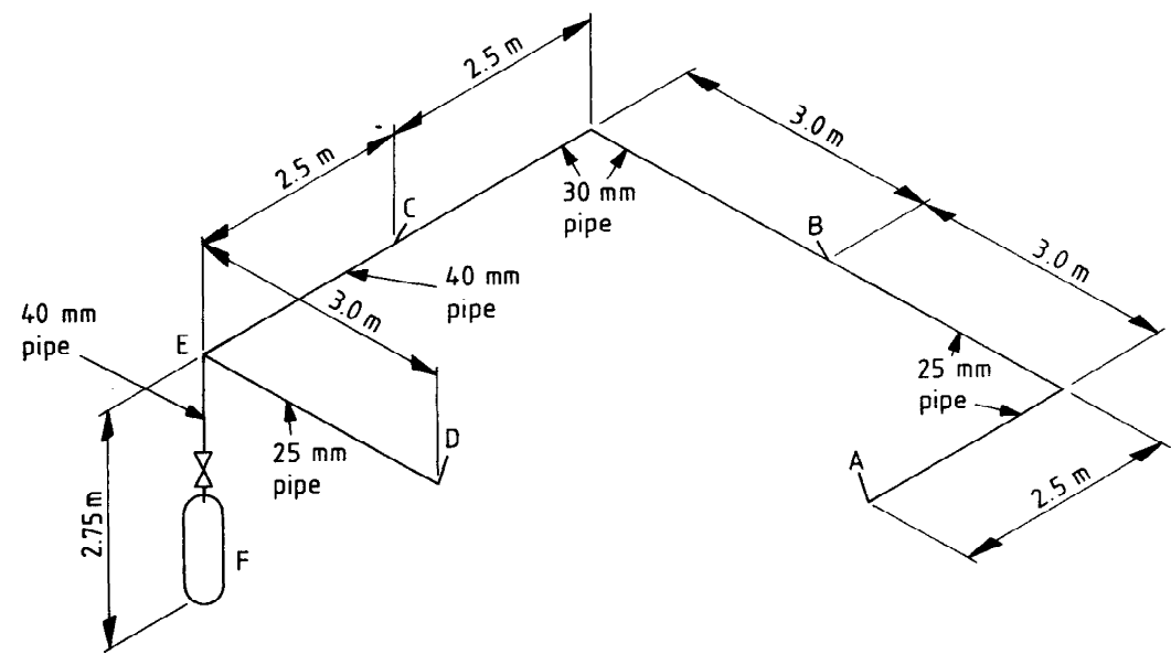
Figure 10. Example of unbalanced system
