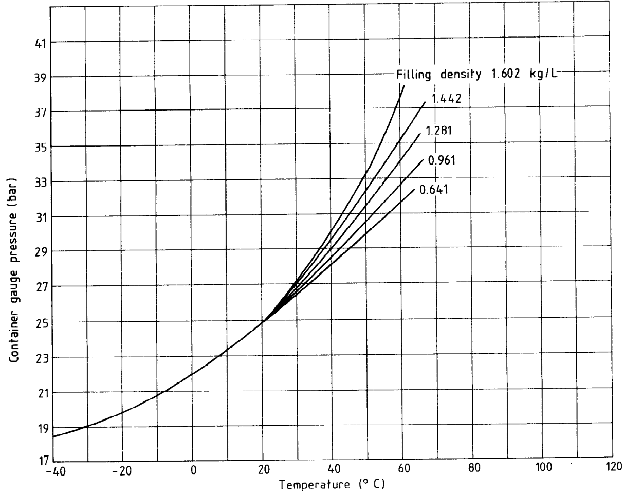
Figure 1. Isometric diagram of Halon 1211 pressurized to 25 bar at 21 °C
