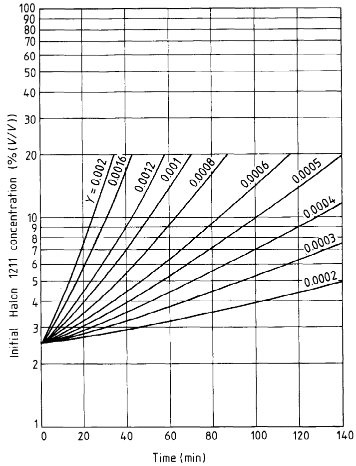
Figure 15. Initial amounts of Halon 1211 to produce a 2.5 % (V/V) residual concentration in enclosures equipped for mechanical mixing
