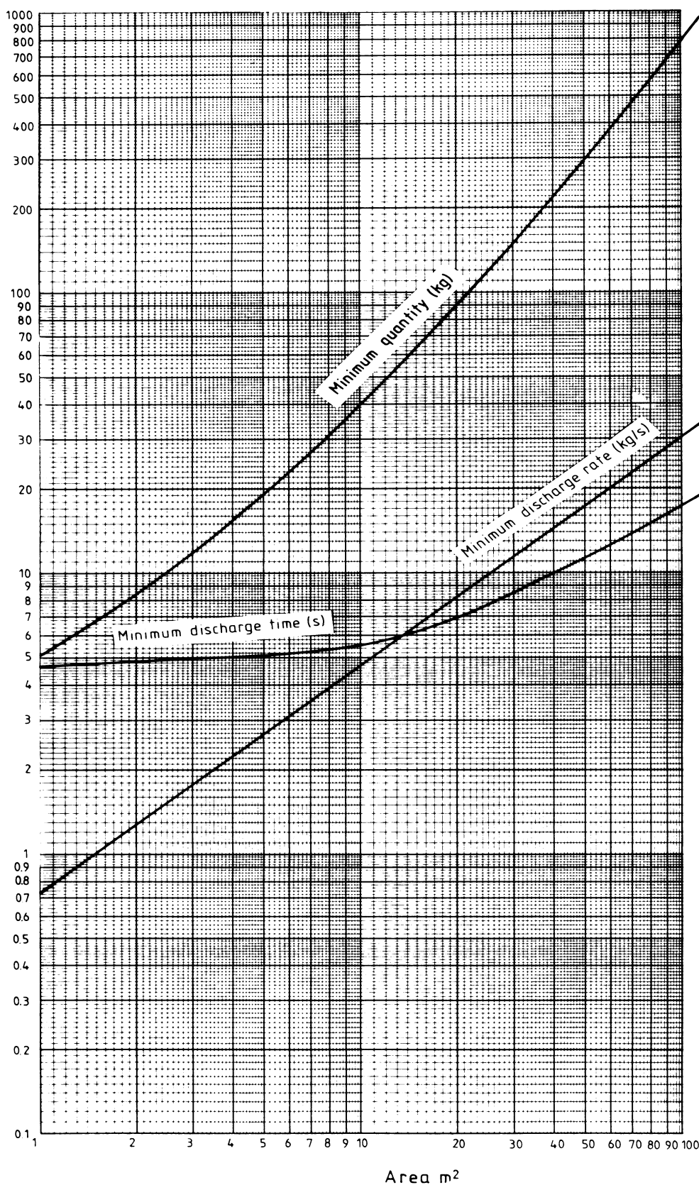
Figure 6 — Local application minimum design conditions for tankside nozzles with sodium bicarbonate; outdoors (see clause 19)
