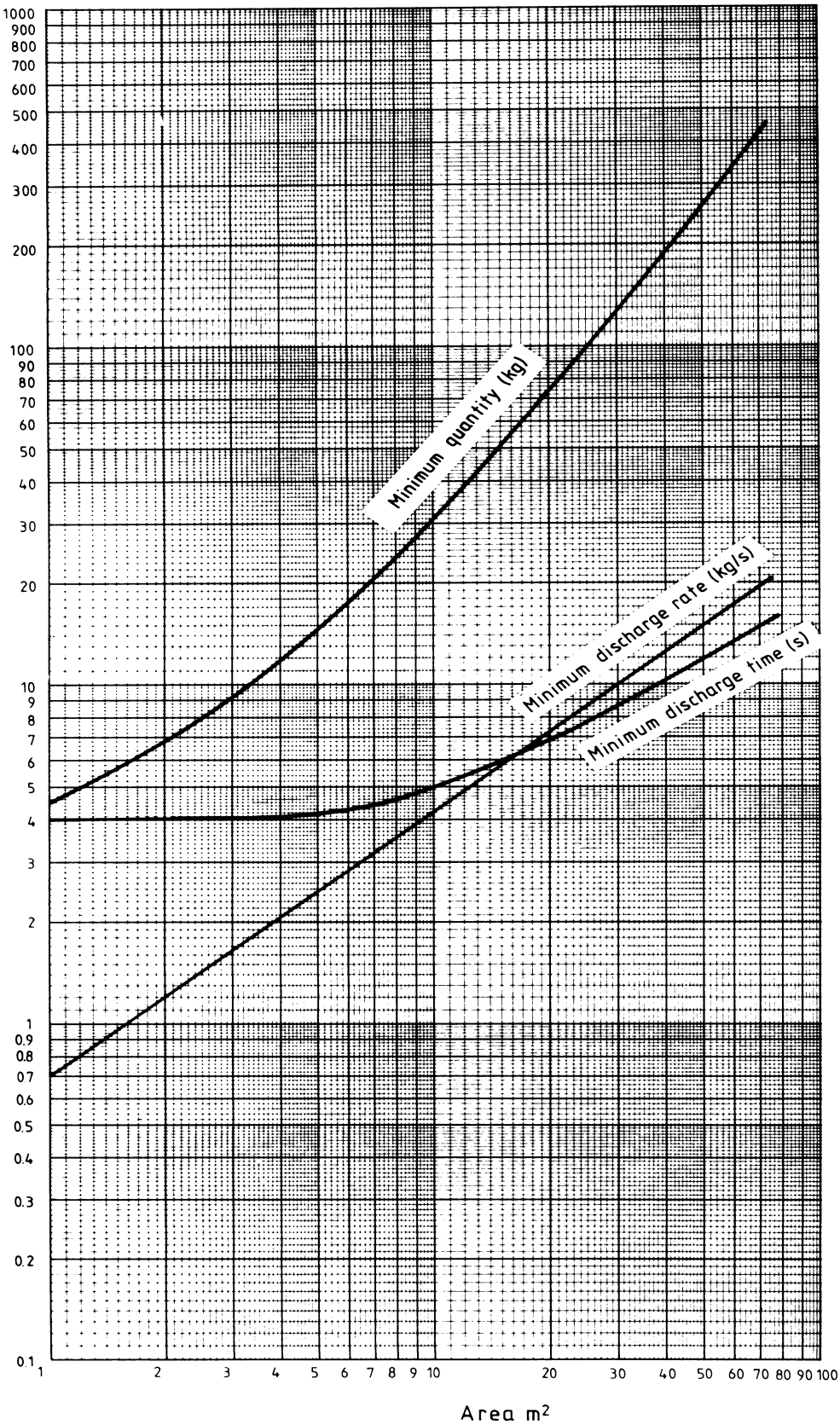
Figure 12 — Local application minimum design conditions for overhead nozzles with potassium bicarbonate; outdoors (see clause 19)
