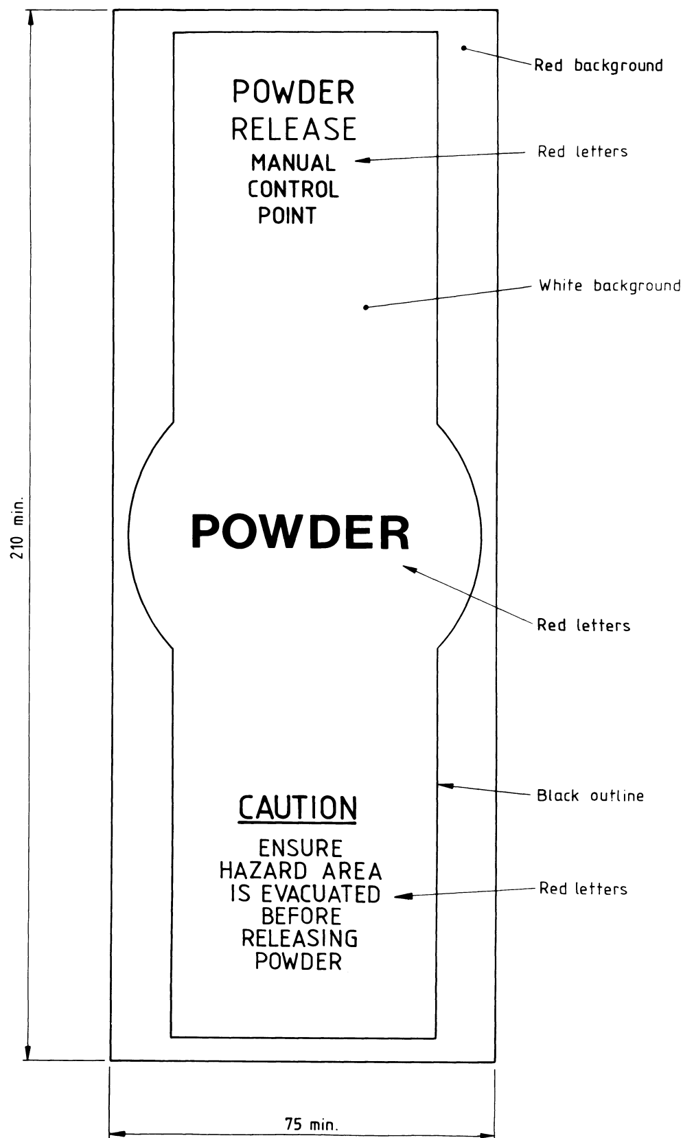
Figure 13 — Label for display at manual control (see 29.1.5)
