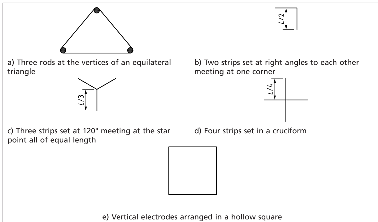
Figure 15 Miscellaneous electrode configurations
