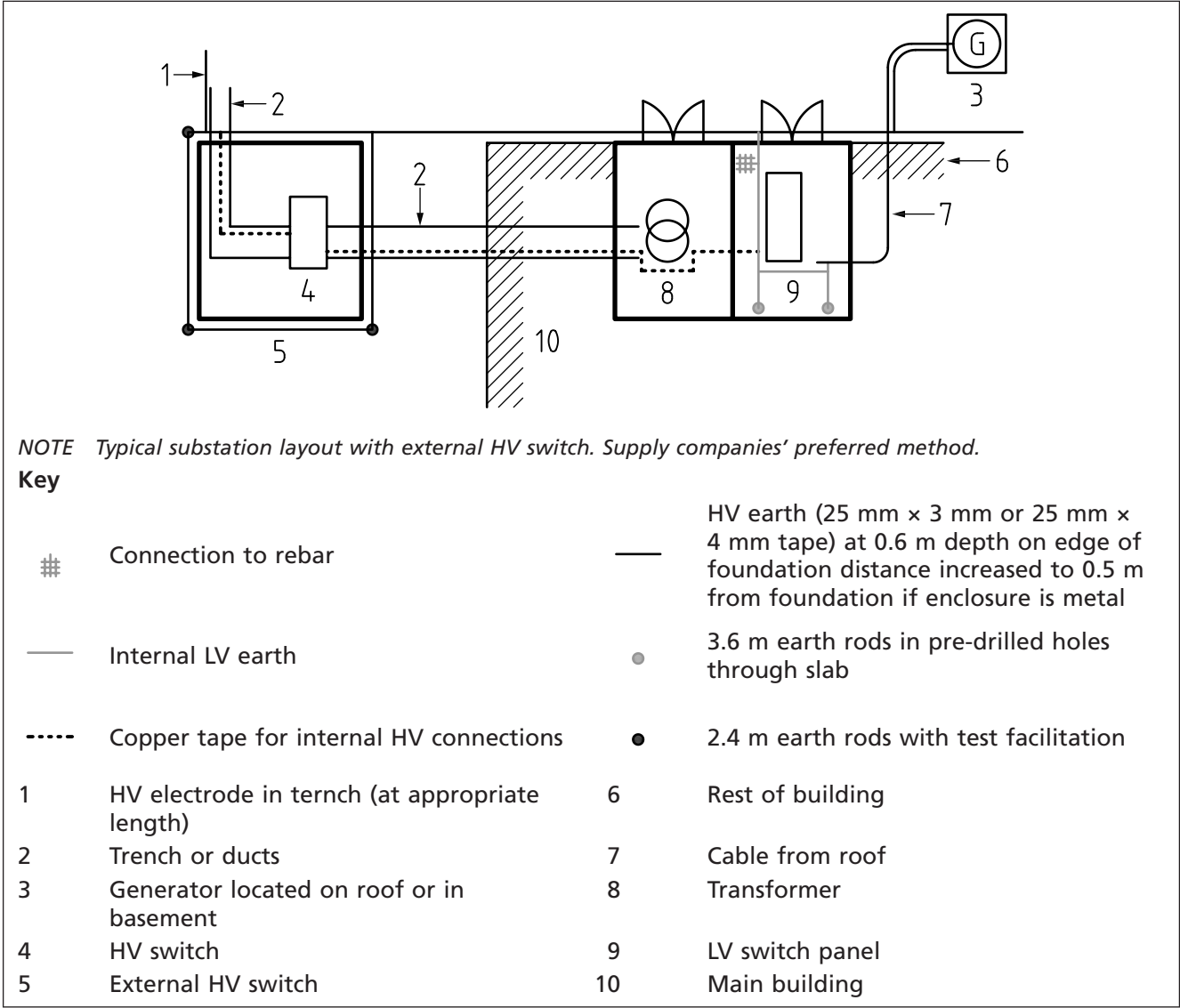
Figure A.4 External HV switch supply
