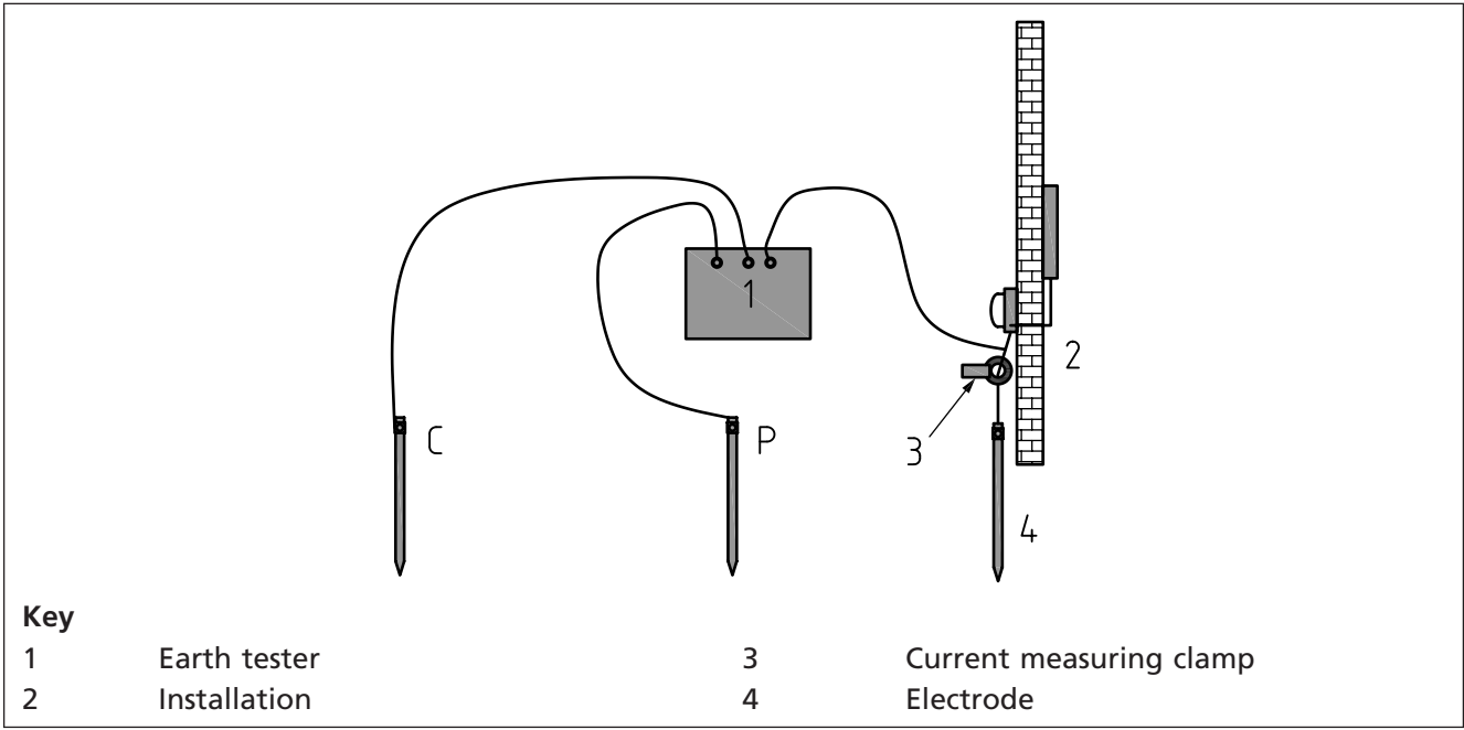
Figure 24 3-terminal tester with CT clamp
