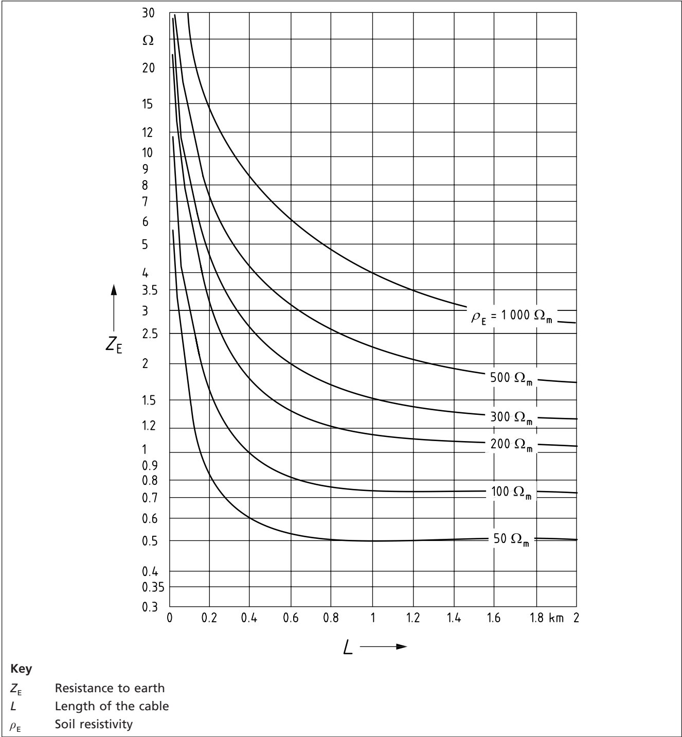
Figure 14 Impedence to earth of horizontal earth electrodes buried in homogeneous soil
