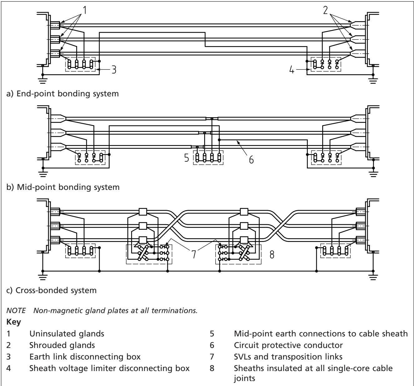
Figure 17 Simplified illustration of single-core cable sheath bonding systems
