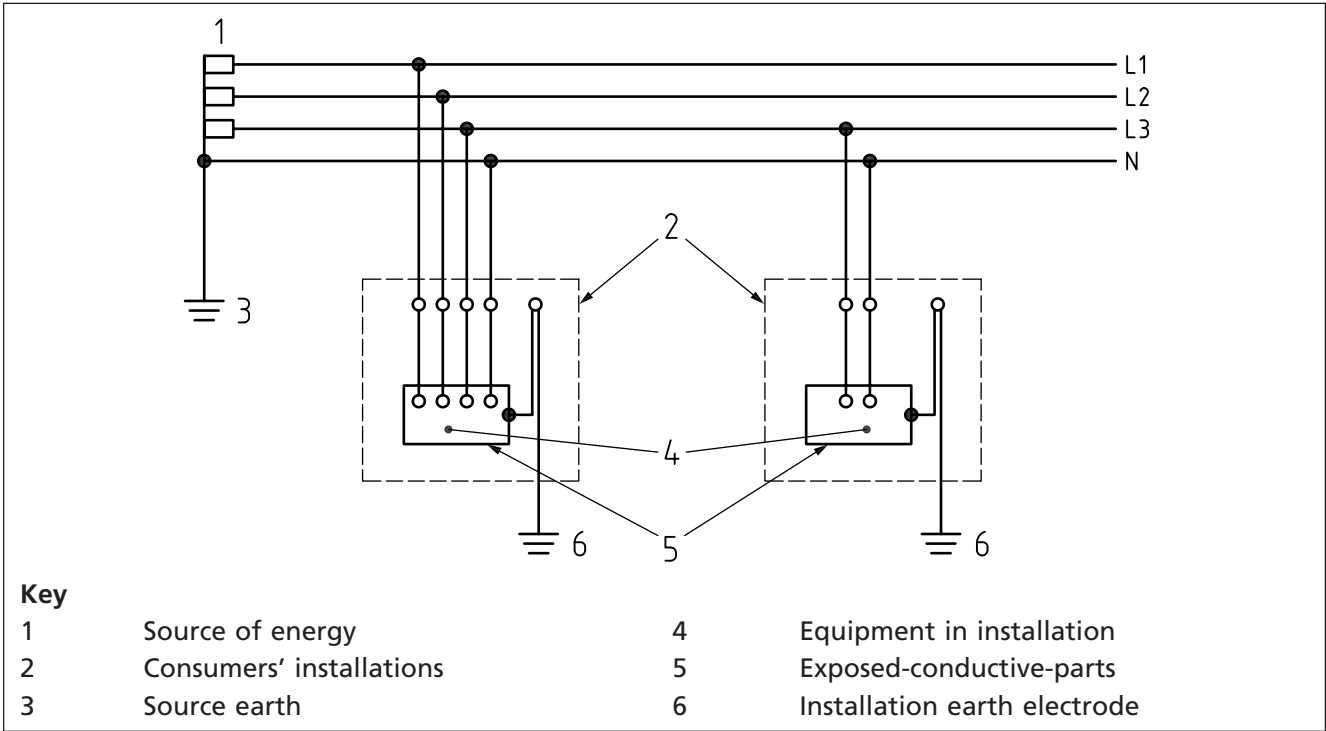
Figure 4 TT system
