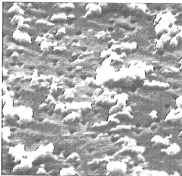
Fig. 1b — E5356 fume (20,000X)
