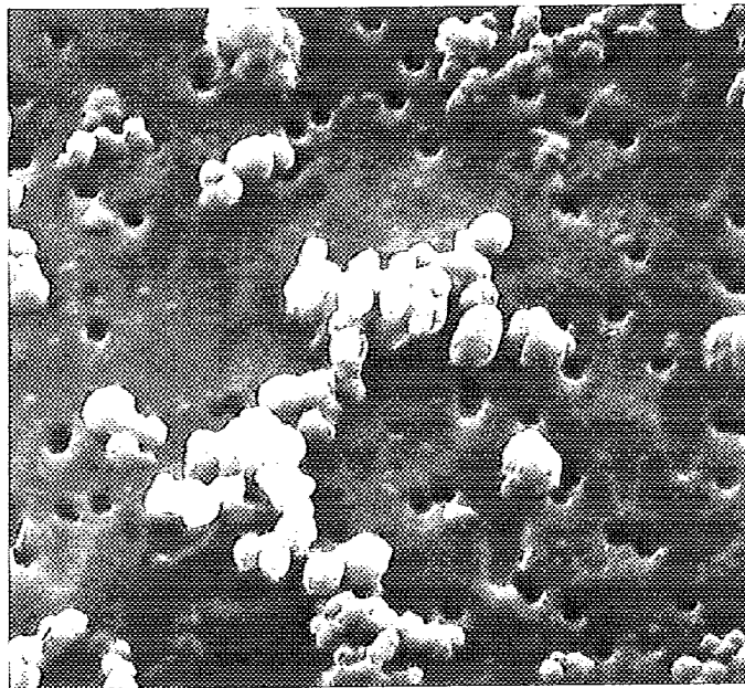
Fig. 1c — E7018 fume (20,000X)
