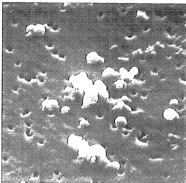
Fig. 1a — E6010 fume (20,000X)
