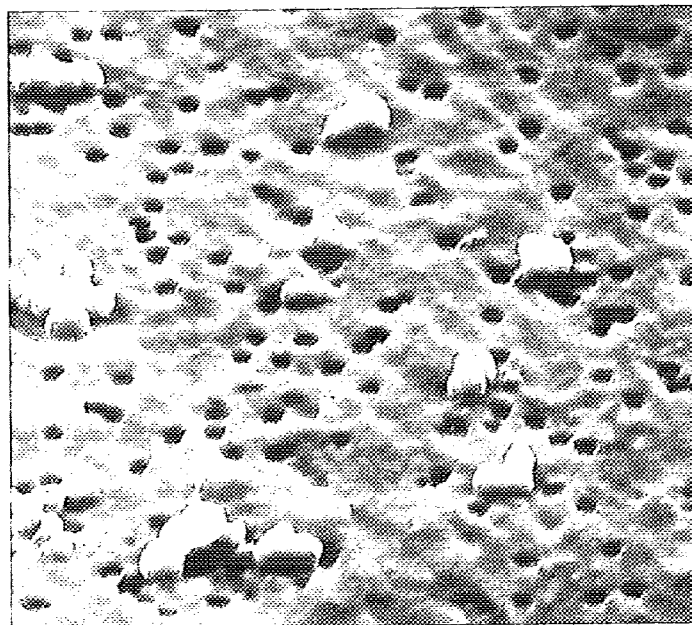
Fig. 1d — E70S-3 fume (20,000X)
