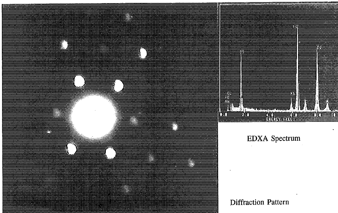
Fig. 9 — STEM Microanalysis for the E6010 fume
