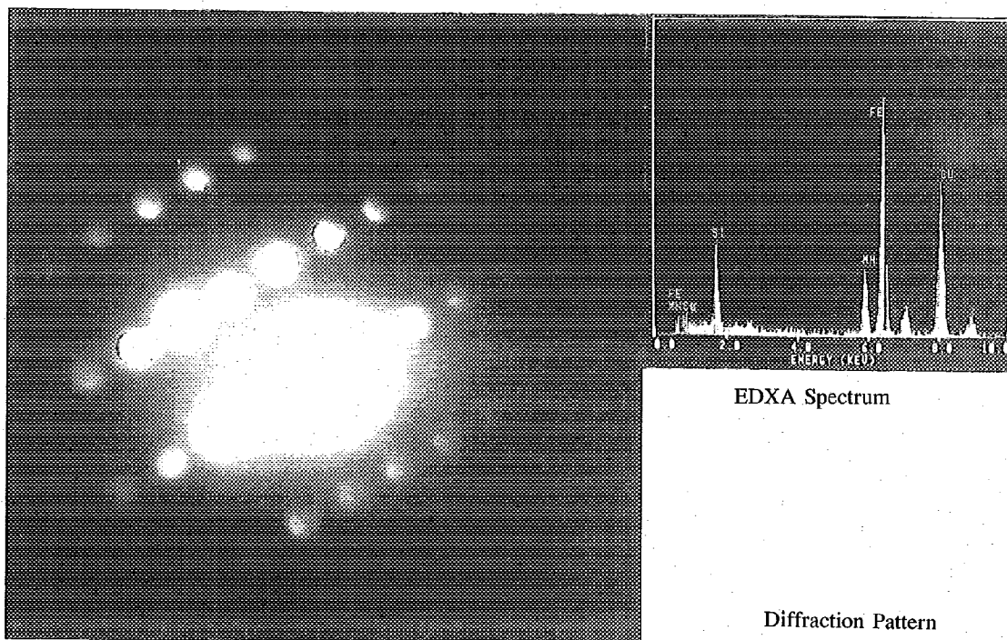
Fig. 11 — STEM Microanalysis for the E70S-3 fume
