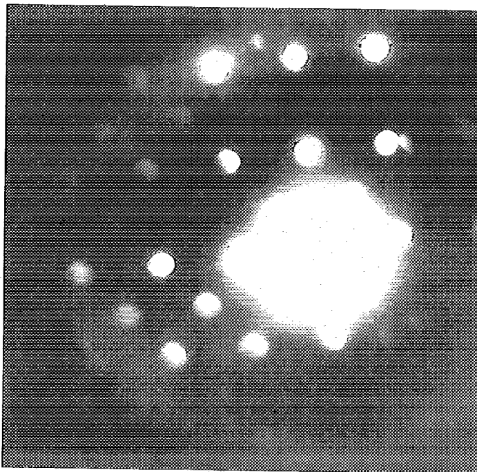
Fig. 14 — STEM Microanalysis for the E5356 fume
