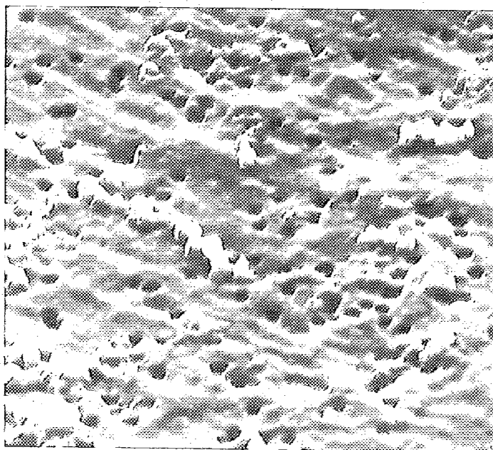
Fig. 1f — E308-16 fume (20,000X)
