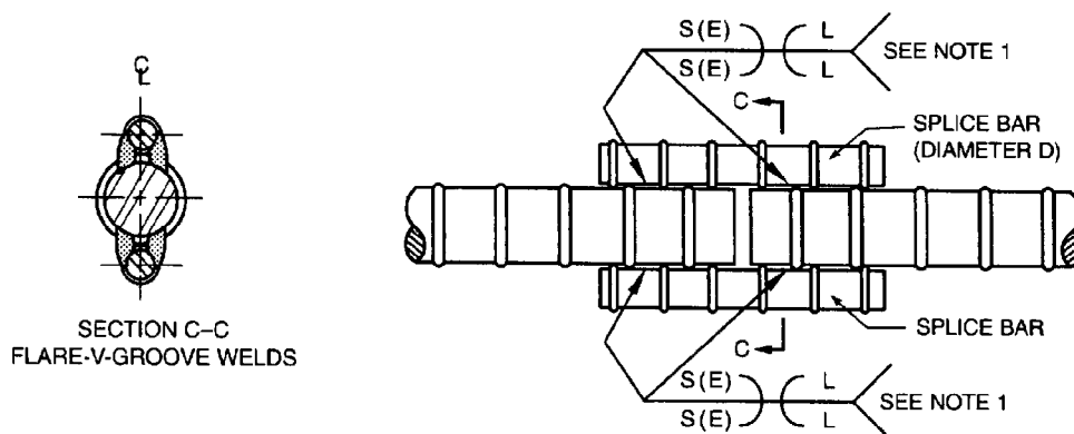
(C) INDIRECT BUTT JOINT TWO SPLICE BARS
