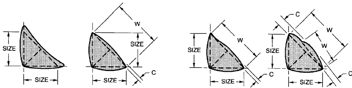
(A) DESIRABLE FILLET WELD PROFILES
