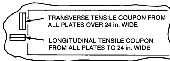
Figure D-2—Tensile Coupon Sampling
