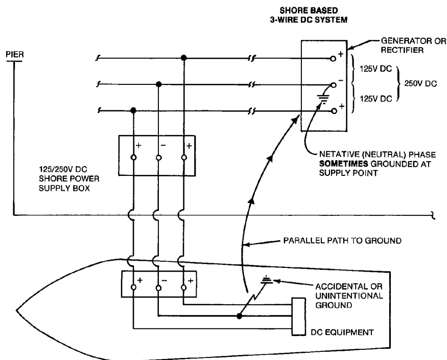
Figure 52—Potential Source of Direct Currents Causing Corrosion Due to Accidental or Unintentional Ground on Vessel
