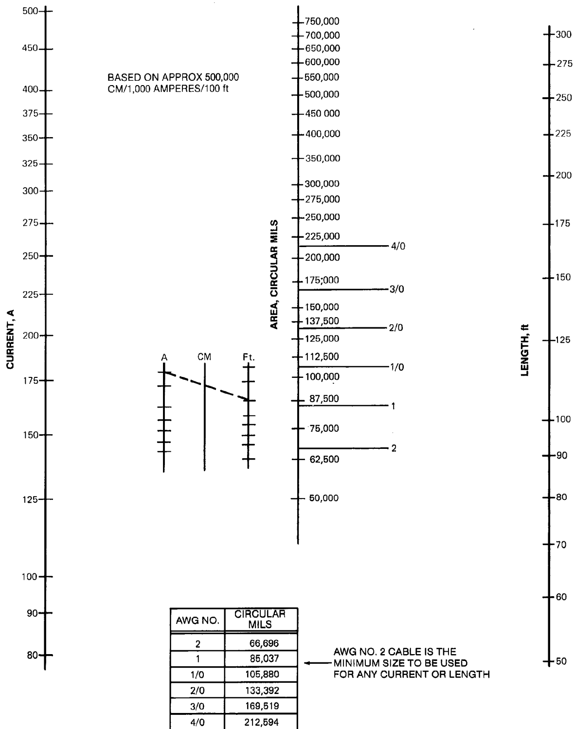
Figure 55—Nomograph for Copper Electrode Lead Cable Size
