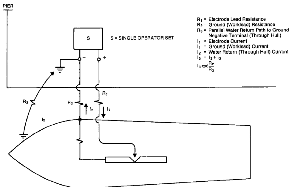
Figure 53—Equivalent Circuit for Improperly Connected Generator or Rectifier
