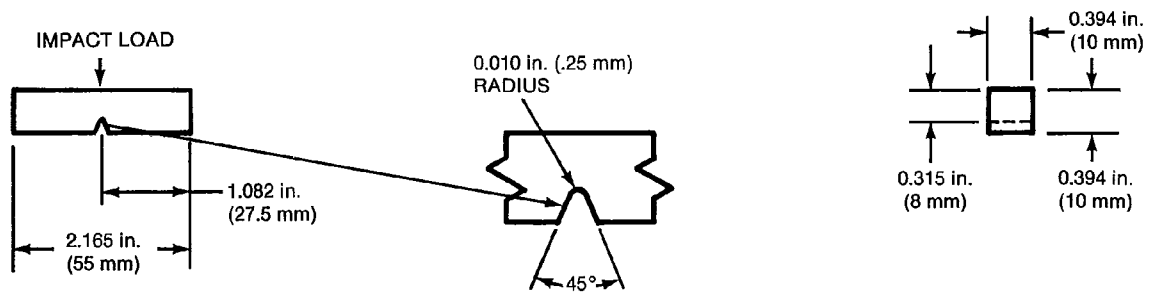
Figure 2A—Standard Charpy V-Notch Test Specimen
