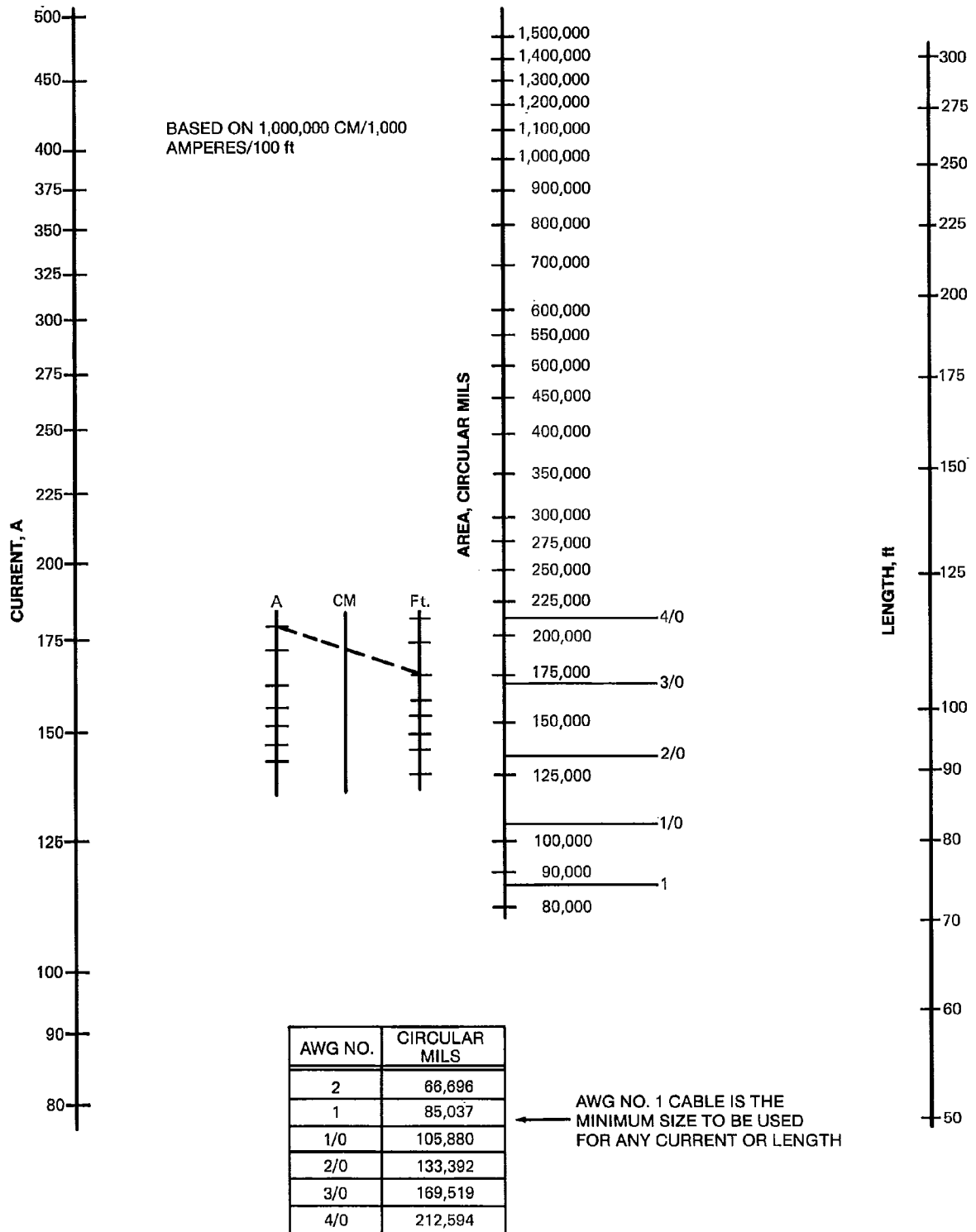
Figure 54—Nomograph for Copper Ground (Work Lead) Wire Size
