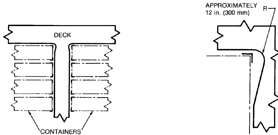
Figure 17—Typical Hatch Corner in Way of Container Guides on Container Ship
