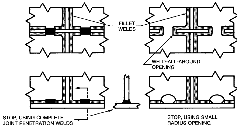
Figure 25—Welded Water- or Oil-Stops at Intersecting Members
