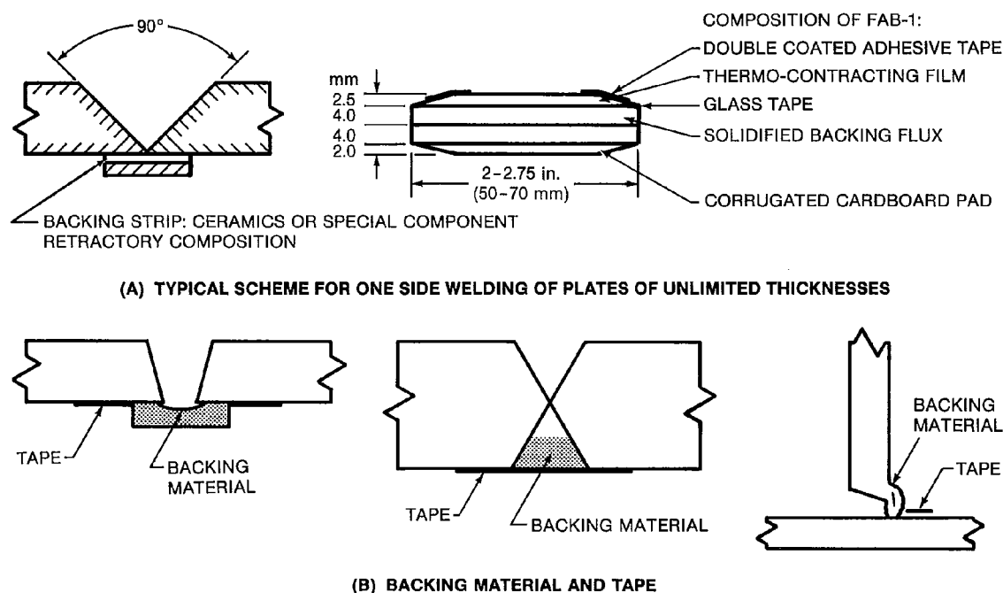
Figure 11—Typical Joint Details for One-Side Welding
