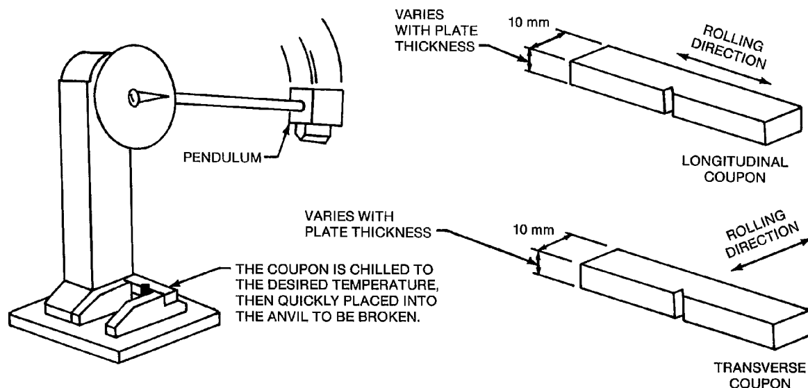
Figure D-5—Charpy Coupon Testing
