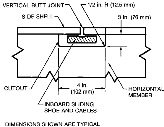
Figure 30—Cutout of Member to Permit Passage of Inboard Sliding Shoe and Cables
