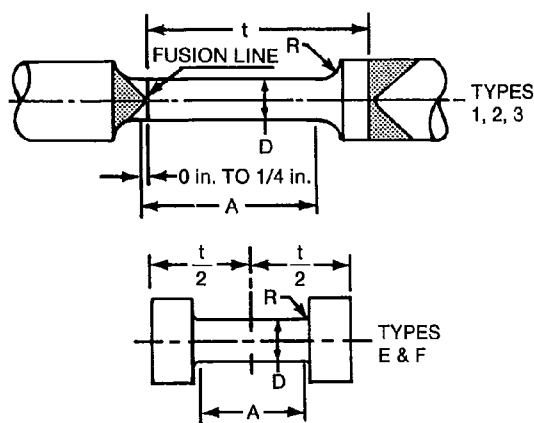
Figure D-8—ASTM A770 Through Thickness Tensile Coupons
