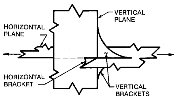
Figure 20—Stress Concentration at Intersecting Planes Eased by Brackets
