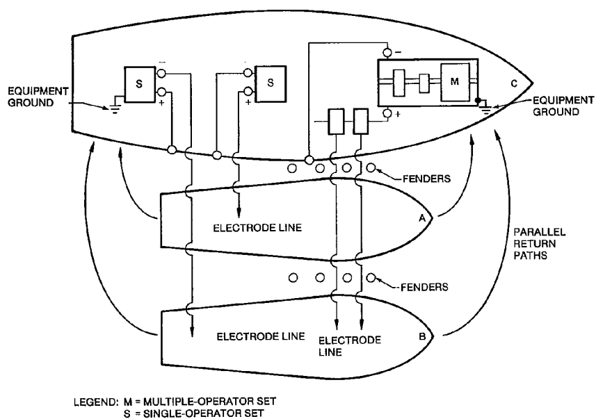
Figure 58—Hookup for Ships Afloat (Sheet 1 of 2 Sheets)
