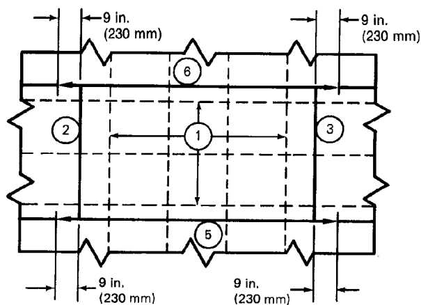
Figure 36—Typical Welding Sequence for Plate Butt and Adjacent Seams Where Internal Framing is Attached
