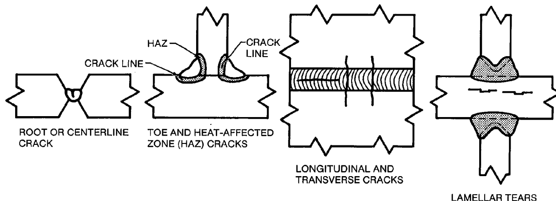
Figure 49—Typical Weldment Cracks
