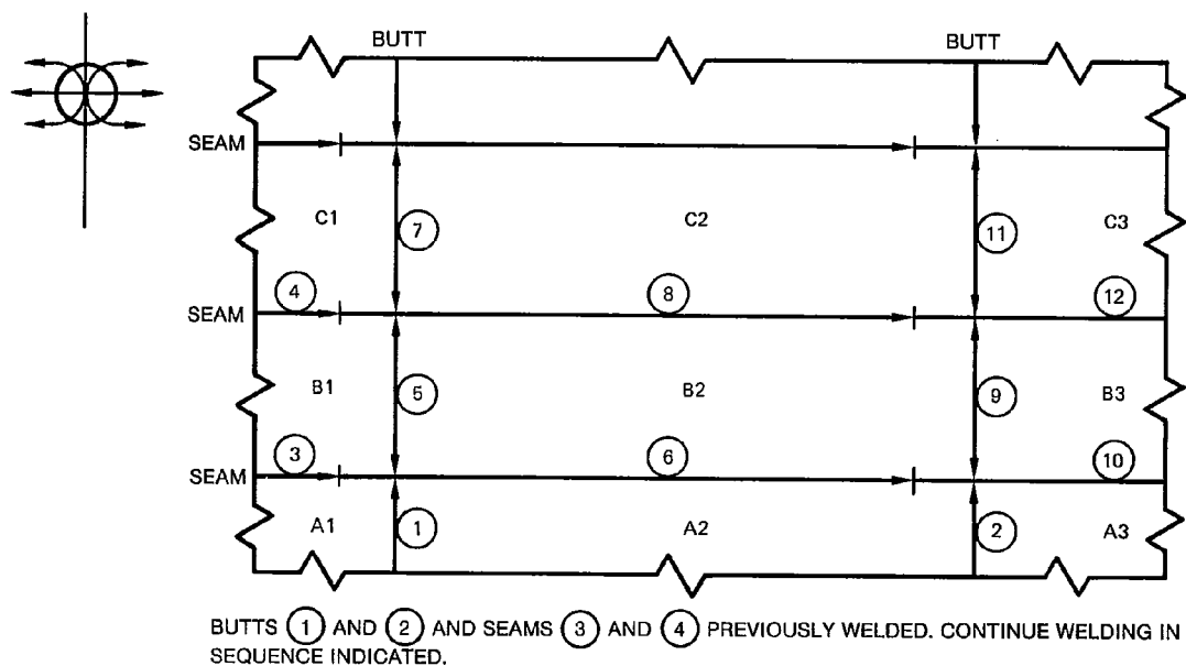
Figure 35—Typical Welding Sequence for Plate Butts and Seams Where Butts are in Line
