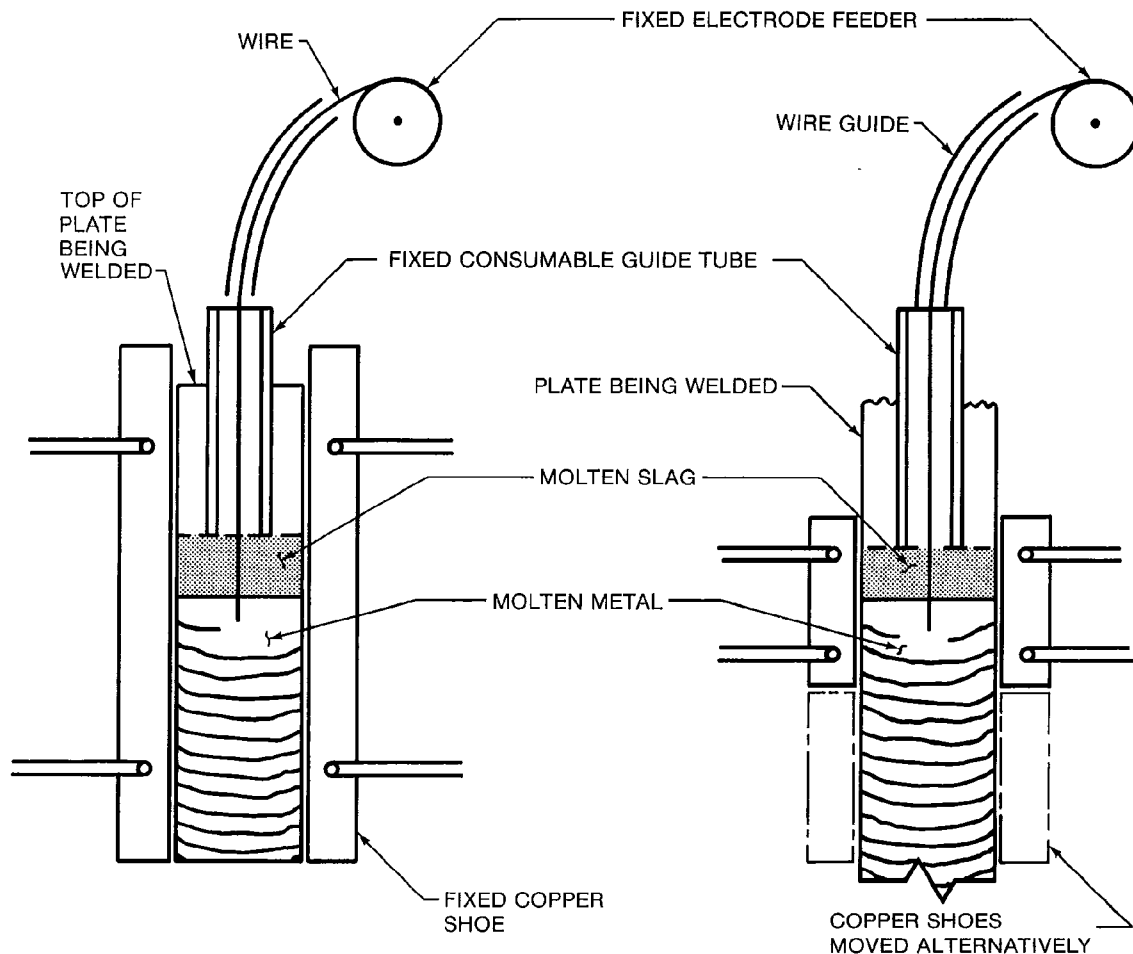
Figure 10—Consumable Guide Tube Welding
