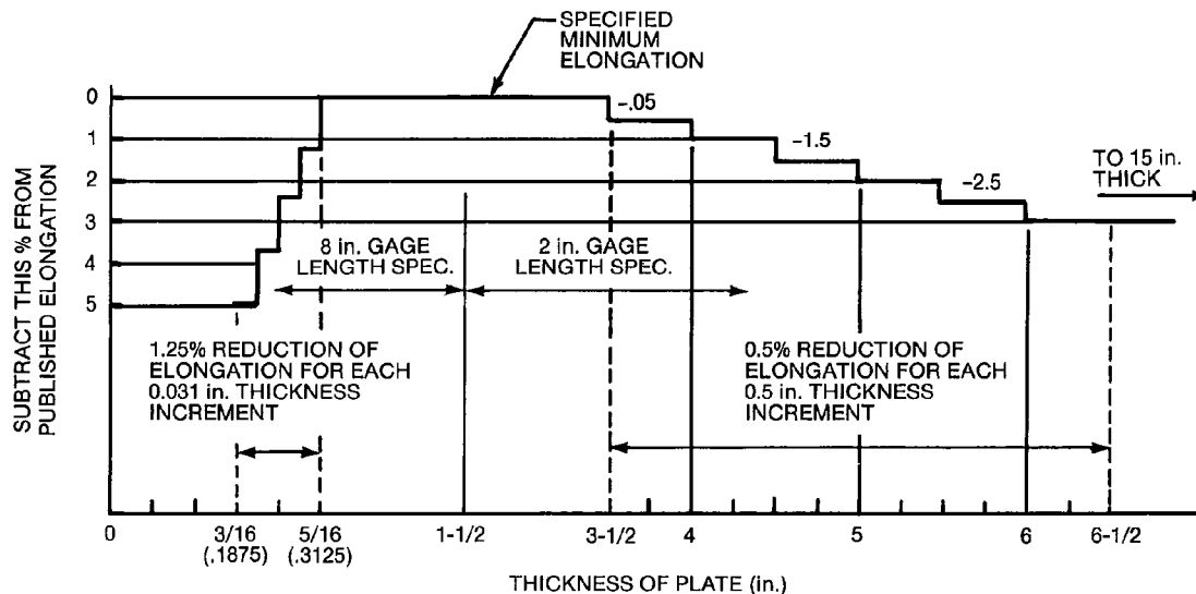
Figure D-4—Allowable Reduction in Tensile Coupon Elongation if Coupon Thickness is Less Than 5/16 Inch or More Than 3-1/2 Inch
