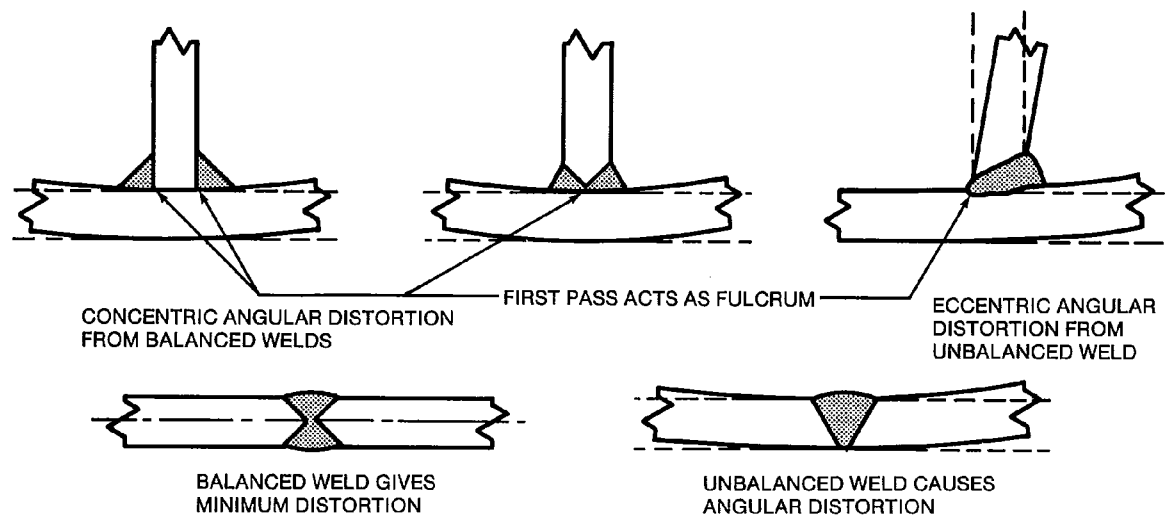
Figure 41—Typical Distortion of Welded Joints
