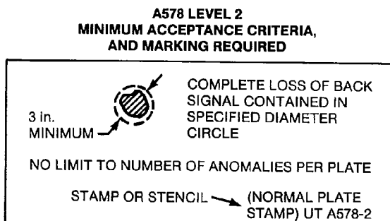
Figure D-10—A578 Minimum Acceptance Criteria and Marking Requirement
