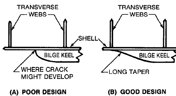
Figure 19—Bilge Keel Endings
