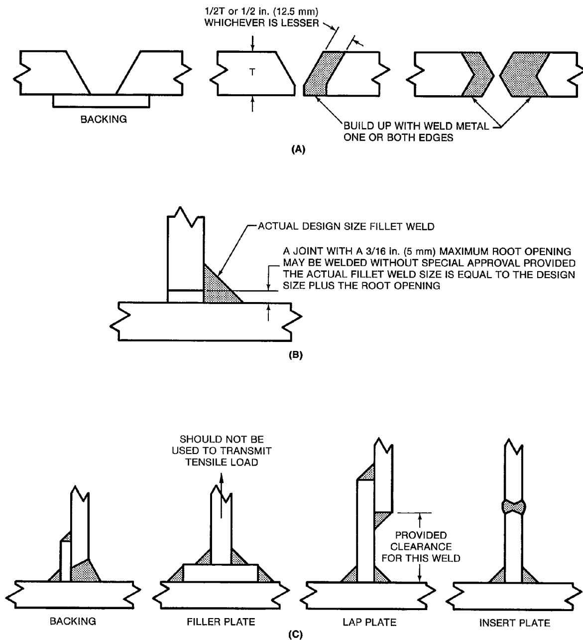
Figure 31—Correction of Poor Fit-Up
