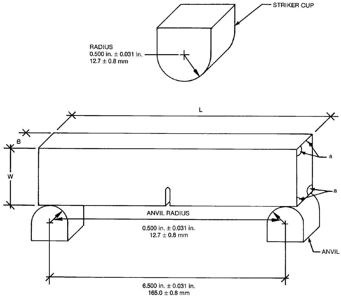
DIMENSIONS AND TOLERANCE FOR SPECIMEN BLANK
