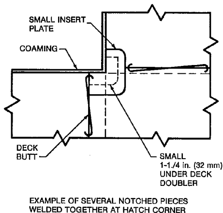
Figure 15—Original Design of Hatch Corner on Liberty Ship
