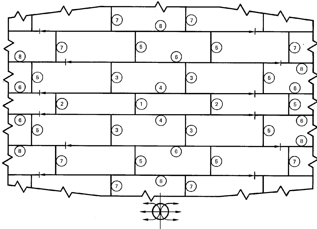
Figure 34—Typical Welding Sequence For Plate Butts and Seams Where Butts are Staggered
