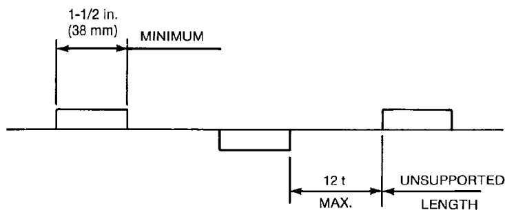
Figure 46—Control of Distortion in Thin Plate By Intermittent Welding
