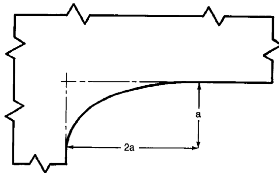
Figure 17—Typical Hatch Corner in Way of Container Guides on Container Ship
