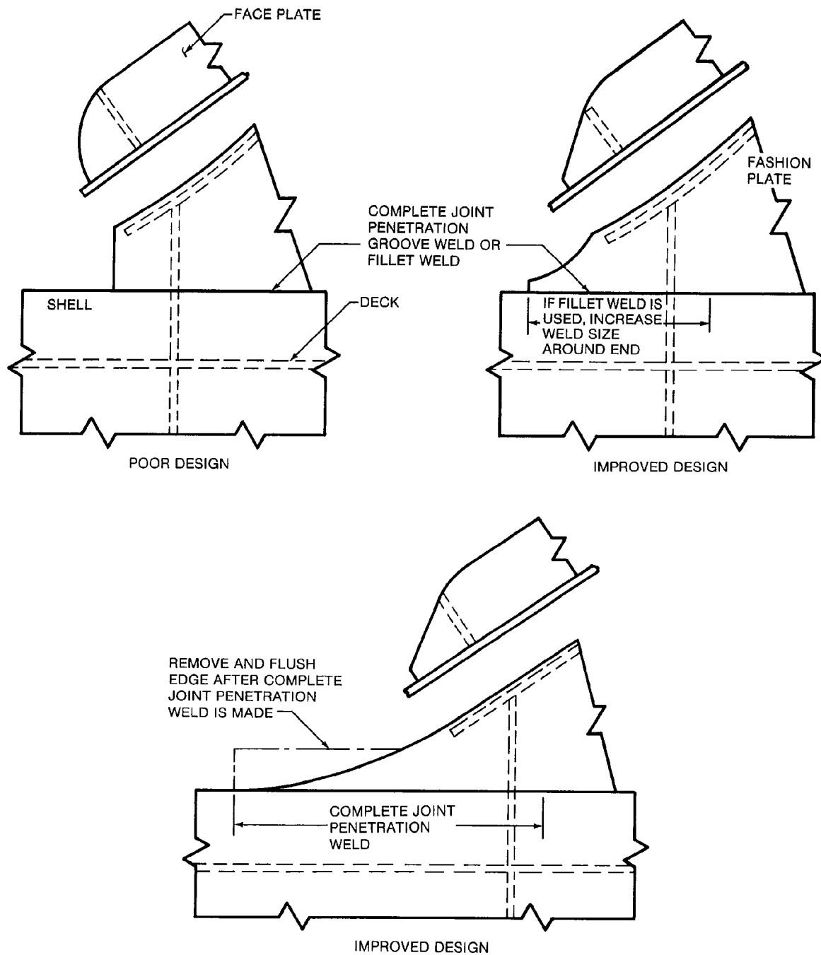
Figure 14—Ending of Bulwark Fashion Plate Welded to Top of Sheerstrake
