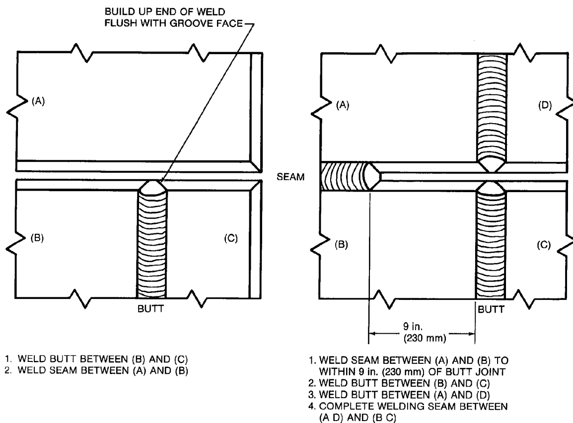
Figure 32—Welding Sequence at Intersection of Butt and Seam
