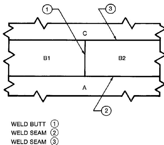
Figure 33—Welding Sequence for Plate Butt and Adjacent Seams
