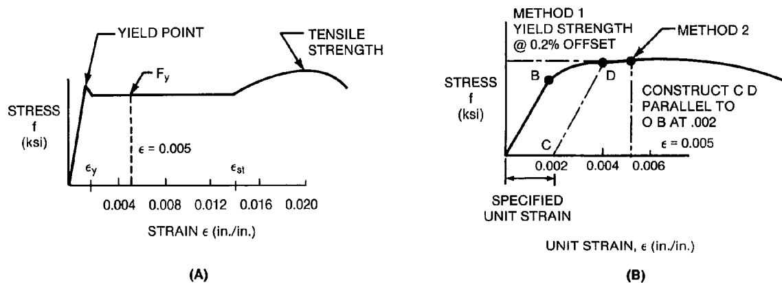
Figure D-3—Yield Stress Defined
