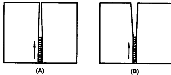
Figure 43—Angular Distortion Tendencies in Making Groove Welds
