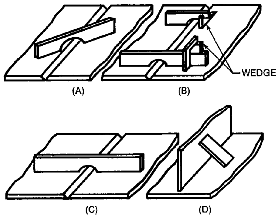
Figure 29—Typical Strongbacks
