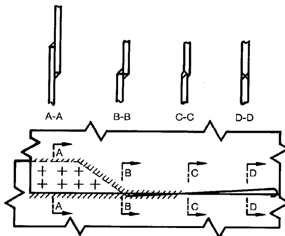
Figure 24—Transition From Riveting to Welding in Lap Seam
