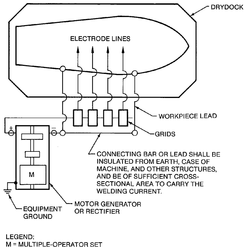
Figure 61—Hookup for Ships in Dry or Graving Dock
