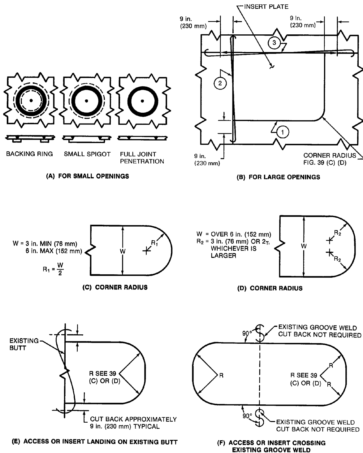
Figure 39—Closure of Small and Large Openings
