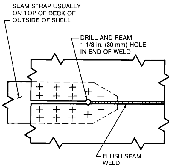
Figure 23—Transition From Riveting to Welding in Flush Seam
