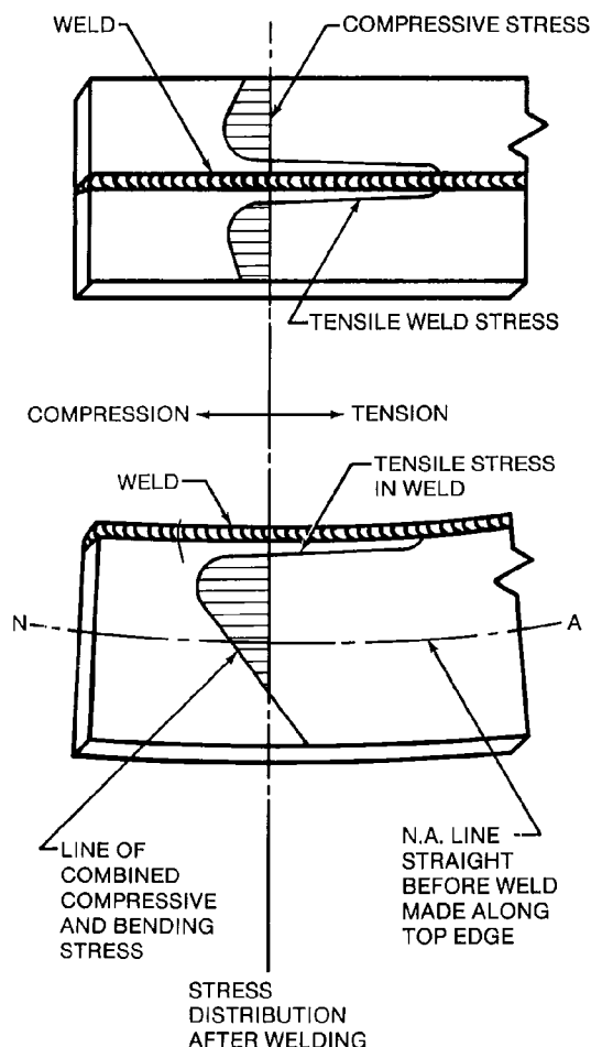
Figure 40—Residual Welding Stresses
