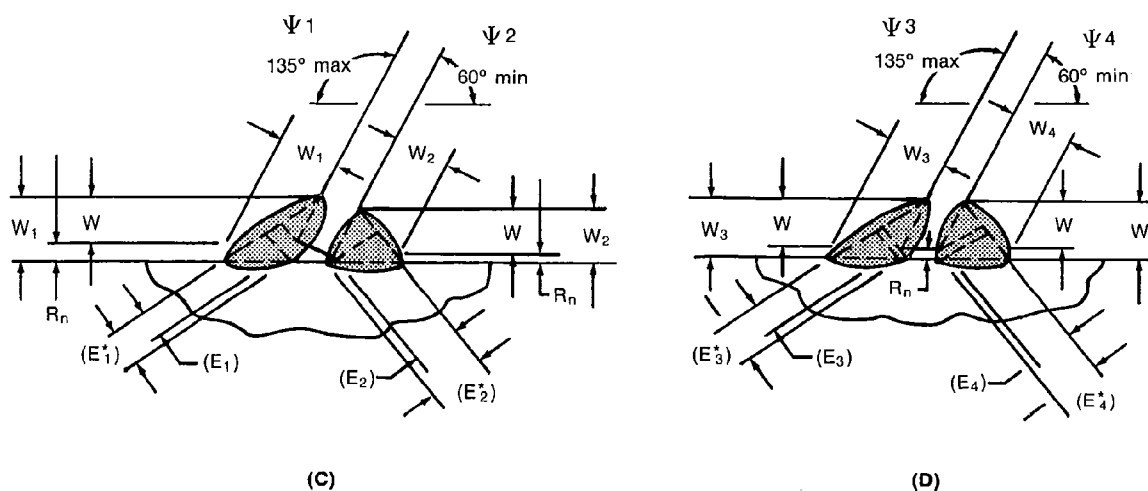
SKEWED T-JOINTS
