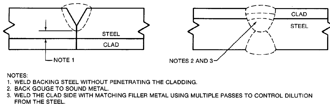
Figure 5—Typical Detail for Groove Welding Clad Plating
