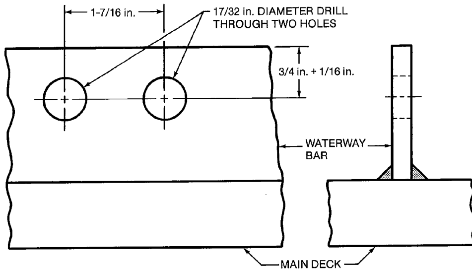
TYPICAL HOLE SPACING, GROUNDING LUG ATTACHMENT
