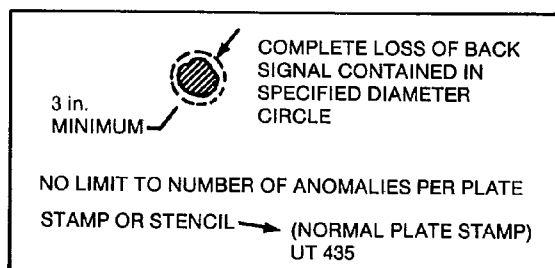
Figure D-9—UT A435 Minimum Acceptance Criteria and Marking Requirement
