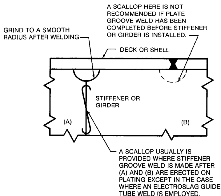
Figure 27—Scallops
