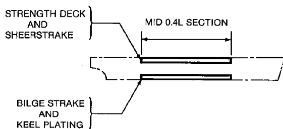
Figure 12—Most Highly Stressed Areas of Hull Girder
