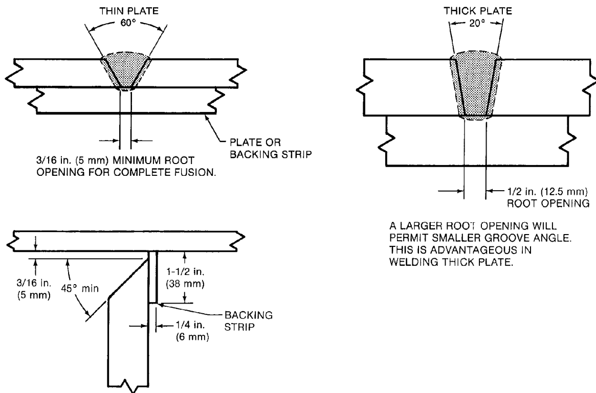
Figure 21—Typical Weld Details for Welding From One Side Only, Permanent Backing
