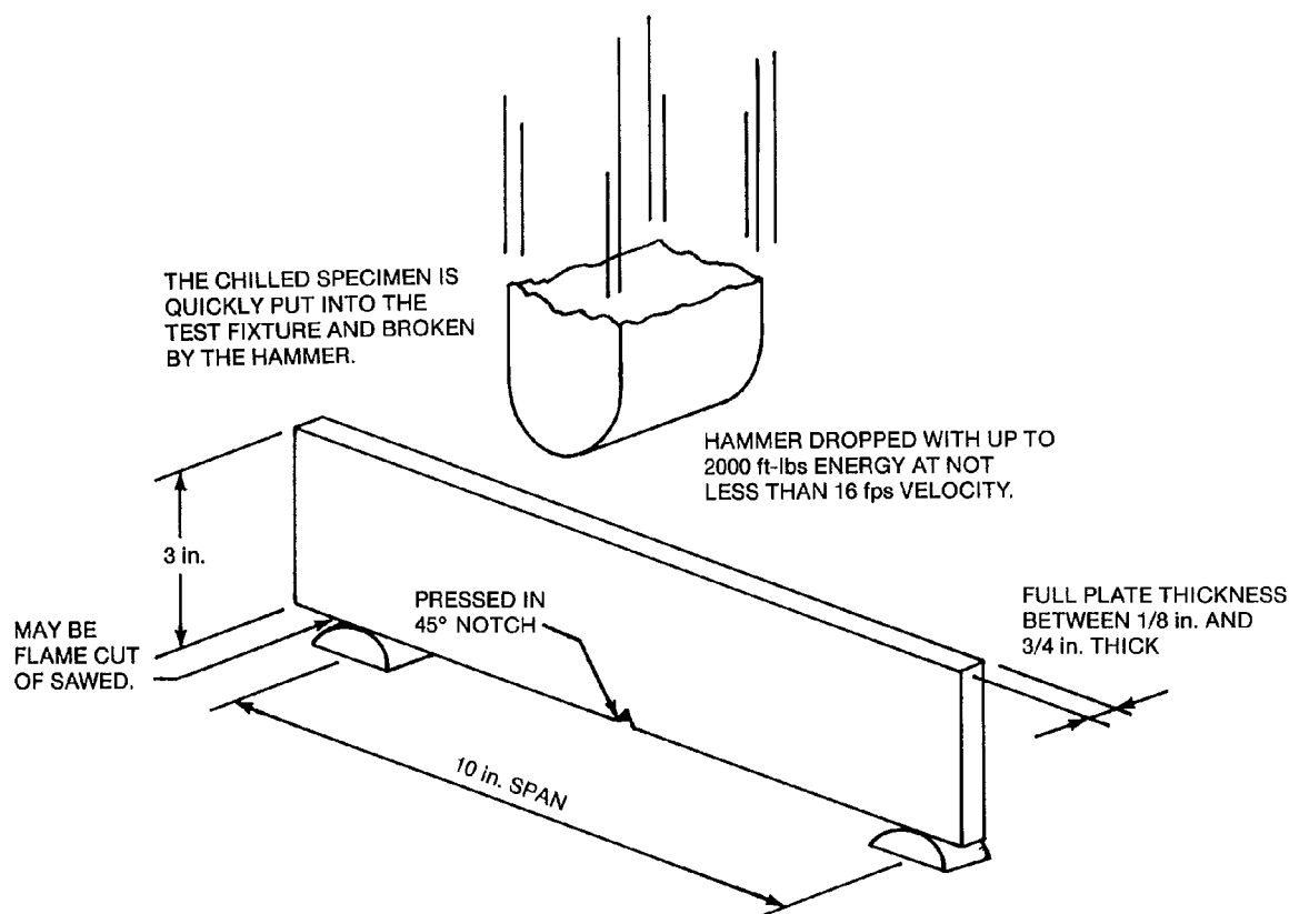
Figure D-7—Drop Weight Tear Test (ASTM E436)
